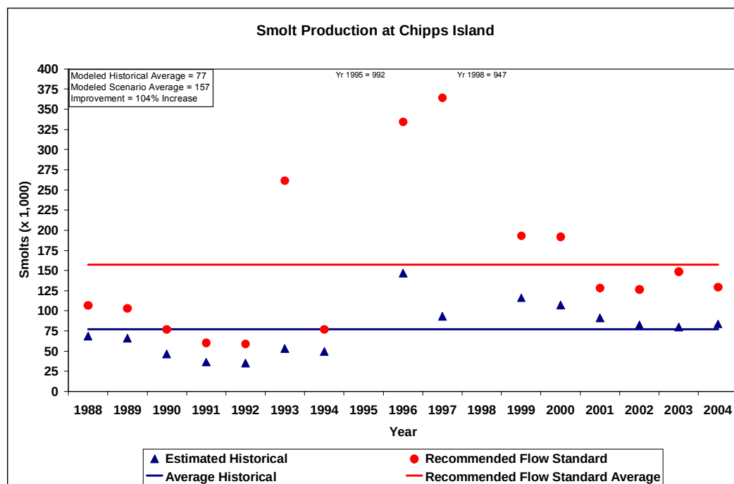
Figure 3: Modeled Chipps Island Salmon Production for Years 1988-2004.
