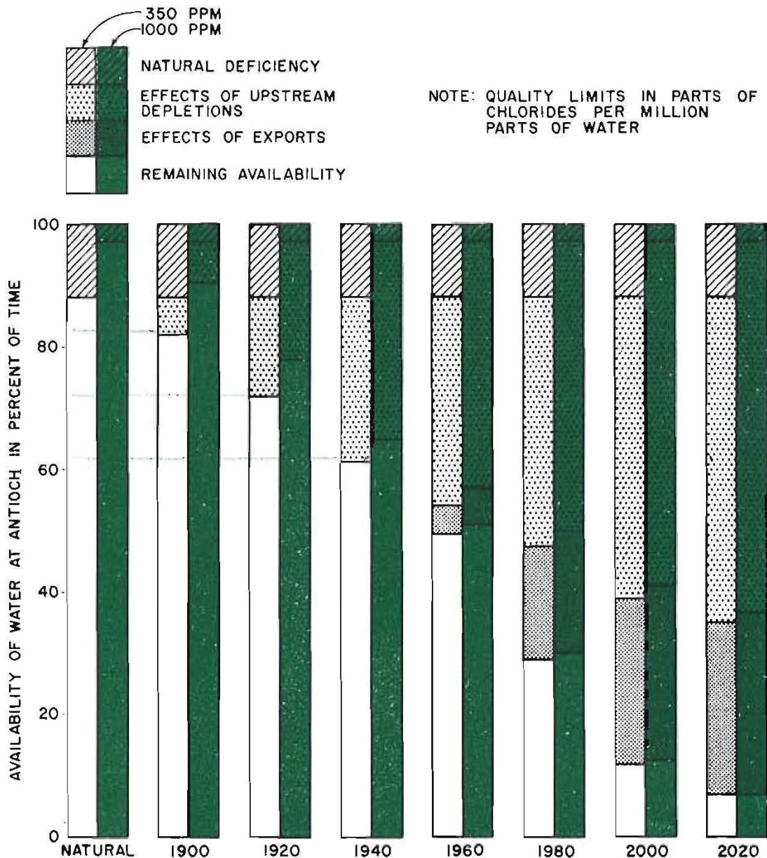
Figure A-4 - Salinity on the San Joaquin River at Antioch (DWR, 1960)
