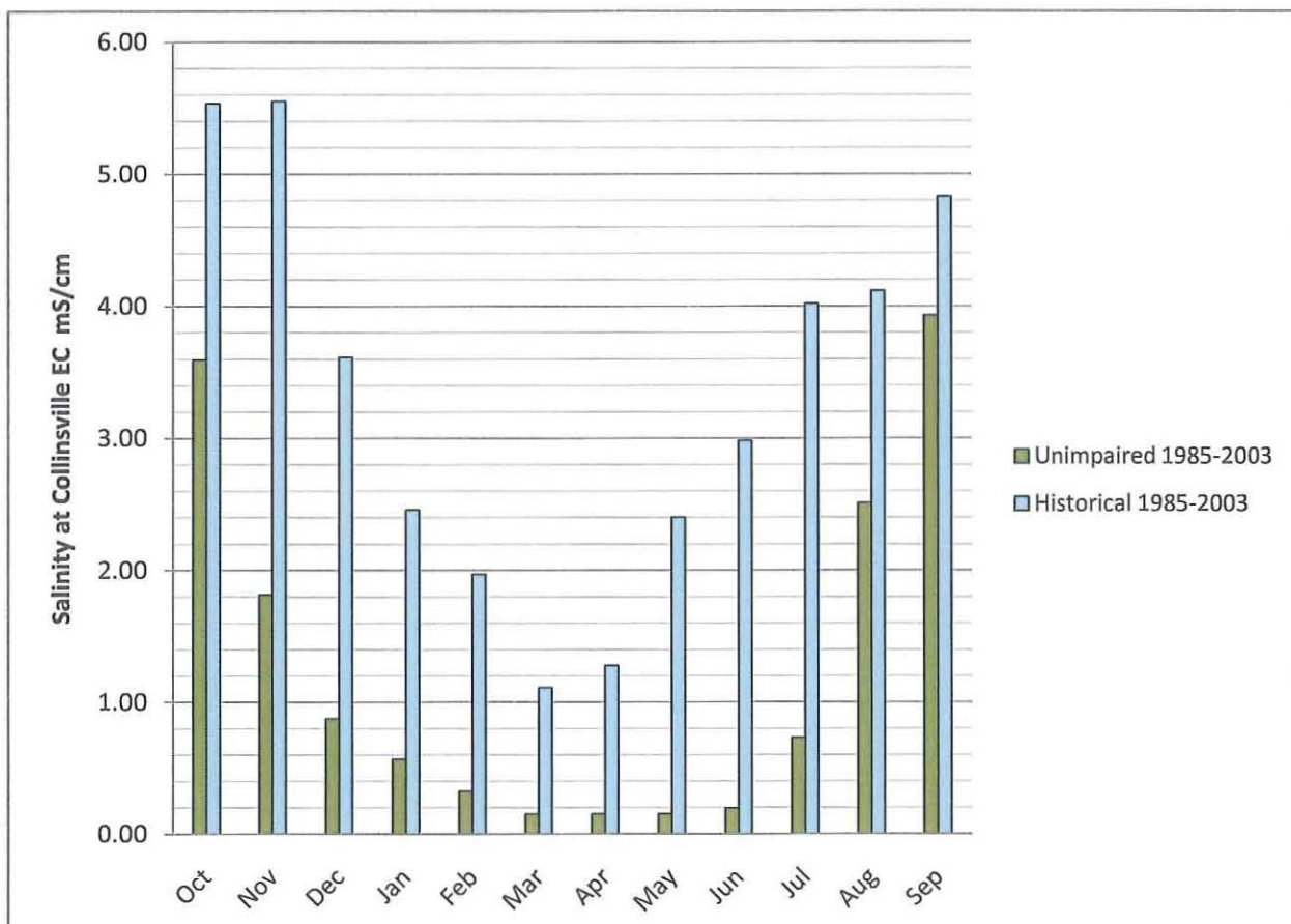
Figure 2 Historical and Unimpaired Salinity at Collinsville. Unimpaired salinity was calculated using unimpaired NDO and the G-model. Note that measured salinities are consistently greater than unimpaired.
