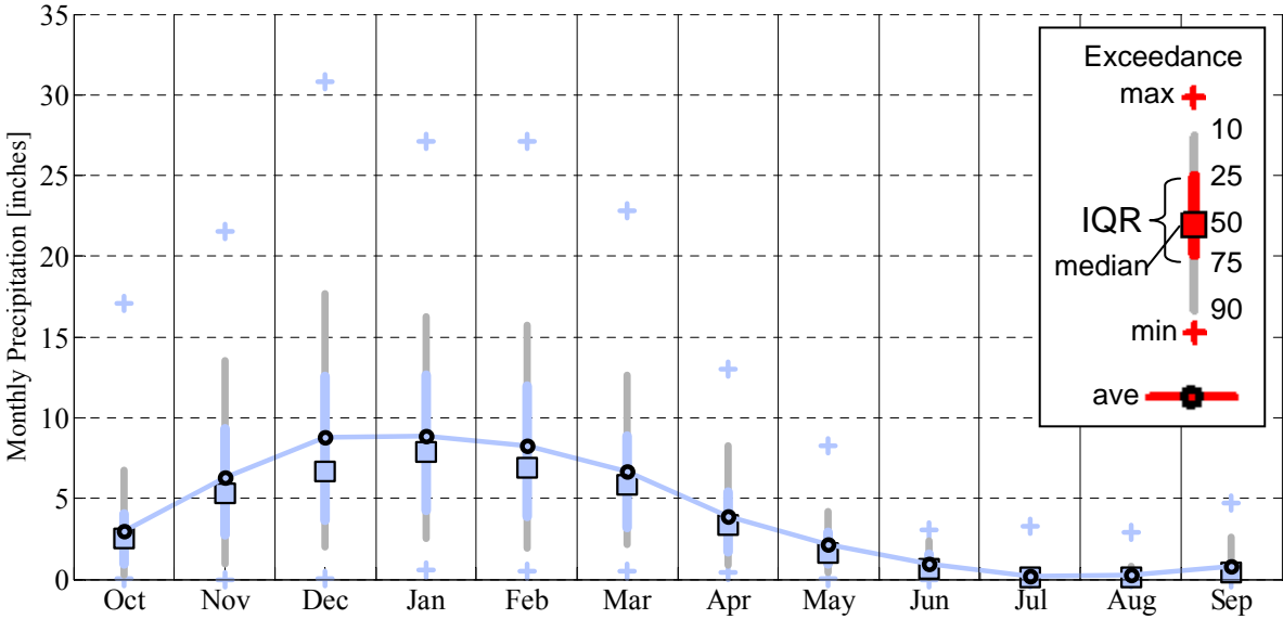
Figure 3-3 – Monthly Distribution of Precipitation in the Sacramento River Basin
