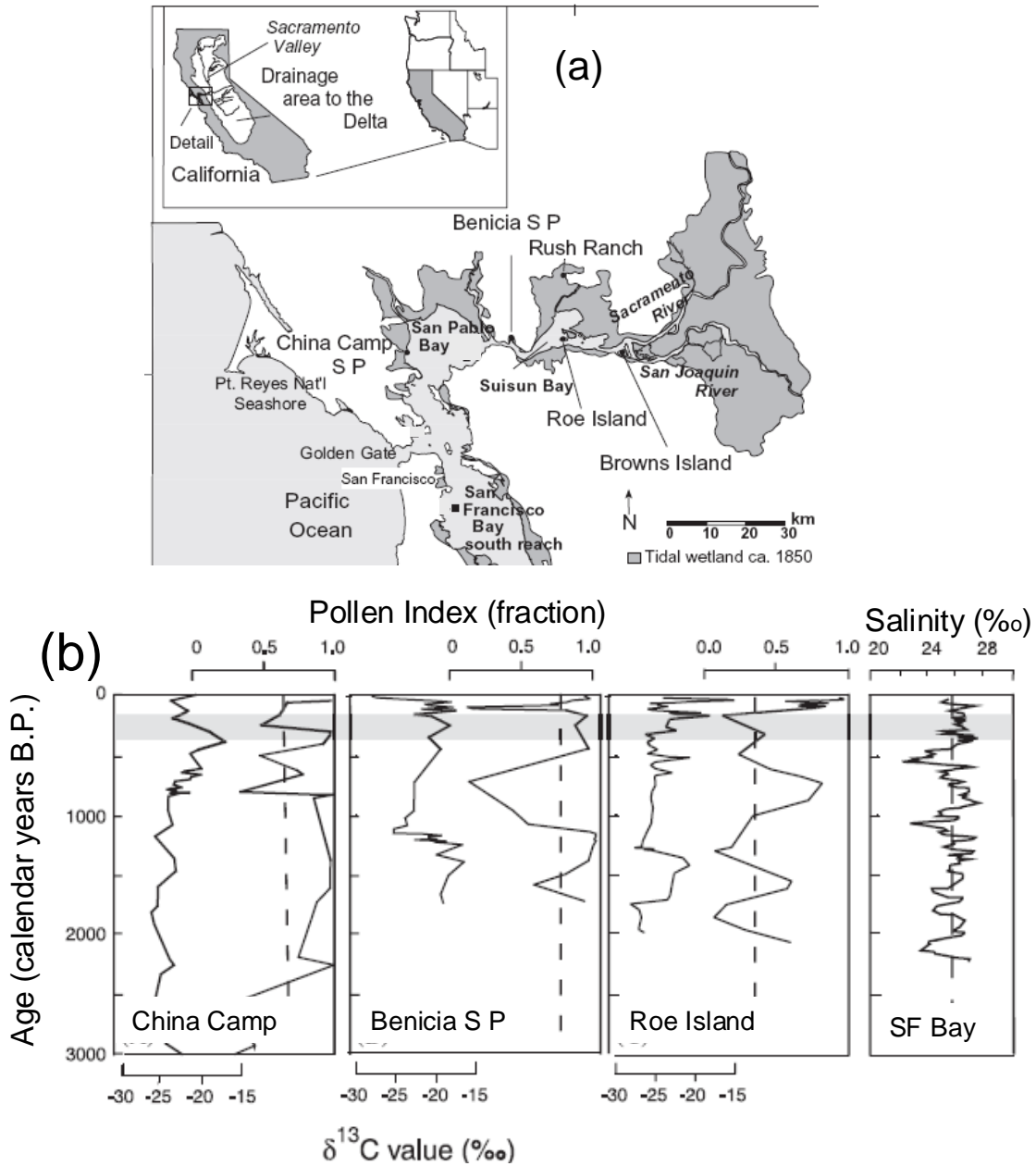
Figure B-2 – Paleosalinity records at selected sites in the San Francisco Estuary (a) location of the three tidal marsh sites (China Camp, Benicia State Park and Roe Island) and one site in the Estuary (Oyster Point in San Francisco Bay) where sediment cores were obtained. (b) time series for the pollen index (ranging from 0 to 1, higher values corresponding to higher salinity) and the \delta^{13}C values at the tidal marsh sites; salinity at Oyster Point, San Francisco Bay (inferred from \delta^{13}O values) is also shown. The broken line shows the estimated mean pollen index prior to European disturbance. (modified from Malamud-Roam and Ingram (2004) and Malamud-Roam et al. (2006))
