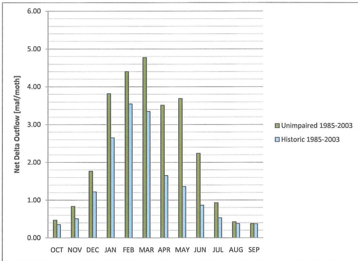
Figure 1 Historical and Unimpaired Net Delta Outflow from 1985-2003. Note that measured NDO is always less than unimpaired.
