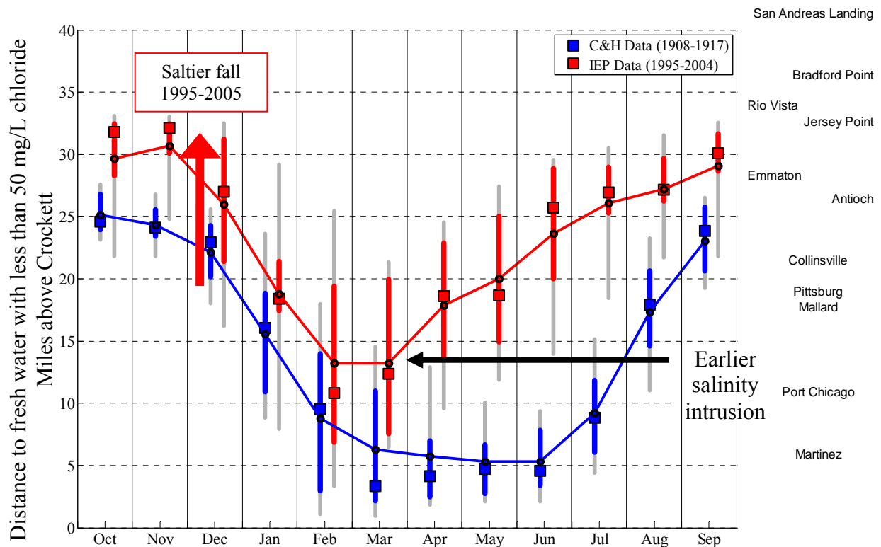
Figure 3-10 – Monthly distribution of distance to fresh water from Crockett
