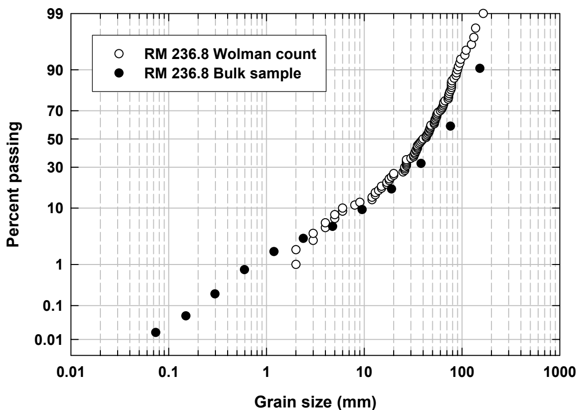
Appendix Figure COMP5. Grain-size distributions of the surface inferred from a Wolman count (open symbols) and a bulk sample (closed symbols) for a site on the Sacramento River in 2005. The Y axis shows a probability scale.
