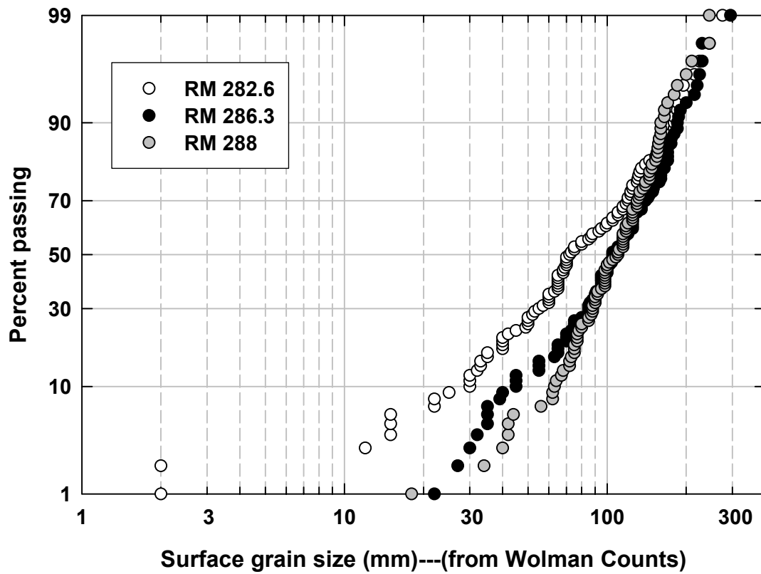
Appendix Figure WC5. Grain-size distributions of the surface inferred from Wolman Counts at 3 locations on the Sacramento River in 2005. The Y axis shows a probability scale.
