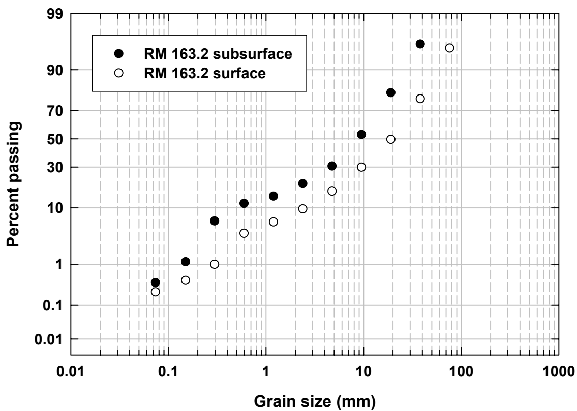
Appendix Figure BS9. Grain-size distribution from bulk sampling at RM 163.2 in 2005. Y axis is a probability scale.
