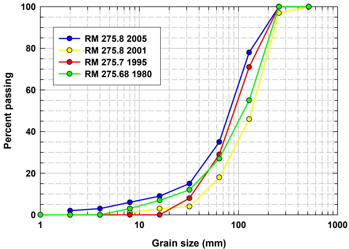
Figure 32. Time series of grain-size distributions from Wolman counts for a location on the upper river. Here, the grain-size measurements from 2005 are binned in "phi"-scale size classes for consistency with previous data. Data suggest the site became finer from 1980 to 1995, then significantly coarser by 2001, and was finer than ever by 2005.
