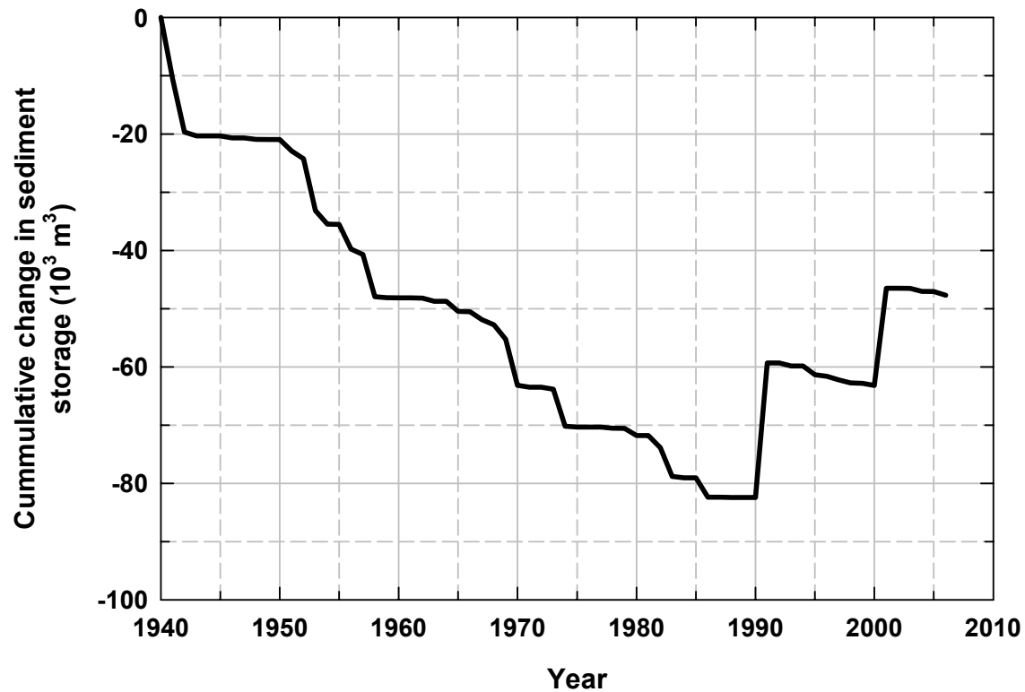
Figure 53. Simulated cumulative change in in-stream sediment storage in reach 3 (RM 295-290) in the post-dam era. After a sharp initial decline in sediment storage (due to the cessation of sediment supply from upstream sources), continued decreases in sediment storage were more progressive, and occurred in years with high flows. Gravel augmentation in 1990 and again in 2000 led to substantial one-time increases in sediment storage in the reach.
