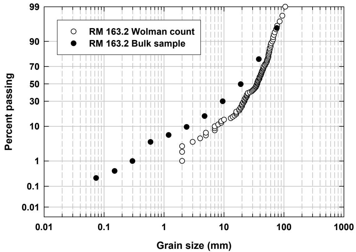
Appendix Figure COMP9. Grain-size distributions of the surface inferred from a Wolman count (open symbols) and a bulk sample (closed symbols) for a site on the Sacramento River in 2005. The Y axis shows a probability scale.
