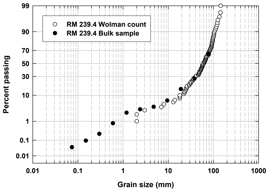
Appendix Figure COMP4. Grain-size distributions of the surface inferred from a Wolman count (open symbols) and a bulk sample (closed symbols) for a site on the Sacramento River in 2005. The Y axis shows a probability scale.
