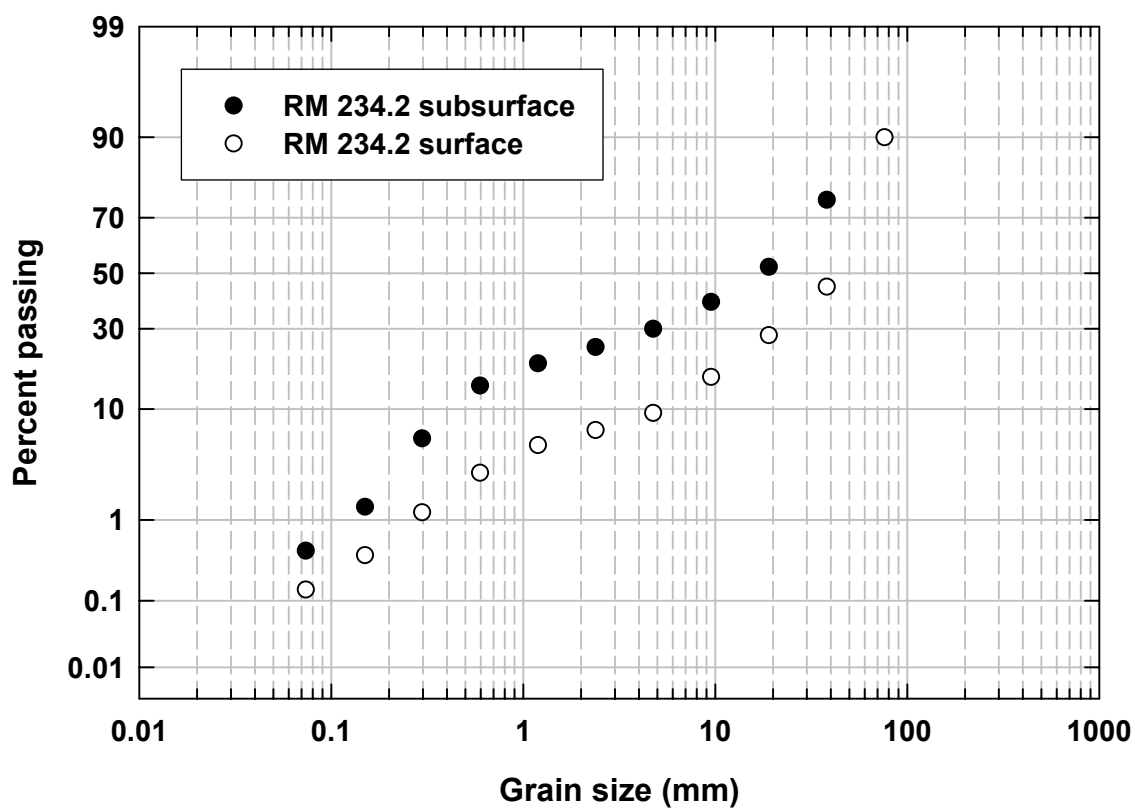
Appendix Figure BS6. Grain-size distribution from bulk sampling at RM 234.2 in 2005. Y axis is a probability scale.
