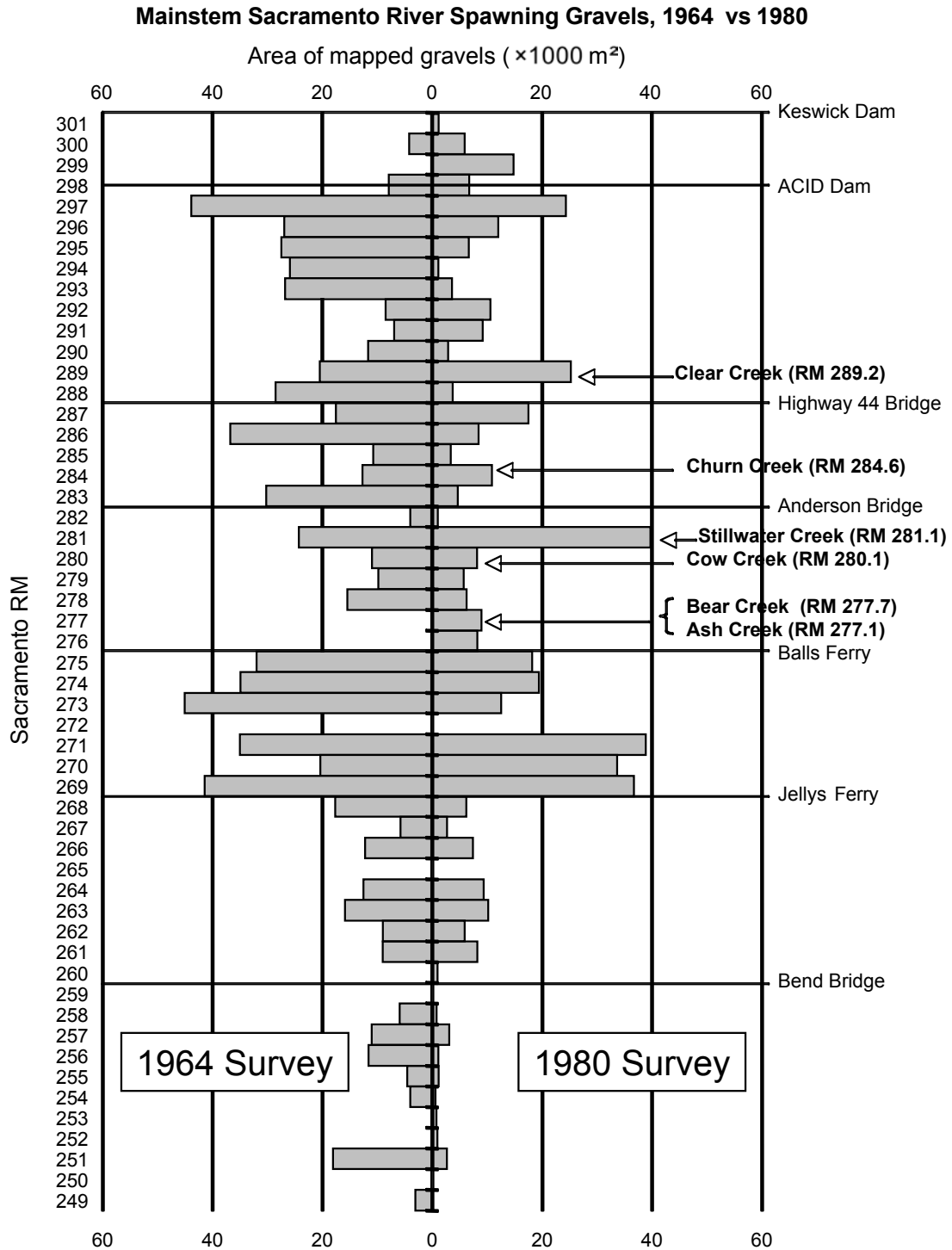
Figure 4. Local effects of small gravel additions. Several tributaries contribute small amounts of sediment to the mainstem channel, helping to maintain patches of spawning habitat near the confluence. However, the small sediment supply produces only local effects, having little impact on the maintenance of spawning habitat farther downstream. Gravel augmentation may create a similar pattern, helping to maintain existing habitat near the injection site, but doing little to expand spawning habitat farther downstream.
