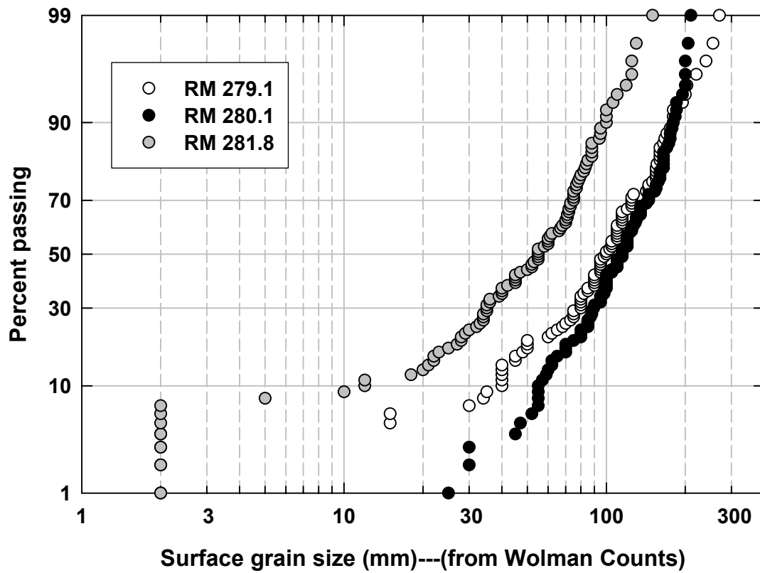
Appendix Figure WC6. Grain-size distributions of the surface inferred from Wolman Counts at 3 locations on the Sacramento River. The Y axis shows a probability scale.
