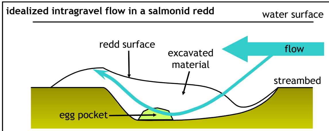
Figure 3. Conceptual diagram of intragravel flow through a buried salmonid egg pocket. The redd imposes a perturbation to the streambed profile, creating hydraulic conditions that force flow through the egg pocket.
