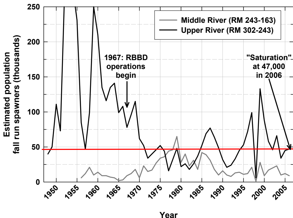
Figure 19. Estimated fall run spawning returns, Sacramento River mainstem. Source: CDFG (2007), except 1948-1956 data (from CDWR 1985; see Table 10). Field observations suggest that fall run returns in 2006 were sufficient to "saturate" available spawning area in the upper river (see text). This implies that the current threshold for saturation by fall run spawners is at least as low as 47,000 fish (red horizontal line). This implies that spawning area was probably saturated with fall run spawners in 2005 (during the helicopter survey) and further suggests that saturation may have occurred in 1964, when the estimated population in the upper river was 141,000 fish. Importantly, the 47,000 fish threshold does not rule out the chance that saturation occurred in 1980, even though only 22,000 fall run spawners returned to the upper river in that year; 47,000 is a minimum bound on the threshold (it could be lower). The late 1960's decline in upper river returns was accompanied by an increase in returns on the middle river, coincident with operation of RBBD, which would have impeded fall run access to the upper river, and thus forced a greater percentage of the run to spawn in the middle river.
