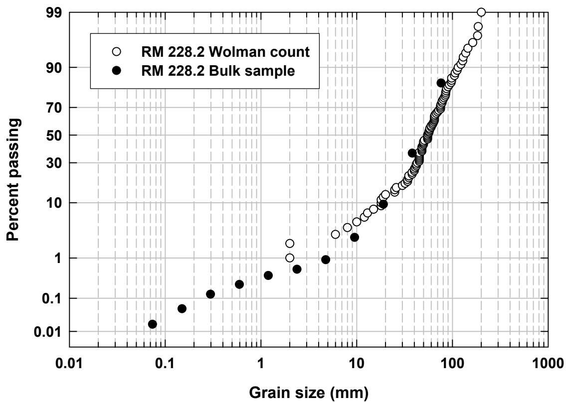
Appendix Figure COMP7. Grain-size distributions of the surface inferred from a Wolman count (open symbols) and a bulk sample (closed symbols) for a site on the Sacramento River in 2005. The Y axis shows a probability scale.
