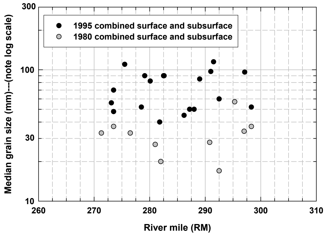
Figure 25. Median grain size (determined from bulk samples) as a function of river mile for heads of point bars (at riffles) in 1980 and 1995. A systematic offset seems to suggest that samples were coarser in 1995. But this conclusion is not actually supported by the data due to discrepancies in the sampling methods (see text). The differences in sampling methods can explain the observed pattern (apparently coarser samples in 1995) in the absence of an increase in grain size over time.
