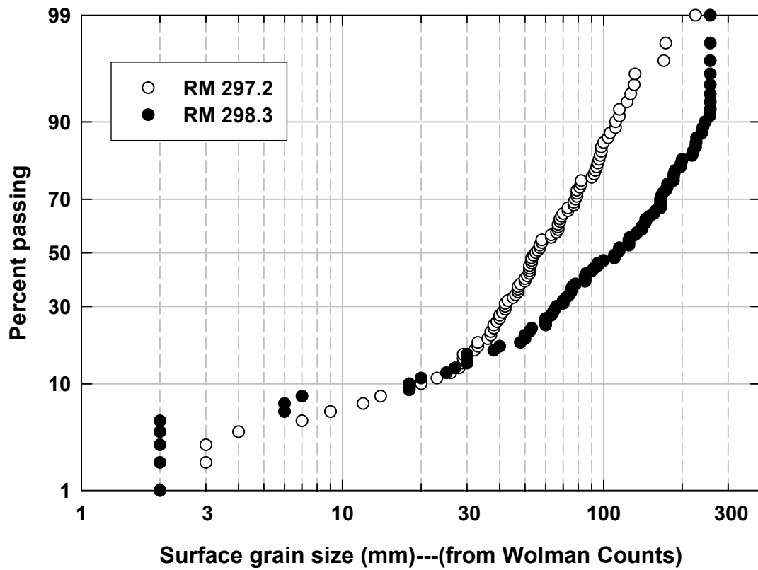
Appendix Figure WC1. Grain-size distributions of the surface inferred from Wolman Counts at 2 locations on the Sacramento River in 2005. The Y axis shows a probability scale.
