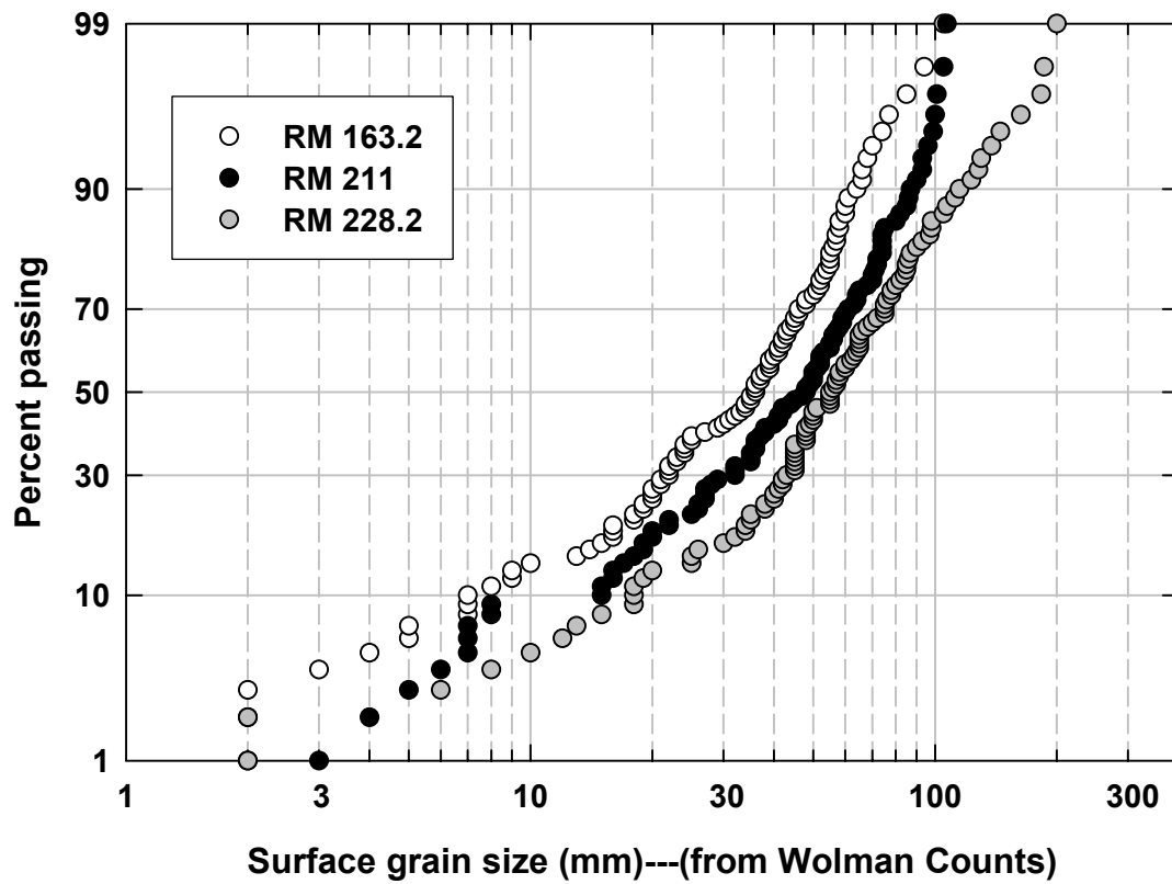
Appendix Figure WC10. Grain-size distributions of the surface inferred from Wolman Counts at 3 locations on the Sacramento River in 2005. The Y axis shows a probability scale.
