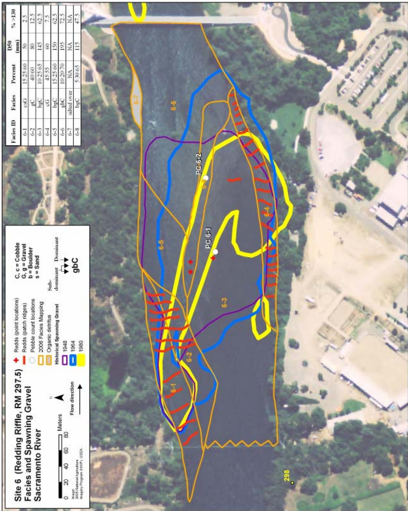
Figure 45. Facies map site 6 at RM 297.5.
