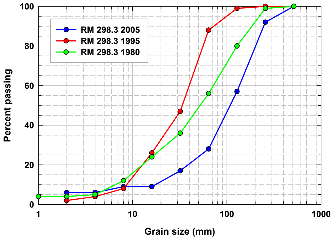
Figure 36. Time series of grain-size distributions from Wolman counts for a location on the upper river. Here, the grain-size measurements from 2005 are binned in "phi"-scale size classes for consistency with previous data. Data suggest the surface became finer by 1995 and then coarsened by 2005.
