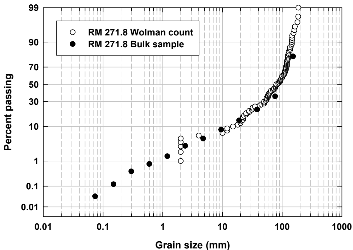
Appendix Figure COMP3. Grain-size distributions of the surface inferred from a Wolman count (open symbols) and a bulk sample (closed symbols) for a site on the Sacramento River in 2005. The Y axis shows a probability scale.
