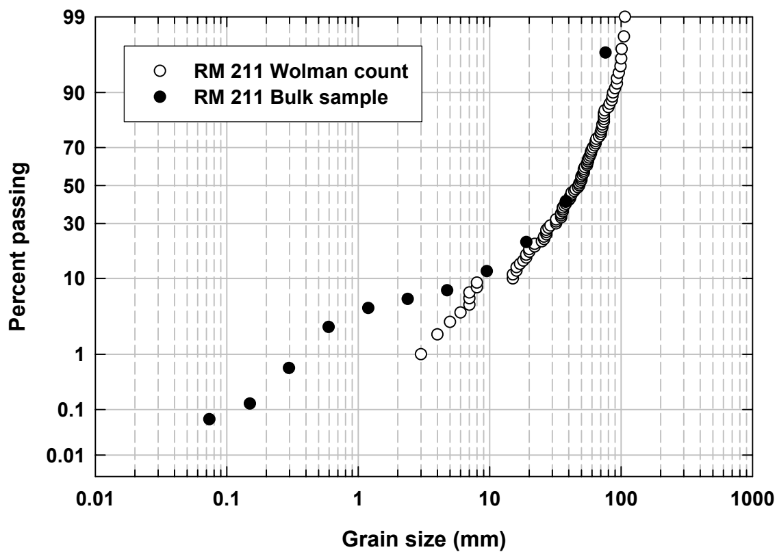
Appendix Figure COMP8. Grain-size distributions of the surface inferred from a Wolman count (open symbols) and a bulk sample (closed symbols) for a site on the Sacramento River in 2005. The Y axis shows a probability scale.
