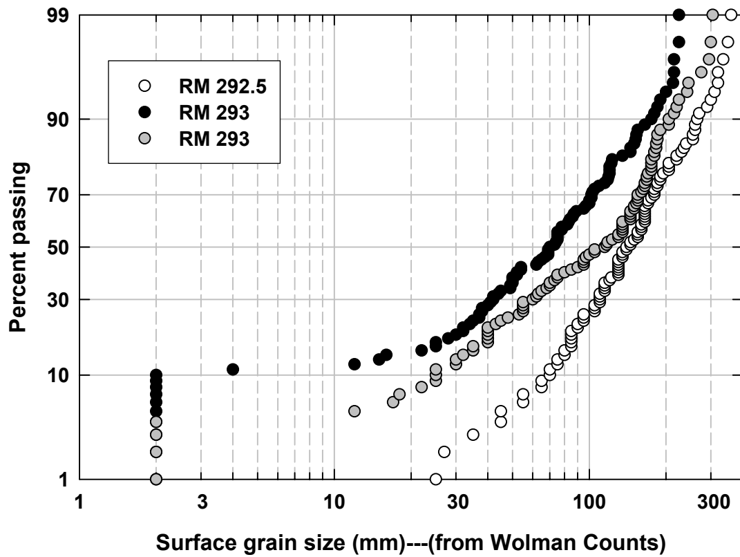
Figure 28. Grain-size distributions of the surface inferred from Wolman Counts at 3 locations on the Sacramento River in 2005. The Y axis shows a probability scale. Data show that grain size distributions vary substantially over the scale of a few hundred to one thousand meters.
