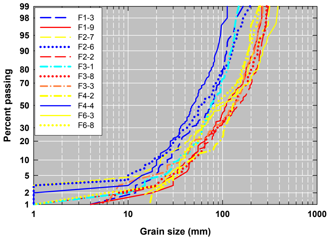
Figure 47. Grain-size distributions of the surface inferred from Wolman counts from 12 facies (labeled in the legend) of the Sacramento River gravel study. The Y axis is a probability scale. Blue lines are distributions from sites with active spawning at the time of the mapping (F1-3, F3-1, and F4-4), or suitable grain size characteristics and a lack of spawning due to poor hydraulic conditions (F2-6). Red lines are distributions from areas where evidence of spawning was absent despite apparently suitable hydraulic conditions. Yellow lines are distributions from the edges of active spawning areas and areas where marginal spawning and potentially failed redds were observed. These distributions presumably characterize gravel near the threshold of spawning suitability, and with the exception of the one from F4-2 show a mixture of seemingly suitable median grain sizes and coarse tails that overlap with unsuitable conditions.
