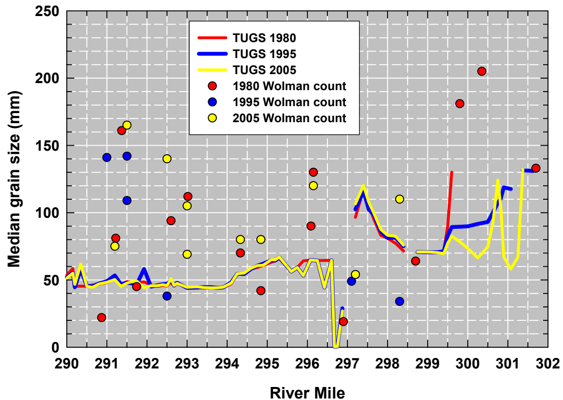
Figure 57. Median grain size versus river mile showing TUGS model predictions (lines) and measurements from Wolman counts (points) for 1980, 1995, and 2005. Agreement between predicted and measured values is about as good as can be expected, given that TUGS generates cross-sectional averages, rather than point measurements of D_{50} , and given the uncertainties in initial conditions for the model.
