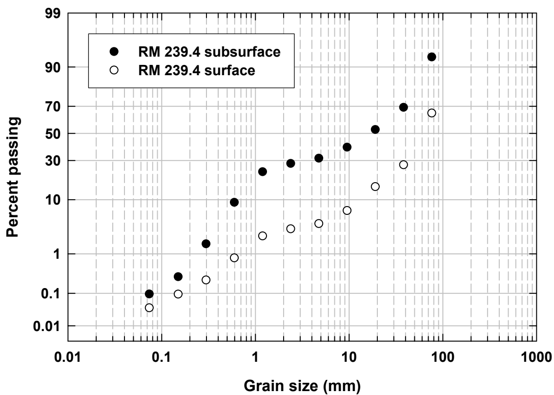
Appendix Figure BS4. Grain-size distribution from bulk sampling at RM 239.4 in 2005. Y axis is a probability scale.
