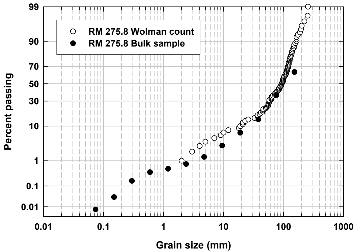
Appendix Figure COMP2. Grain-size distributions of the surface inferred from a Wolman count (open symbols) and a bulk sample (closed symbols) for a site on the Sacramento River in 2005. The Y axis shows a probability scale.
