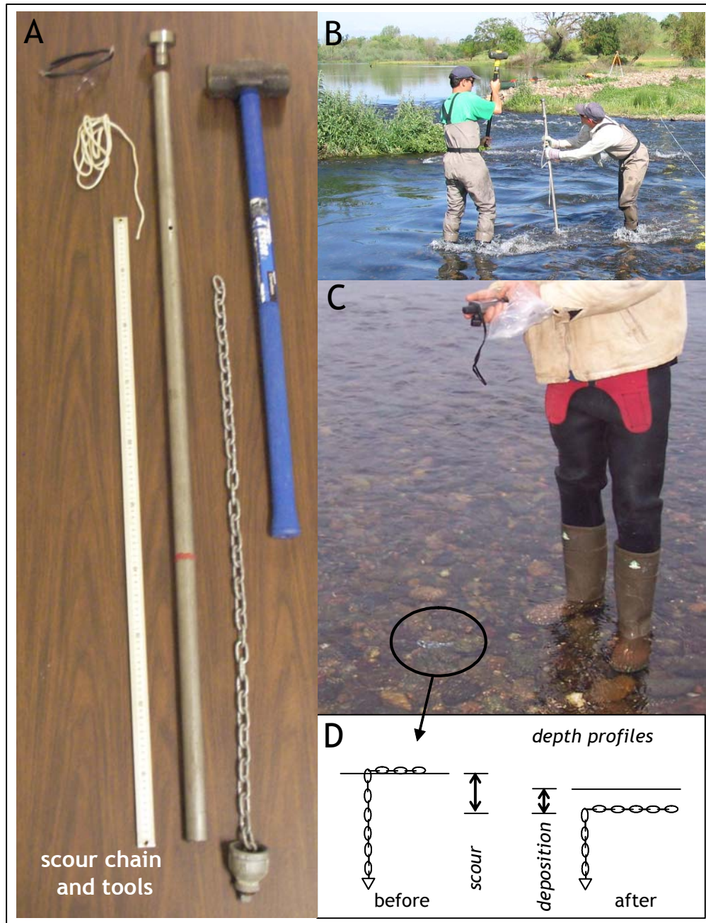
Figure 10. Scour chain installation and monitoring. (A) Scour chain with installation tools. (B) Installation. (C) Scour chains in place in bed after installation. (D) Depth profiles of installed chain before and after a bed mobilizing flow showing monitoring principles: scour can be measured as the difference between the trailing lengths of the chain before and after the flow; deposition (shown in this example to be less than the scour) is measured as the depth to the horizontally oriented length of chain after the flow.
