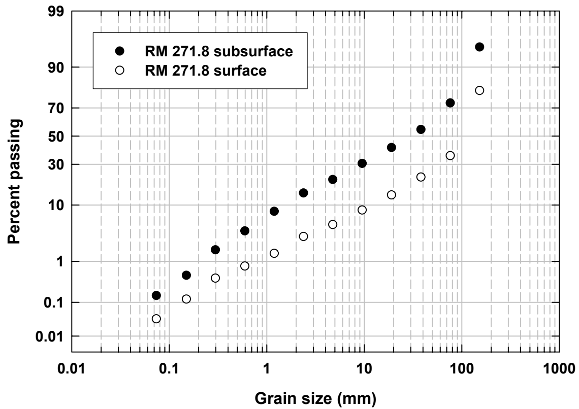
Appendix Figure BS3. Grain-size distribution from bulk sampling at RM 271.8 in 2005. Y axis is a probability scale.
