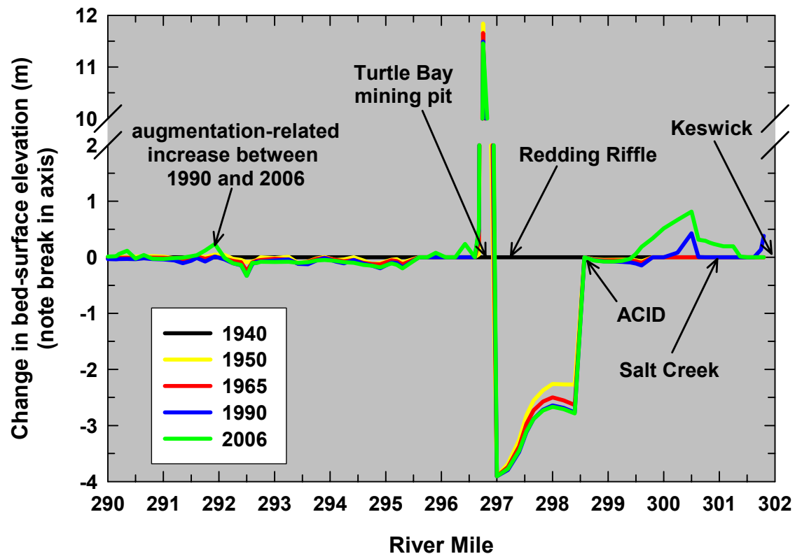
Figure 56. Predicted change in bed elevations (relative to initial conditions) at selected points in time for the upper river, based on TUGS model simulations. The initial depth of the mining pit at Turtle Bay was an unknown boundary condition that had to be assumed. Errors in the assumption would affect the magnitude but not the pattern of changes in the immediate vicinity of the pit. Simulations show an upstream-propagating wave of incision that decreases bed elevations upstream. The actual depth of incision may be limited by the bedrock depth, which, like the depth of the pit, is unknown. The bed is predicted to increase in elevation above RM 299, due to grade control at ACID dam and gravel augmentation at Salt Creek and Keswick Dam. Decreases in bed elevation occur below Turtle Bay, due to the system-wide shutdown in sediment supply. The increase in elevation near RM 290 is due to the simulated effects of gravel augmentation at Tobiasson and Shea Levee.
