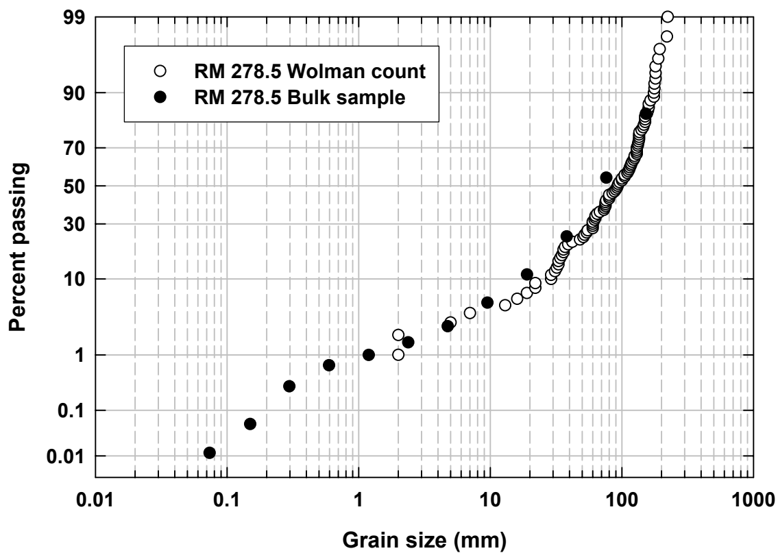
Appendix Figure COMP1. Grain-size distributions of the surface inferred from a Wolman count (open symbols) and a bulk sample (closed symbols) for a site on the Sacramento River in 2005. The Y axis shows a probability scale.
