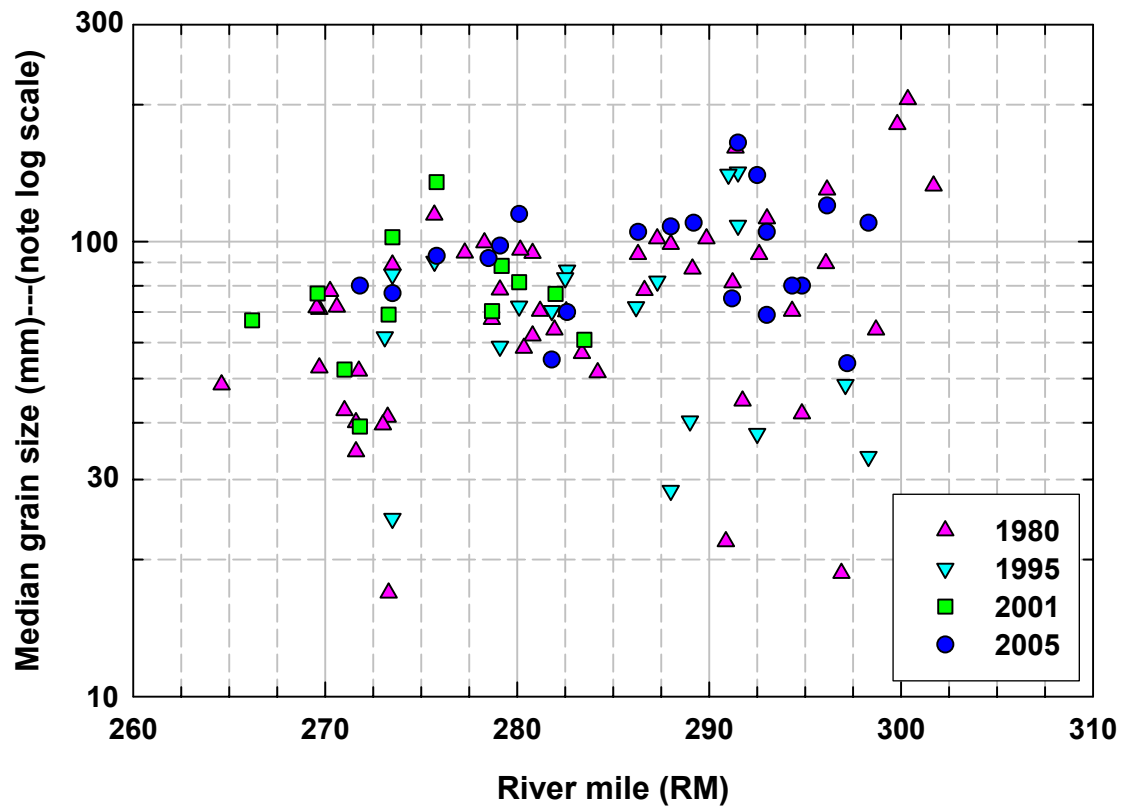
Figure 37. Median grain size on the upper Sacramento River (RM 310-260), based on Wolman pebble counts from geomorphically comparable positions on point bars. A time series of median grain sizes as a function of river mile shows wide scatter within each data set, indicating there is substantial natural variability in grain size at the local (ten- to hundred-meter) scale. Data from later years fall entirely within the range plotted by the earliest data set from 1980. The upper limits on median grain size are essentially constant, indicating that the coarsest deposits have not become substantially coarser (or finer) over the sampling interval. In contrast, the lower limits on median grain size appear to have changed over time, such that it has become increasingly less likely to sample riffles with relatively low median grain sizes (note the absence of data below about 50 mm as of 2001 and 2005). This is broadly consistent with hypothesis 1—the finest riffles appear to have been coarsening over time in the upper river over the last 25 years. A formal, statistical analysis confirms the visual impressions of this plot (see text).
