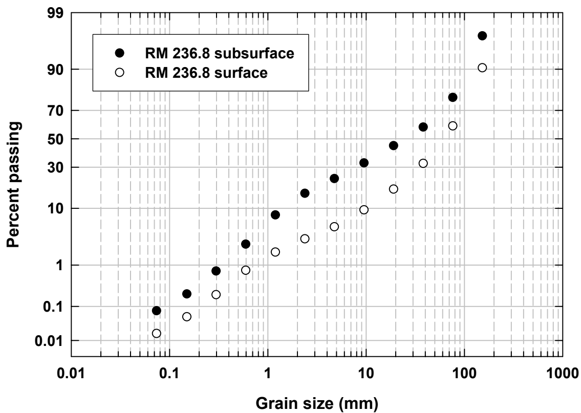
Appendix Figure BS5. Grain-size distribution from bulk sampling at RM 236.8 in 2005. Y axis is a probability scale.
