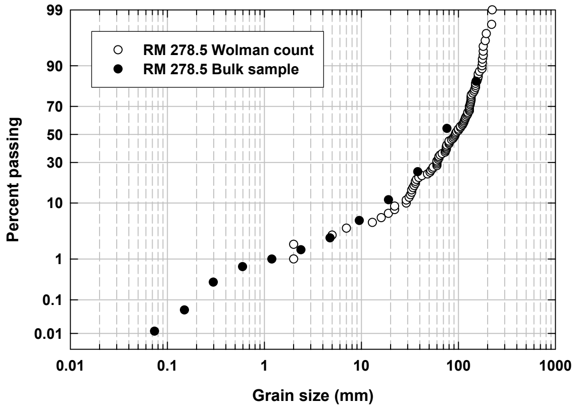
Figure 29. Grain-size distributions of the surface inferred from a Wolman count (open symbols) and a bulk sample (closed symbols) for a site on the Sacramento River in 2005. The Y axis shows a probability scale.
