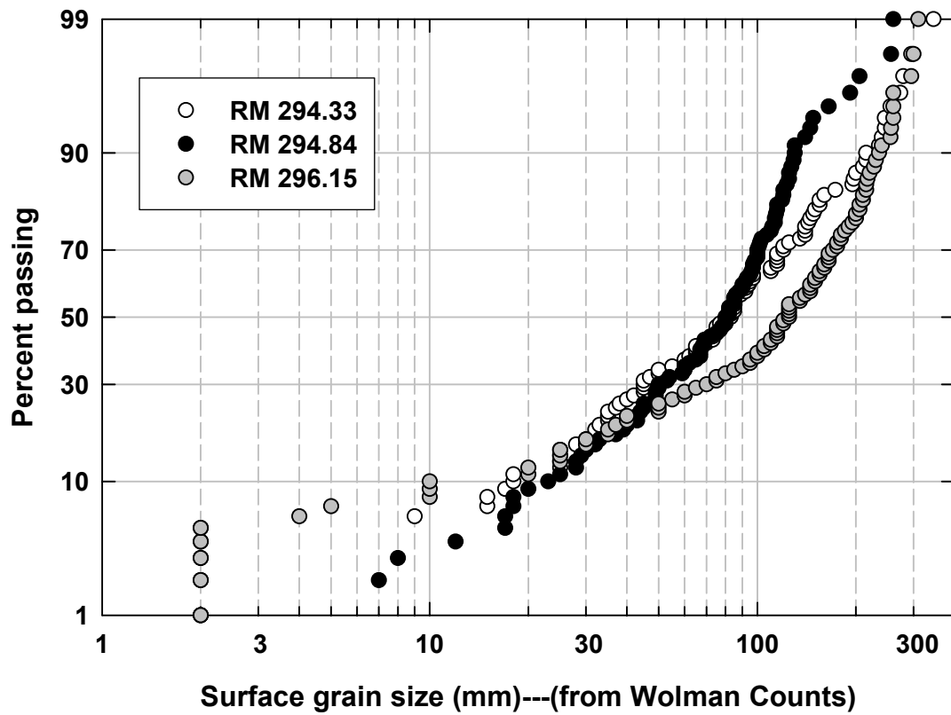
Appendix Figure WC2. Grain-size distributions of the surface inferred from Wolman Counts at 3 locations on the Sacramento River in 2005. The Y axis shows a probability scale.
