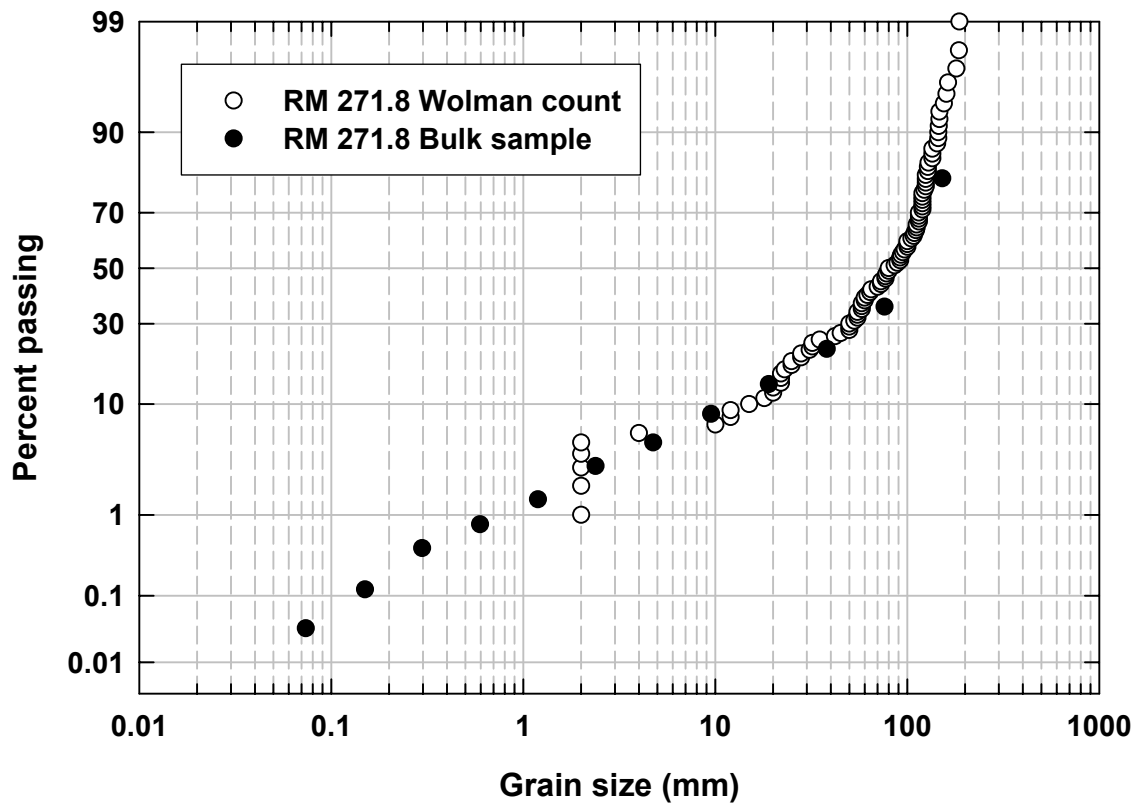
Figure 31. Grain-size distributions of the surface inferred from a Wolman count (open symbols) and a bulk sample (closed symbols) for a site on the Sacramento River in 2005. The Y axis shows a probability scale.
