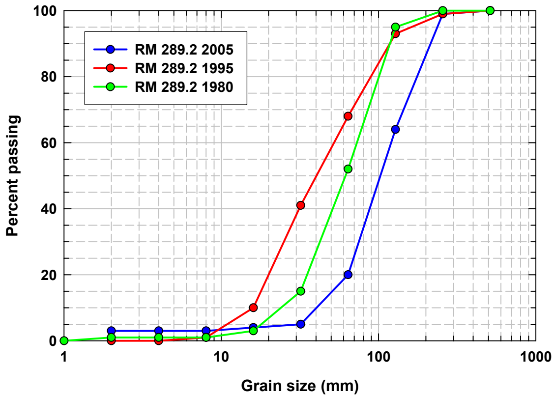
Figure 34. Time series of grain-size distributions from Wolman counts for a location on the upper river. Here, the grain-size measurements from 2005 are binned in "phi"-scale size classes for consistency with previous data. Data suggest the surface became finer by 1995 and then coarsened by 2005.
