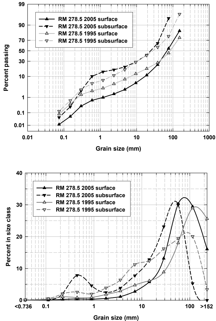
Figure 24. Time series of grain-size cumulative distribution functions (A) and probability distribution functions (B) of the surface (up-pointing triangles, solid line) and subsurface (down-pointing triangles, dashed line) at geomorphically comparable positions on a point bar at RM 278.5, based on data from bulk samples.
