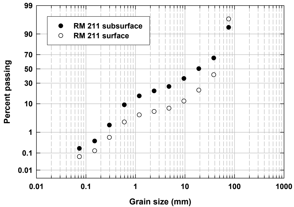
Appendix Figure BS8. Grain-size distribution from bulk sampling at RM 211 in 2005. Y axis is a probability scale.
