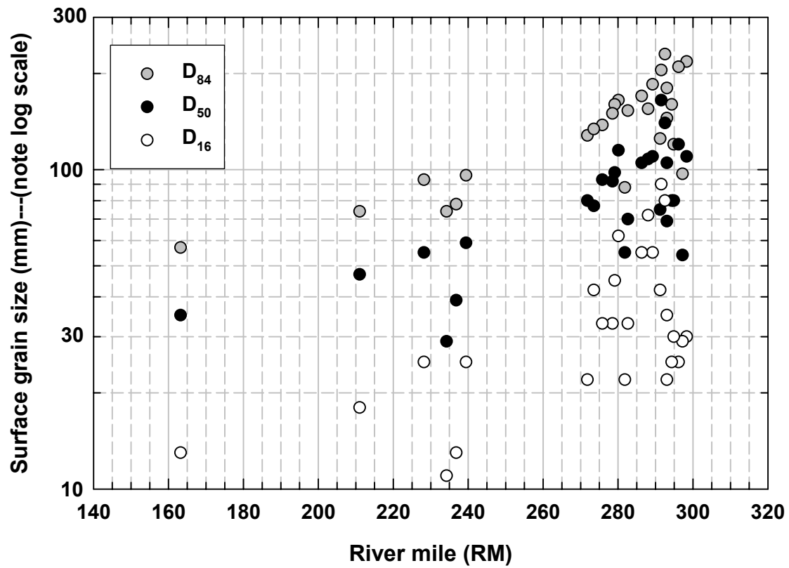
Figure 27. Grain size indexes (determined from Wolman counts) as a function of river mile for heads of point bars (at riffles) in 2005 (this study). Wide scatter within each data set is indicative of substantial natural variability in grain size at the local (i.e., few tens to hundreds of meters) scale.
