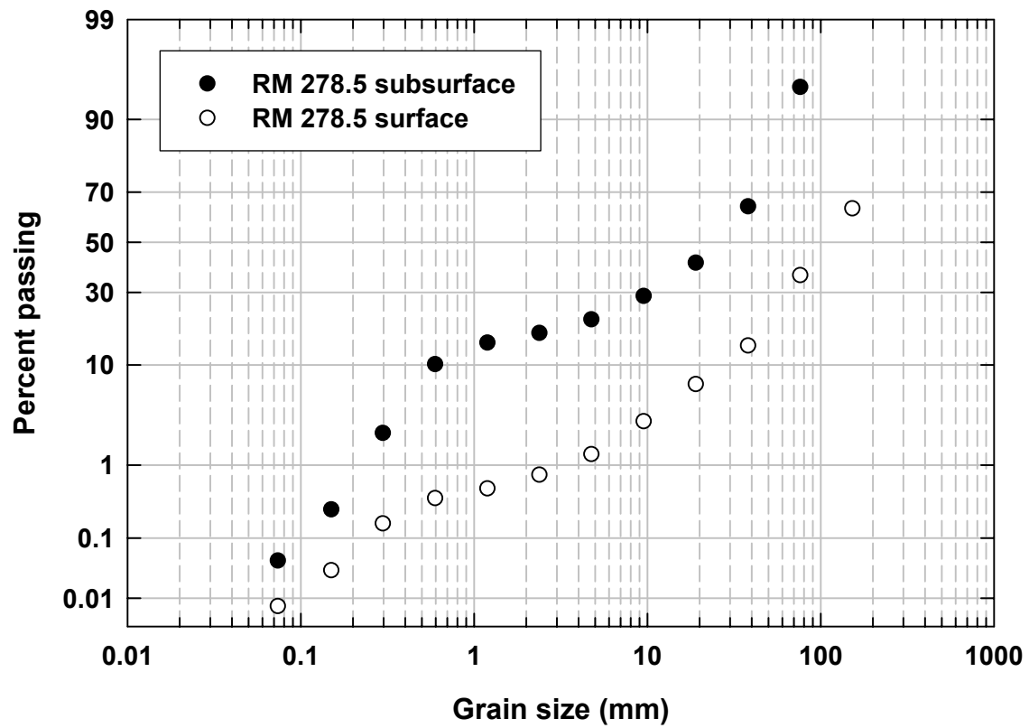
Appendix Figure BS1. Grain-size distribution from bulk sampling at RM 278.5 in 2005. Y axis is a probability scale.
