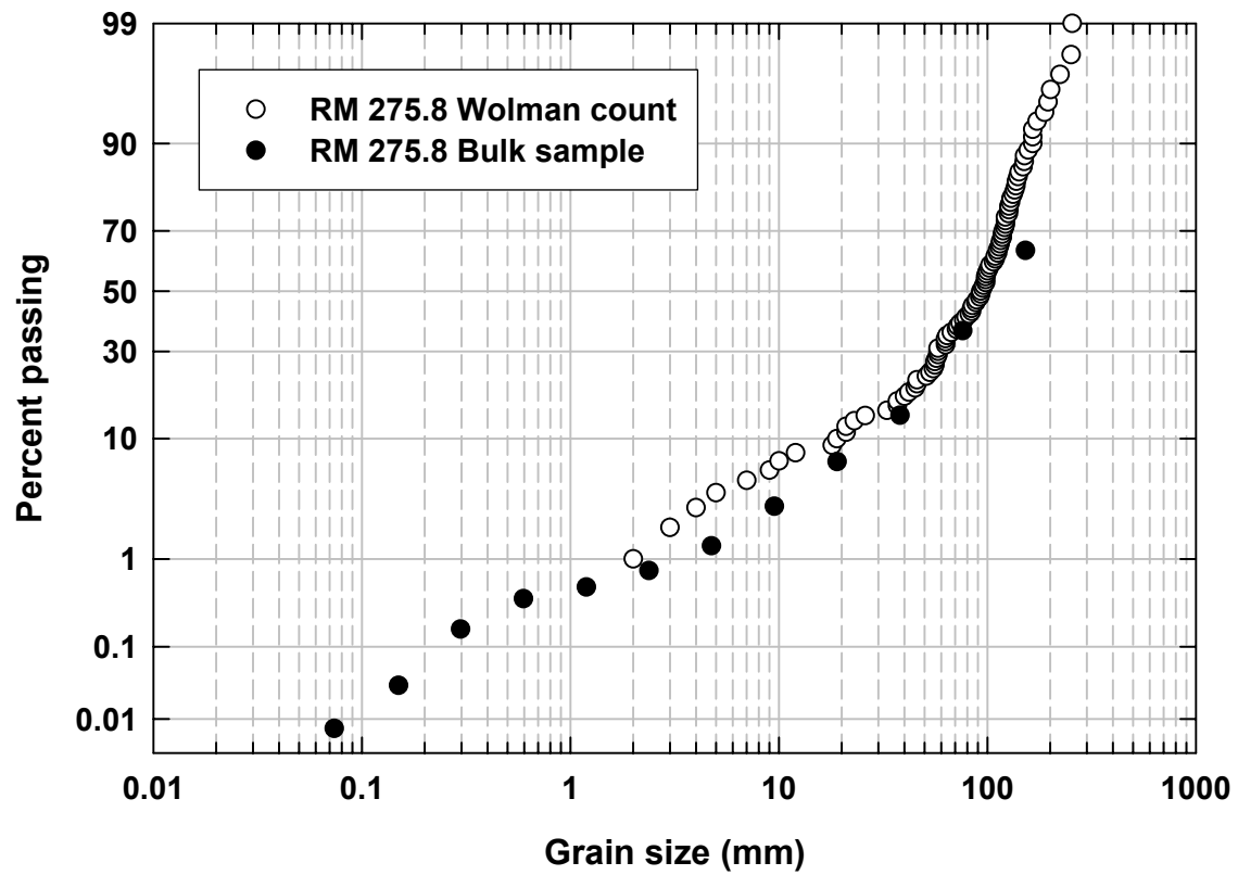
Figure 30. Grain-size distributions of the surface inferred from a Wolman count (open symbols) and a bulk sample (closed symbols) for a site on the Sacramento River in 2005. The Y axis shows a probability scale.
