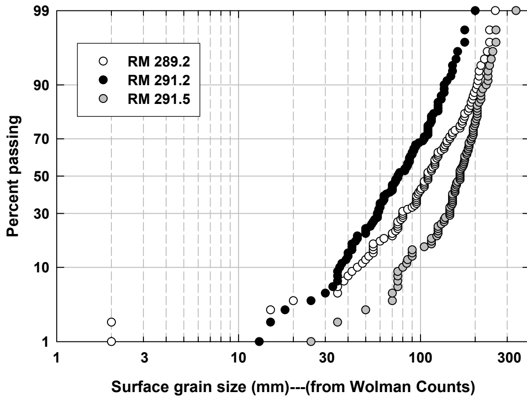
Appendix Figure WC4. Grain-size distributions of the surface inferred from Wolman Counts at 3 locations on the Sacramento River in 2005. The Y axis shows a probability scale.
