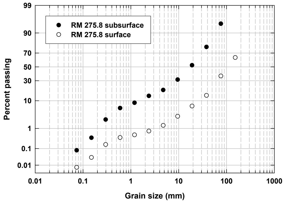
Appendix Figure BS2. Grain-size distribution from bulk sampling at RM 275.8 in 2005. Y axis is a probability scale.
