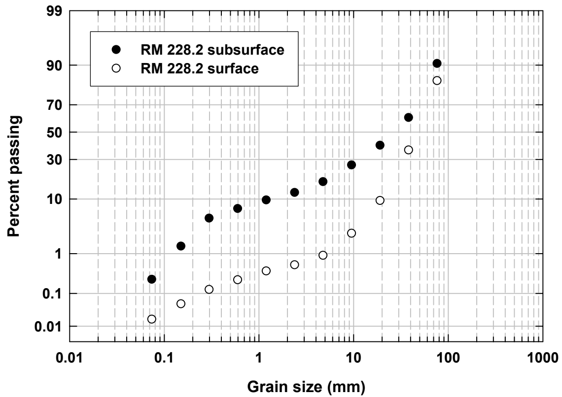
Appendix Figure BS7. Grain-size distribution from bulk sampling at RM 228.2 in 2005. Y axis is a probability scale.
