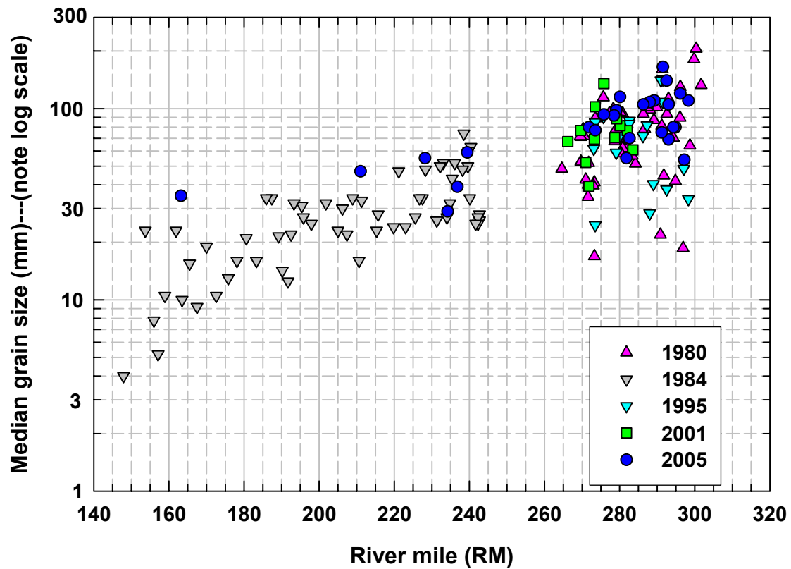
Figure 39. Time series of median grain sizes (determined from Wolman counts) as a function of river mile for geomorphically comparable positions on point bars across the entire study area. Data from Figure 37 and Figure 38 are compiled here for an overall view of grain size versus river mile at the different sampling times.
