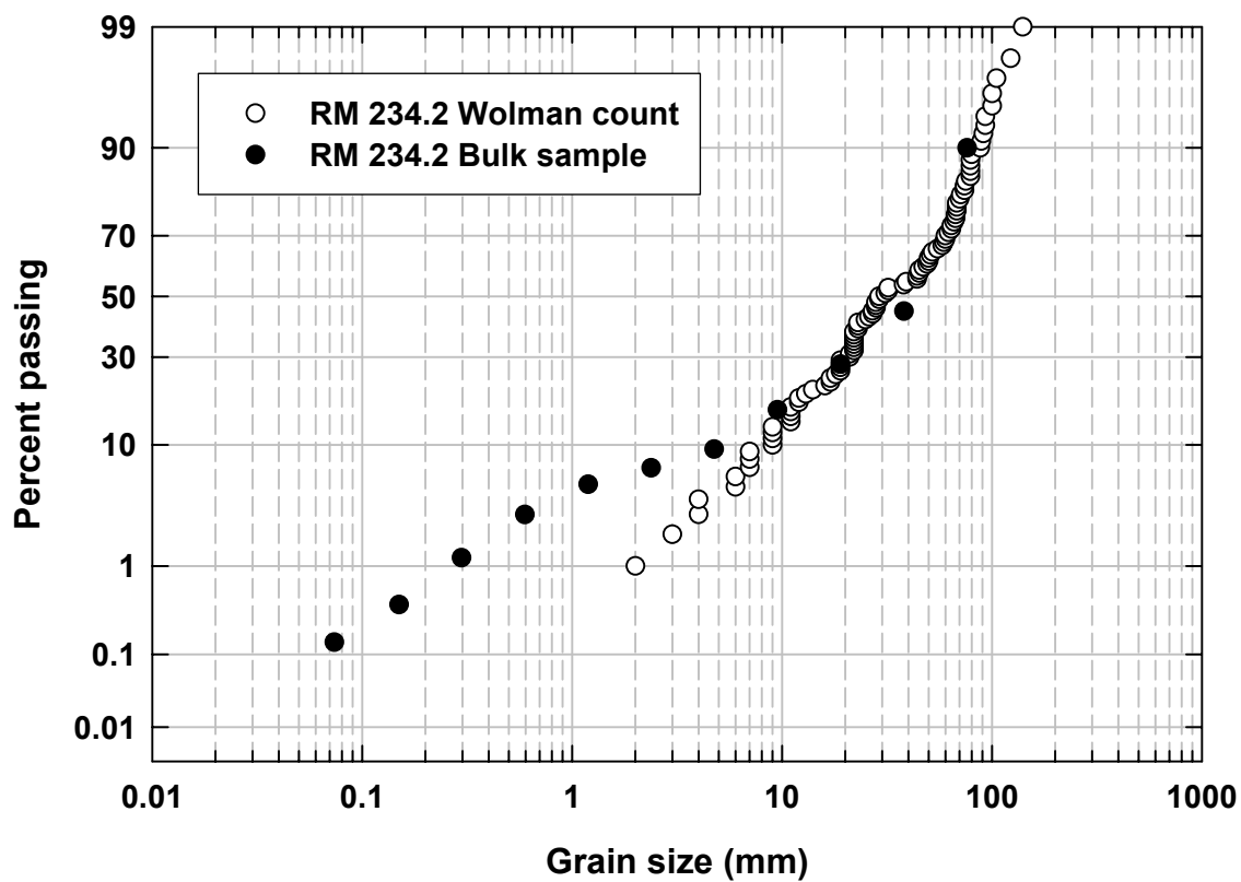
Appendix Figure COMP6. Grain-size distributions of the surface inferred from a Wolman count (open symbols) and a bulk sample (closed symbols) for a site on the Sacramento River in 2005. The Y axis shows a probability scale.
