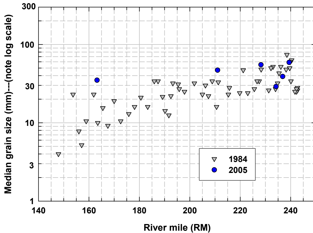
Figure 38. Time series of median grain sizes (determined from Wolman counts) as a function of river mile in the middle river for geomorphically comparable positions on point bars. The wide scatter within the 1984 data set is consistent with substantial (i.e., 3- to 5-fold) natural variability in grain size at the local (ten- to hundred-meter) scale. Overlap among data from the two periods is consistent with little change in median grain size over time; the fact that the grain sizes from 2005 at RM 163 and RM 211 plot somewhat higher than the band of data from 1984 is too isolated to support conclusions about systematic changes in grain size over time.
