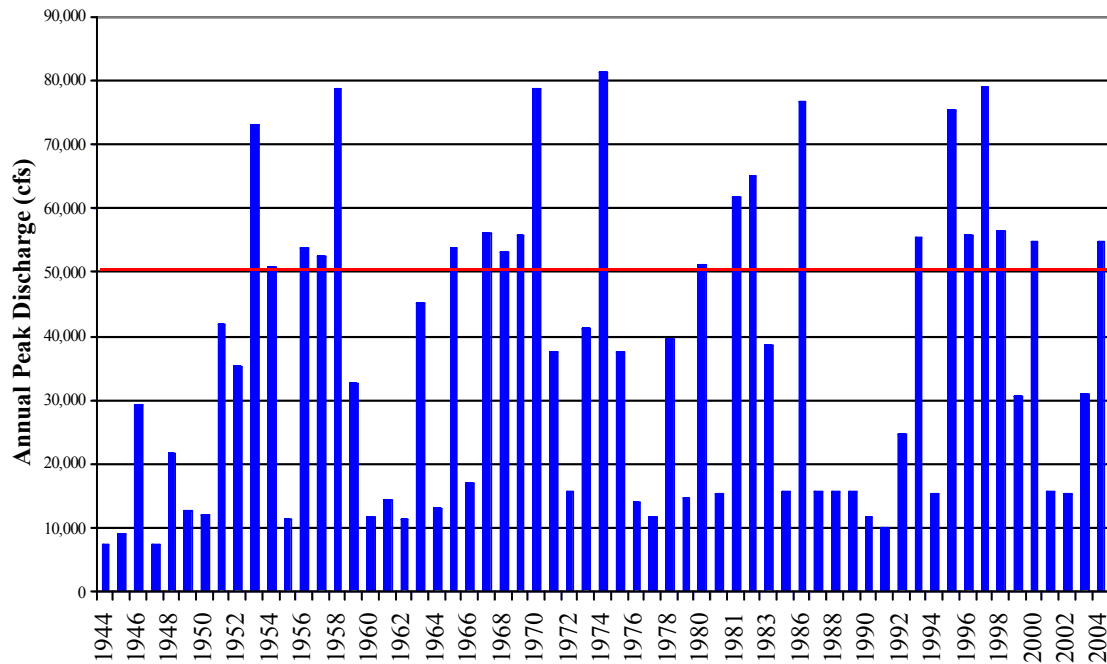
Figure 2. Bed scouring flow events. Since the completion of Shasta Dam in 1945, the USGS gauge at Keswick (no. 11370500) has registered several floods with magnitudes greater than the 50,000 cfs estimated to mobilize and scour spawning-sized gravel below Keswick Dam. Shasta and Keswick dams trap sediment from the upper watershed, depriving downstream reaches of material needed to replenish gravel scoured from the channel bed by high flow releases.
