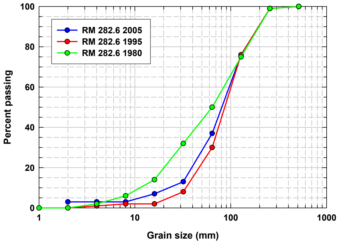
Figure 33. Time series of grain-size distributions from Wolman counts for a location on the upper river. Here, the grain-size measurements from 2005 are binned in "phi"-scale size classes for consistency with previous data. Data suggest the site became coarser by 1995 and then finer from 1995 to 2005.
