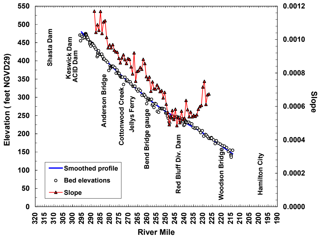
Figure 13. Long profile from 2001 CDWR HEC-RAS modeling of Sacramento River (black circles), with smoothed profile (blue line), and average slope (triangles, in m/m) of the smoothed profile (red line).
