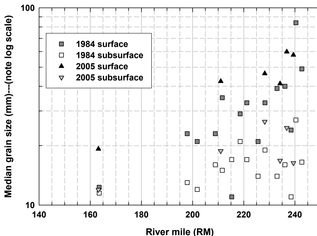
Figure 26. Median grain size in the middle river as a function of river mile for heads of point bars (at riffles) in 1984 and 2005, as determined from bulk samples. The slight offset in both the surface and subsurface samples seems to suggest that samples were coarser in 2005, but this conclusion is not supported by the data because differences in the sampling methods could produce the observed pattern in the absence of coarsening. The smaller sampling plot of the 1984 methodology (Buer 1984) may have biased the sampling toward relatively fine-grained sites, and moreover would have been unable to sample enough particles to make D_{50} statistically representative of the point bar. In contrast, in 2005 when larger plot was sampled, sample sizes were 2 or more times larger than they were in 1984. From a statistical standpoint, this would make the 2005 sampling more robust and less likely to be biased toward fine-grained sites.
