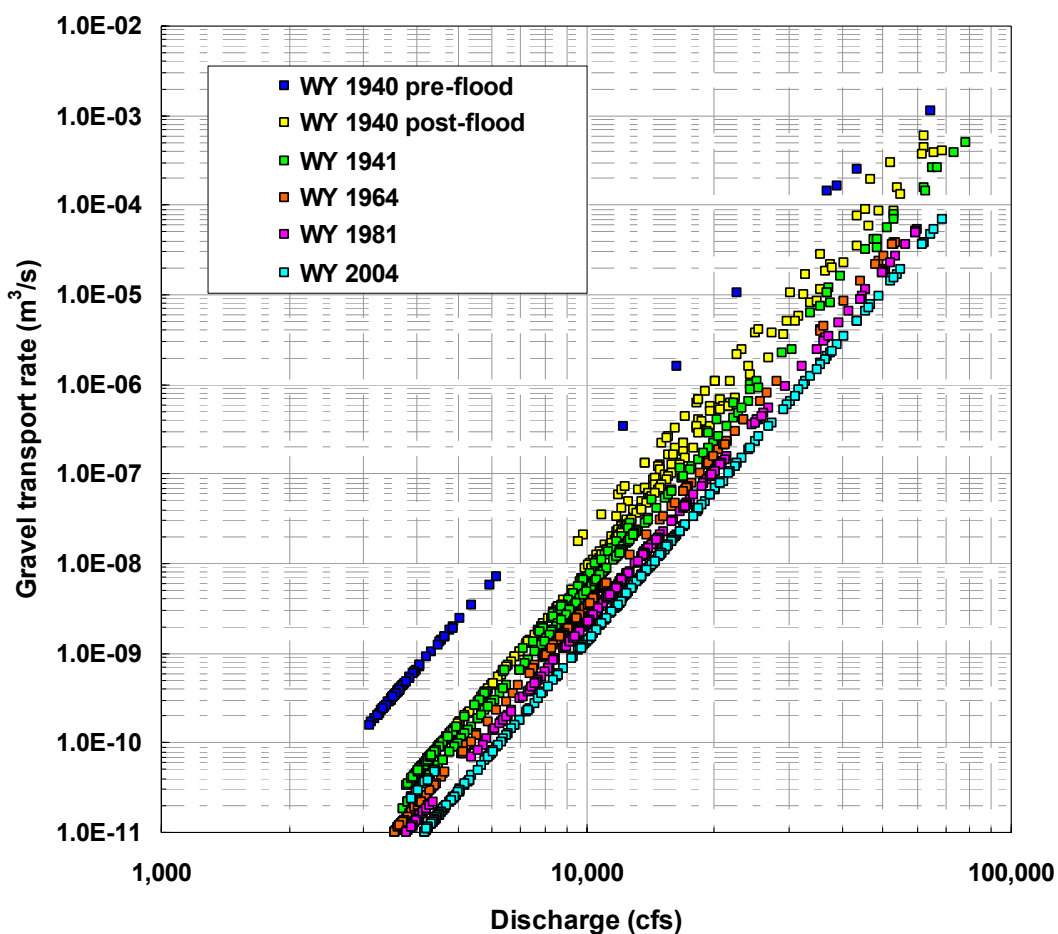
Figure 55. Sediment rating curves from TUGS model simulations at RM 294. The shift in the curves over time is a direct result of coarsening, which reduces bed mobility and thus reduces the predicted amount of sediment transport that should occur for a given flow.
