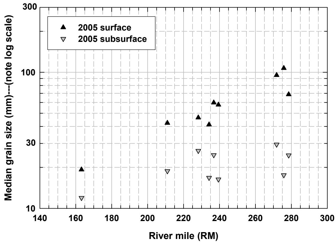
Figure 21. Median grain size as a function of river mile for heads of point bars (at riffles) in 2005, as determined from bulk samples. Median grain sizes of both the surface and subsurface decline, on average, with distance downstream.
