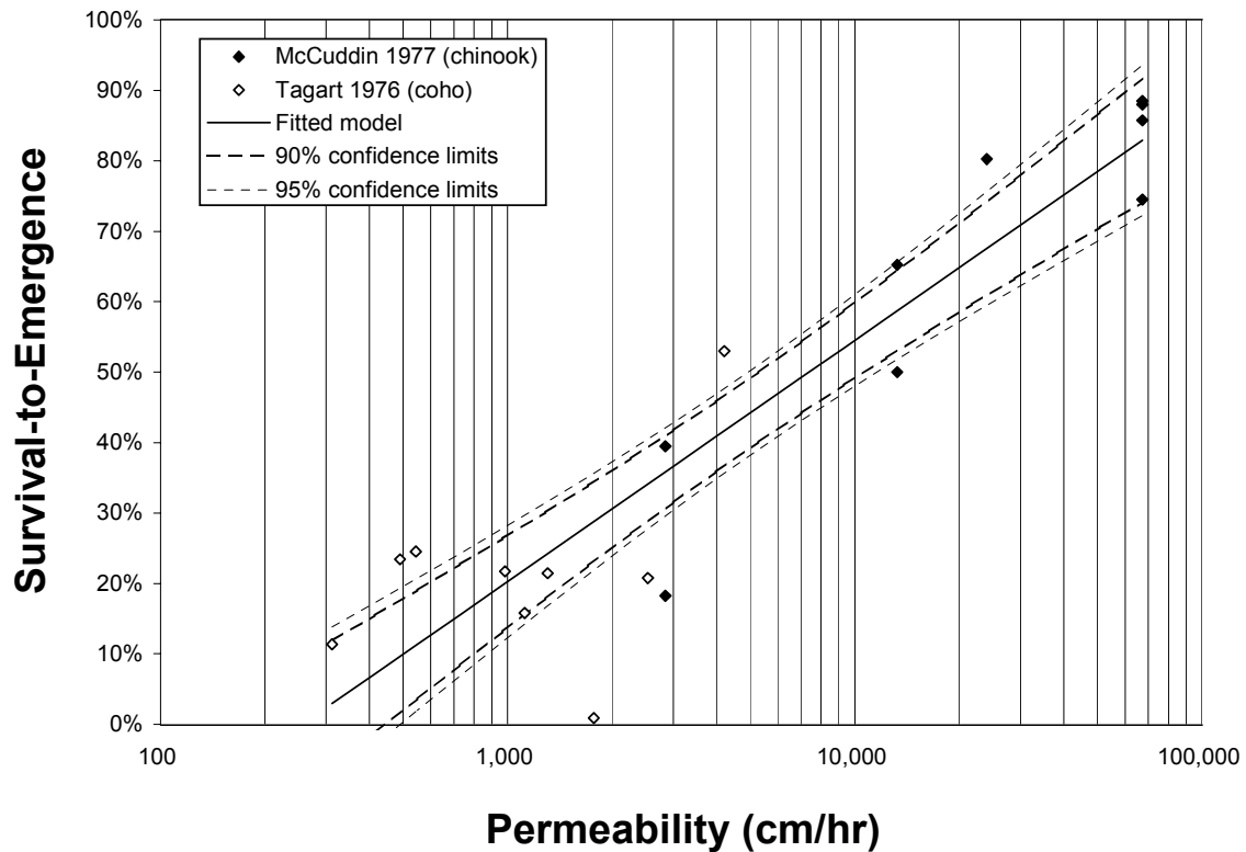
Figure 50. Measured survival to emergence (in %) plotted against the log of measured permeability for coho (Tagart 1976) and Chinook salmon (McCuddin 1977) of the Pacific Northwest, with best fit regression (see equation 1, text) and its 90- and 95-percent confidence limits.
