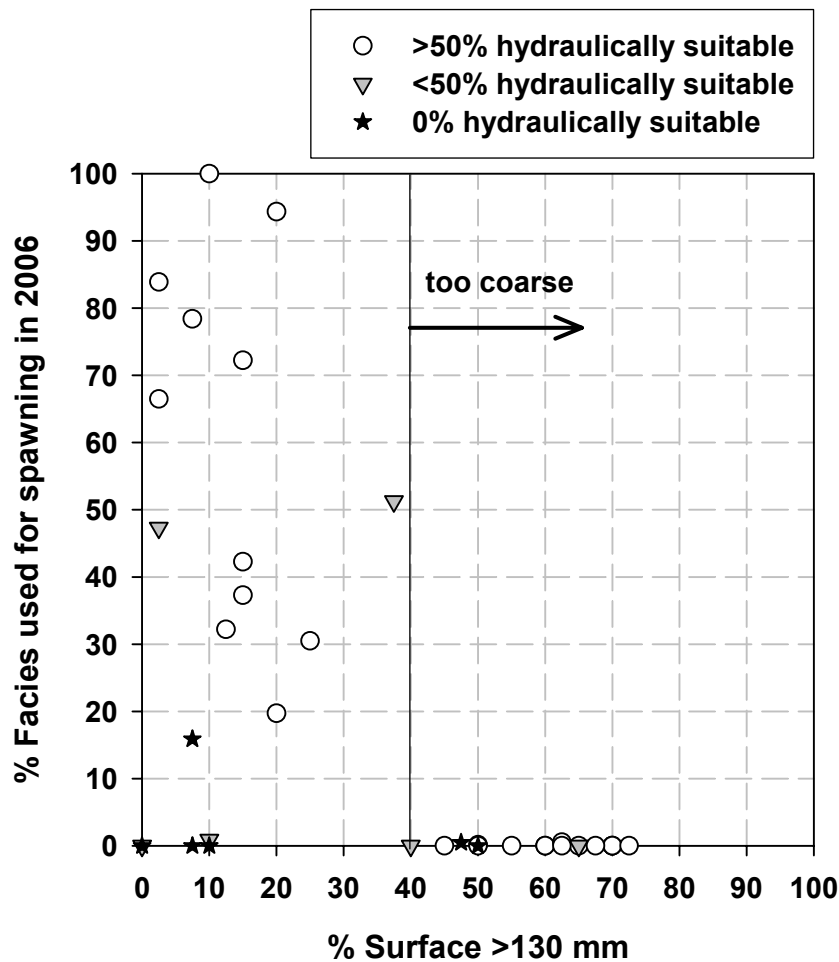
Figure 46. Percent of area used by spawning fish in 2006 against the percent coverage by particles with intermediate axis diameters >130 mm for each of the facies on the Sacramento River. Hydraulic conditions were judged to be mostly favorable for spawning in only some of the facies (plotted as open circles) at the time of the field work. Spawning was scarce or absent in facies where <50% of the area was hydraulically suitable (plotted as triangles for 1-50% and stars for 0%). Spawning was also absent in areas with more than 40% coverage by particles with b-axis diameters >130 mm. We suggest that the 40% level of coarse particles represents an upper threshold on spawning suitability.
