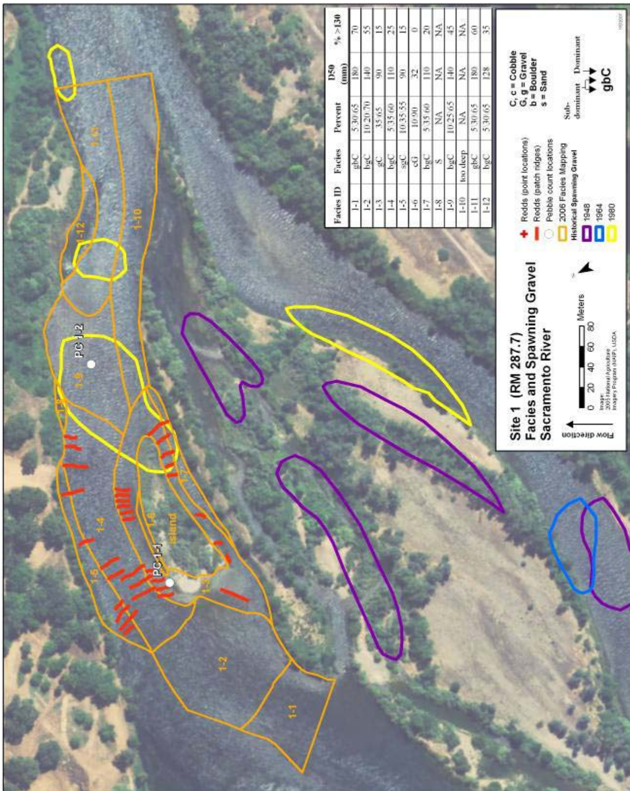
Figure 41. Facies map site 1 at RM 287.7.
