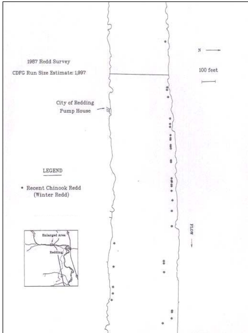
Figure 20. Winter-run Chinook salmon redds in the Sacramento River upstream of Dieselhorst Bridge (RM 299.0–299.3) in 1987. Source: Bigelow 1996.
