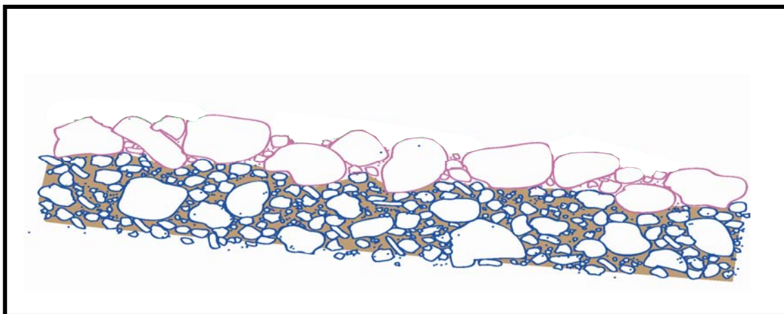
Figure 5. Schematic profile of sediment near the surface of a streambed. A coarse surface layer (pink) overlies a finer subsurface layer (blue). Surface coarsening is an inevitable result of selective transport in the absence of sediment supply. On the Sacramento River, the surface has locally become so coarse that salmonids are no longer able to break through it to spawn in the gravel below. We hypothesize that this may have occurred in many deposits of the upper Sacramento River (Hypothesis 1). We further hypothesize that increased coarsening has been propagating downstream from the dams progressively over time (Hypothesis 2). We also hypothesize that the coarsening process has reduced mobility of the surface such that fine sediment has become trapped beneath it in steadily increasing concentrations, resulting in steadily decreasing spawning gravel quality for a many of the remaining deposits in the post-dam era (Hypothesis 3).
