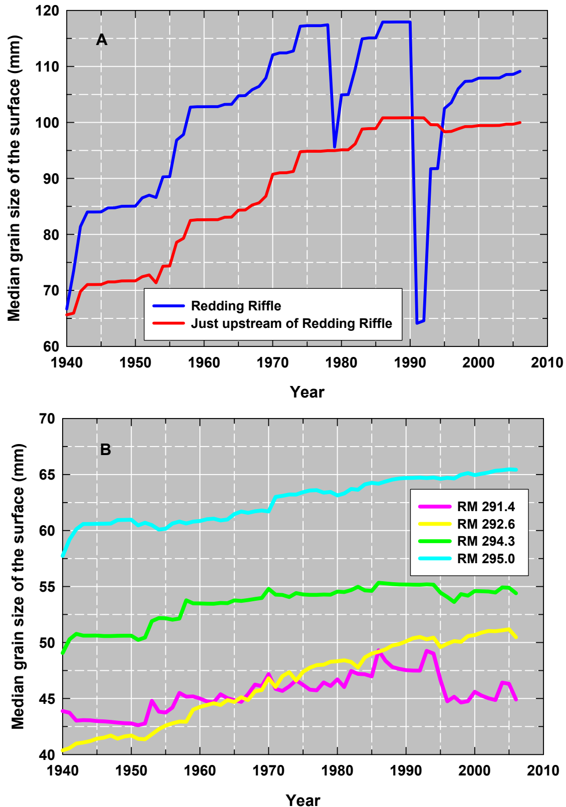
Figure 54. Simulated change in median grain-size of the surface at several sites in reach 2 (A) and reach 3 (b) of the sediment transport modeling analysis.
