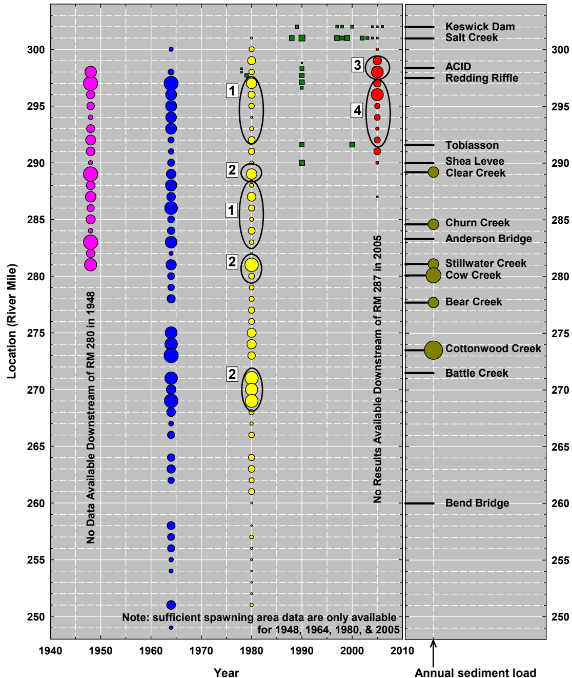
Figure 17. Bubble plot showing spawning habitat area by river mile and year. Surveys of salmonid spawning habitat were conducted in 1948 (pink), 1964 (blue), 1980 (yellow), and 2005 (red). Note: Data from 2005 are incomplete; extensive spawning was observed (but not mapped) downstream of RM 290. Spawning area scales uniformly with bubble area. Green squares show location, timing, magnitude of gravel augmentation (see also Figure 18), with injected volume scaled to plot symbol area. The scale on the right shows major landmarks, with relative annual sediment loads (in mass per unit time; Table 8) of tributaries scaled according to brown bubble area. Labeled circles identify four trends discussed in text: (1) A marked decline in spawning area from 1964 to 1980 from Redding Riffle (RM 298) to RM 292 and from RM 289 to Anderson Bridge (RM 283); (2) Roughly stable spawning area in the immediate downstream vicinity of the river's sediment-bearing tributaries; (3) Greatly increased spawning area in the upper-most reaches of the river by 2005, due to local effects of gravel augmentation; (4) persistence of reduced area from Redding Riffle (RM 298) to RM 292 by 2005.
