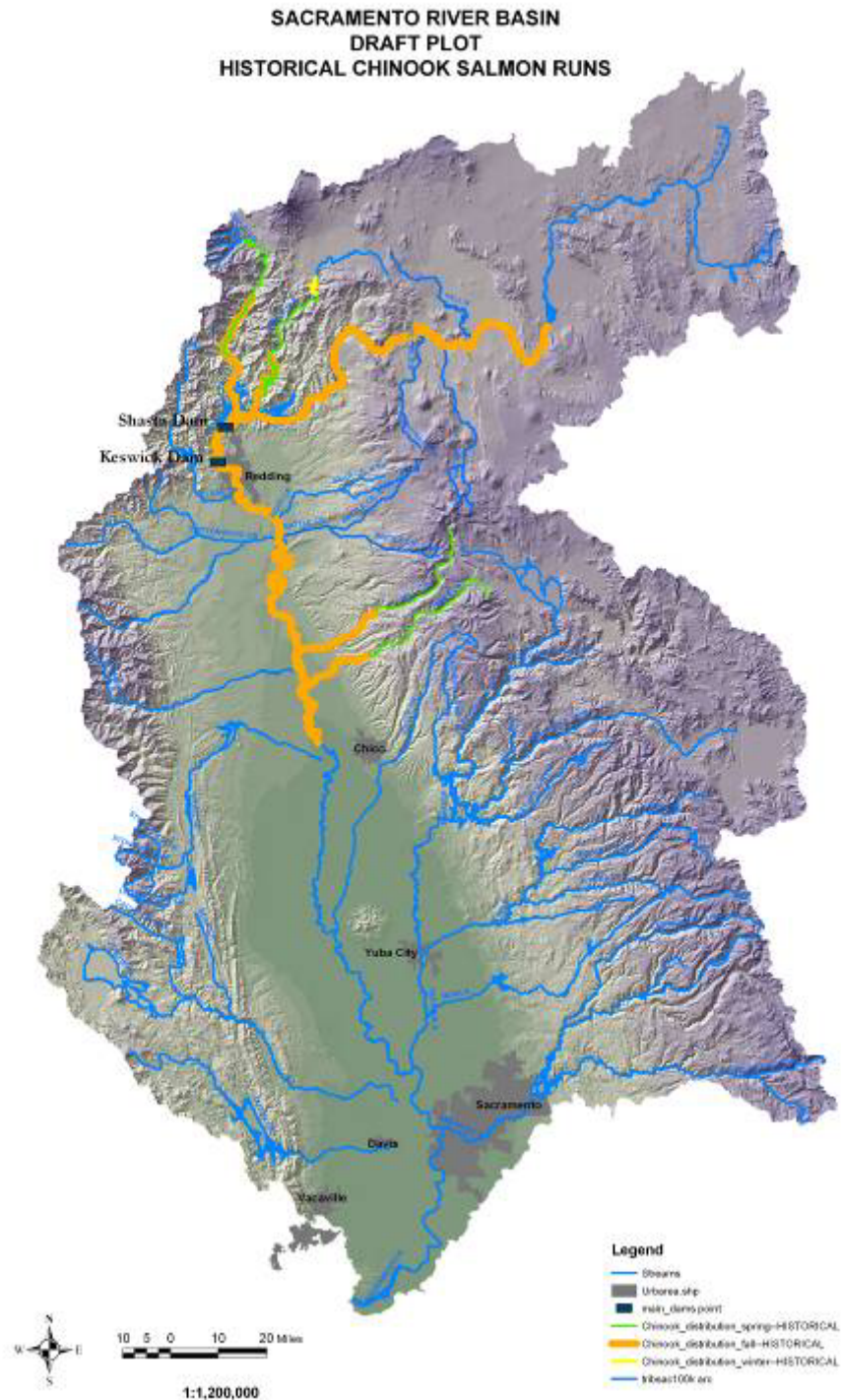
Figure 4. Sacramento River watershed map showing estimated historical extent of spawning for three of the basin's Chinook salmon races. Comparison of this map with the one shown in Figure 1 illustrates how the extent of spawning has been greatly reduced relative to historic conditions.
