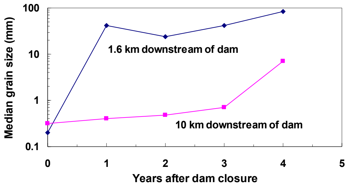
Figure 6. Median grain size as a function of time for two sites on the Colorado River below Hoover Dam. Close to the dam, grain size increased quickly after dam closure. In contrast, grain size at the site farther downstream stayed relatively fine for two years before showing signs of increasing substantially. The delayed response of the more distal site reflects a downstream propagation of surface coarsening after sediment supply was reduced by dam construction. In the case of the Sacramento River, we expect that the coarsening has been less pronounced, because initial conditions below Keswick Dam were much coarser than they were below Hoover Dam. Source: Williams and Wolman (1984).
