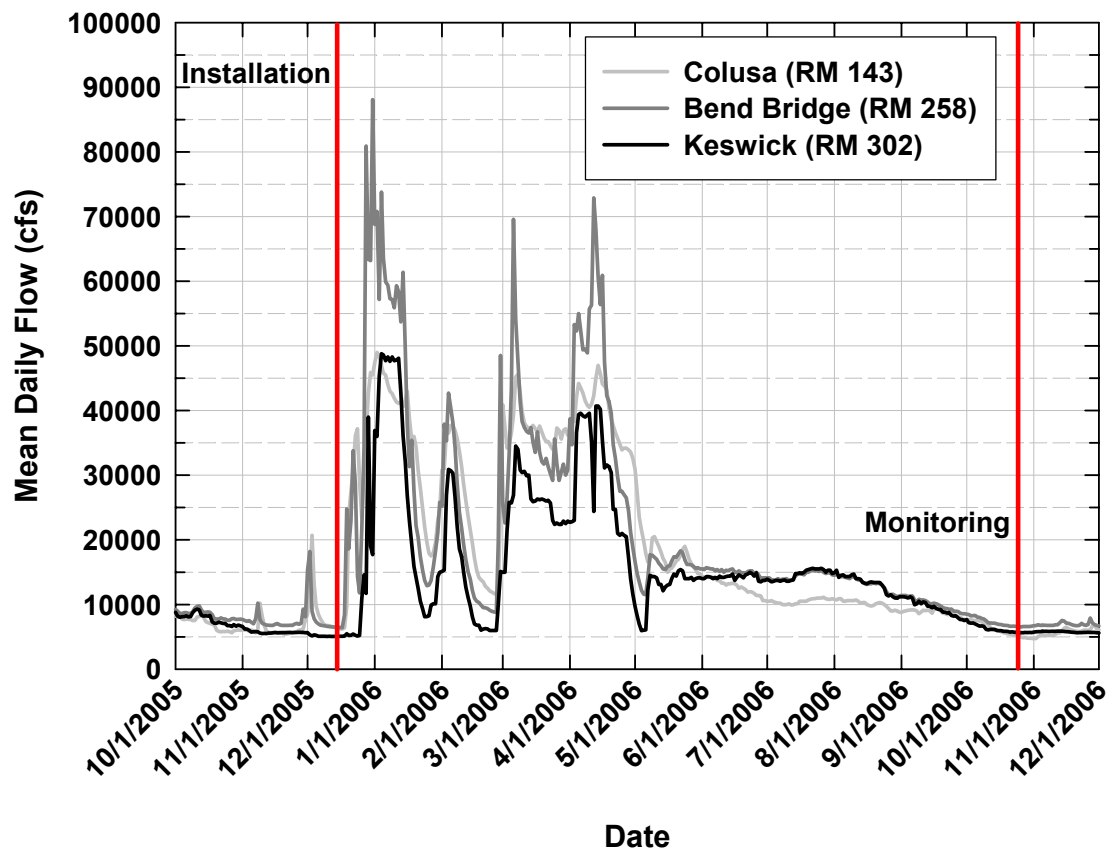
Figure 12. Mean daily flow at Keswick (RM 302), Bend Bridge (RM 258), and Colusa (RM 143), 3 USGS gauges that span the upper and middle sections of the river. Vertical lines mark the installation and monitoring dates of the bed scour study. Daily flow averaged greater than 60,000 cfs at Bend Bridge for 14 days in the interval. The peak daily flow at Bend Bridge was 88,100 cfs. Note that instantaneous peak flows for each of the WY 2006 flood pulses on the Sacramento River would likely plot significantly higher than the mean daily peaks plotted here.
