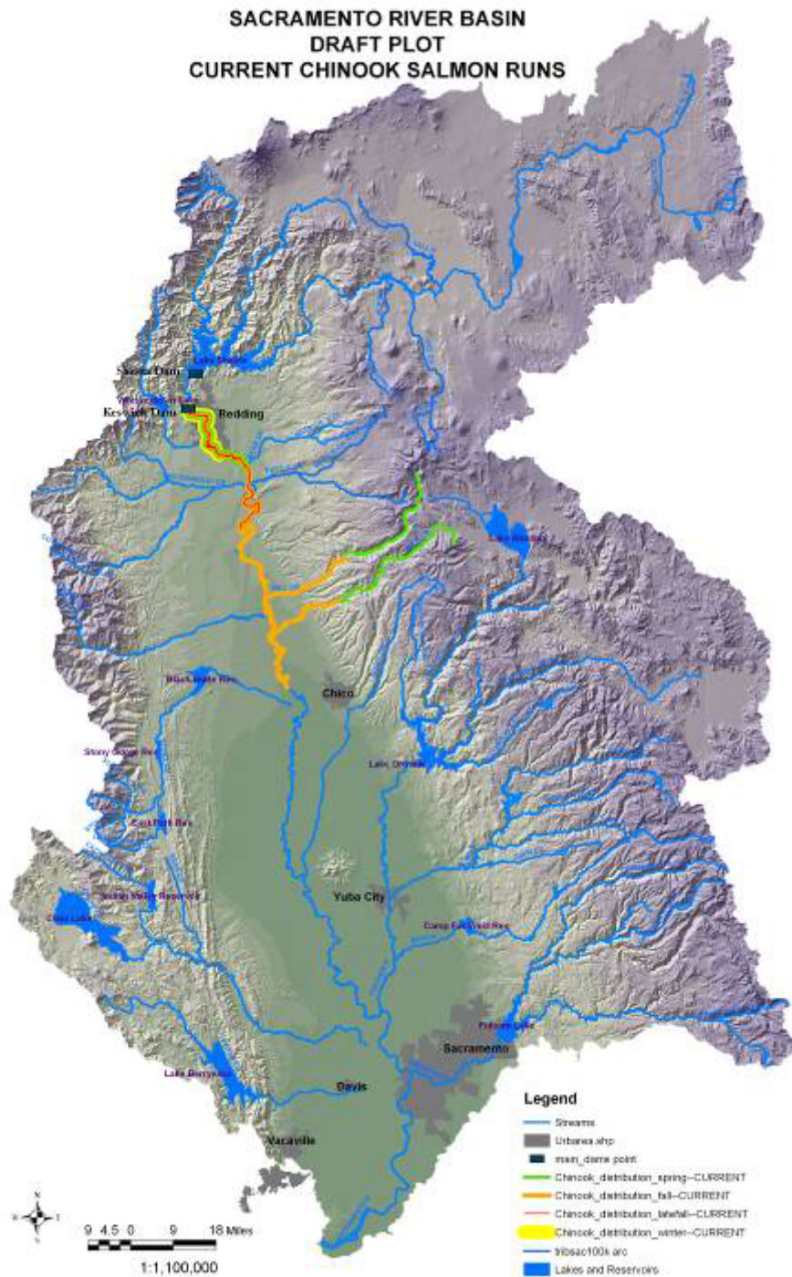
Figure 1. Sacramento River watershed map showing estimated current extent of spawning for each of the basin's four Chinook salmon races.
