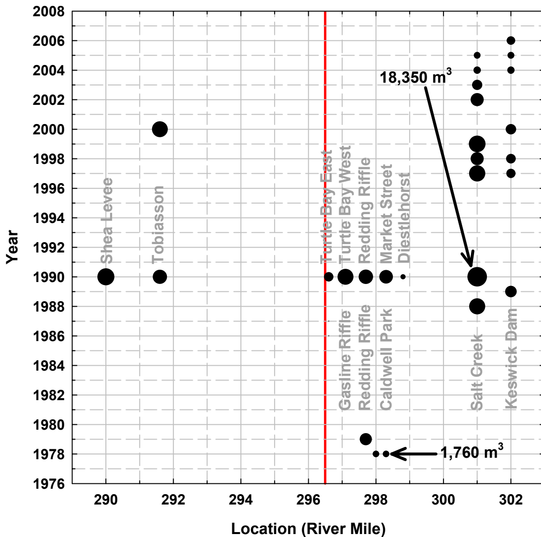
Figure 18. Bubble plot of gravel augmentation by year and river mile for the upper Sacramento River. Bubble area scales proportionally with volume added. The lowest (1760 m 3 ) and highest (18,350 m 3 ) augmentation volumes are labeled for scale. Vertical line marks location of Turtle Bay, a deep, remnant in-stream mining pit that can presumably trap much of any sediment in transit from upstream and thus significantly disrupt the continuity of sediment transport of more than half of the gravel that has been added to the river.
