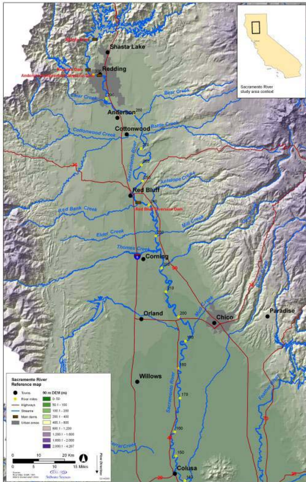
Figure 2. Shaded relief map of the northern Central Valley of California. The study area of the Sacramento River Ecological Flows Project extends along the mainstem from RM 302 (at Keswick Dam) to RM 143 (at Colusa).
