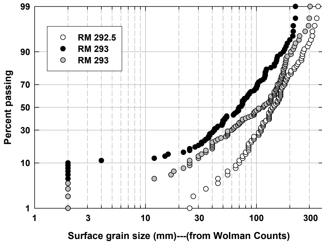
Appendix Figure WC3. Grain-size distributions of the surface inferred from Wolman Counts at 3 locations on the Sacramento River in 2005. The Y axis shows a probability scale.
