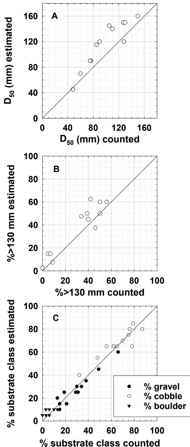
Figure 48. Comparison of estimated (vertical axes) and measured (horizontal axes) median particle size (A), percent coverage by particles with intermediate diameters >130 mm (B), and percent occurrence of each qualifying substrate class (C). Lines mark perfect agreement between estimated and measured values. Estimates of D_{50} were systematically high but generally within \pm 20\% of the measured value. Errors in estimated coverage by coarse particles and individual substrate types were typically less than 20% and 10%, respectively.
