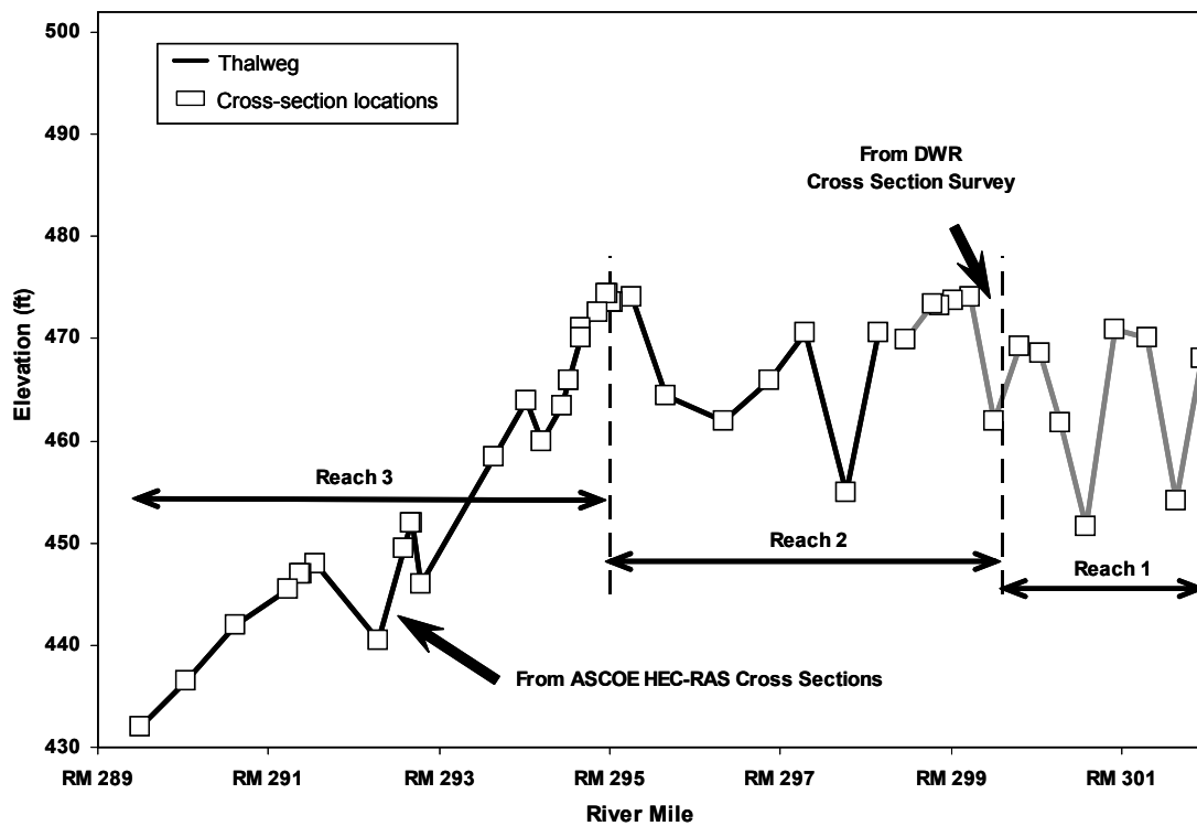
Figure 14. Thalweg profiles for three subreaches where dam-related coarsening is expected to have been most significant. TUGS model was applied to each subreach, but only reach 3 had enough cross-section data to resolve effects of sediment transport on individual spawning areas.
