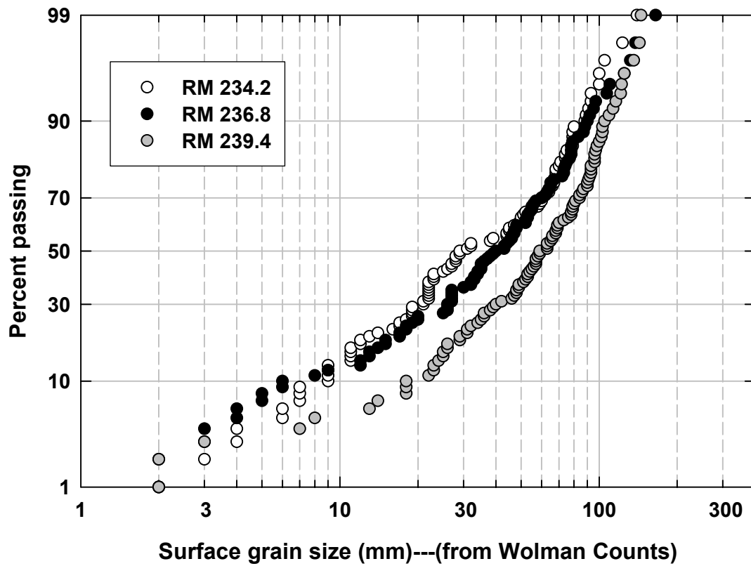
Appendix Figure WC9. Grain-size distributions of the surface inferred from Wolman Counts at 3 locations on the Sacramento River in 2005. The Y axis shows a probability scale.
