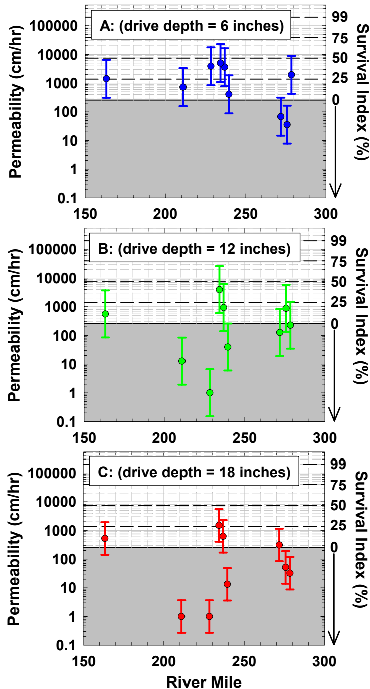
Figure 49. Permeability (left axis) and estimated survival index (right axis) in 2005 at 6 inches (A), 12 inches (B), and 18 inches (C) as a function of river mile for the middle and upper reaches of the Sacramento River. Data collected in 2006 and after "redd building" were excluded from the plots (see text). Permeability shows no clear trend with river mile for any of the drive depths. Survival index scaling and units (% survival) are based on available data for coho and Chinook salmon of the Pacific Northwest (see next figure). Shaded regions have estimated survival index equal to 0%. Low survival indices suggest that many of our sites would be unsuitable for successful spawning due to low permeability. This seems especially true at 12 and 18 inches (B and C), at depths where Sacramento River Chinook salmon are generally observed to bury their eggs. This highlights the likely importance of redd building as a mechanism for cleaning gravel (and thus enhancing its permeability) at spawning sites.
