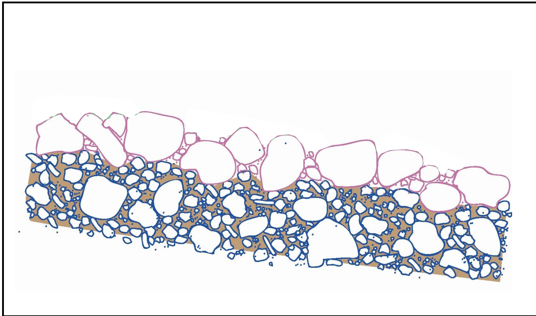
Figure 4.2-12. Illustration of an armored bed. As high flow releases from Shasta Dam transported gravels downstream, a greater proportion of the channel bed surface was covered by larger particles that could not be mobilized by high flow events. This armor layer traps gravels in the subsurface, making them unavailable for spawning.
