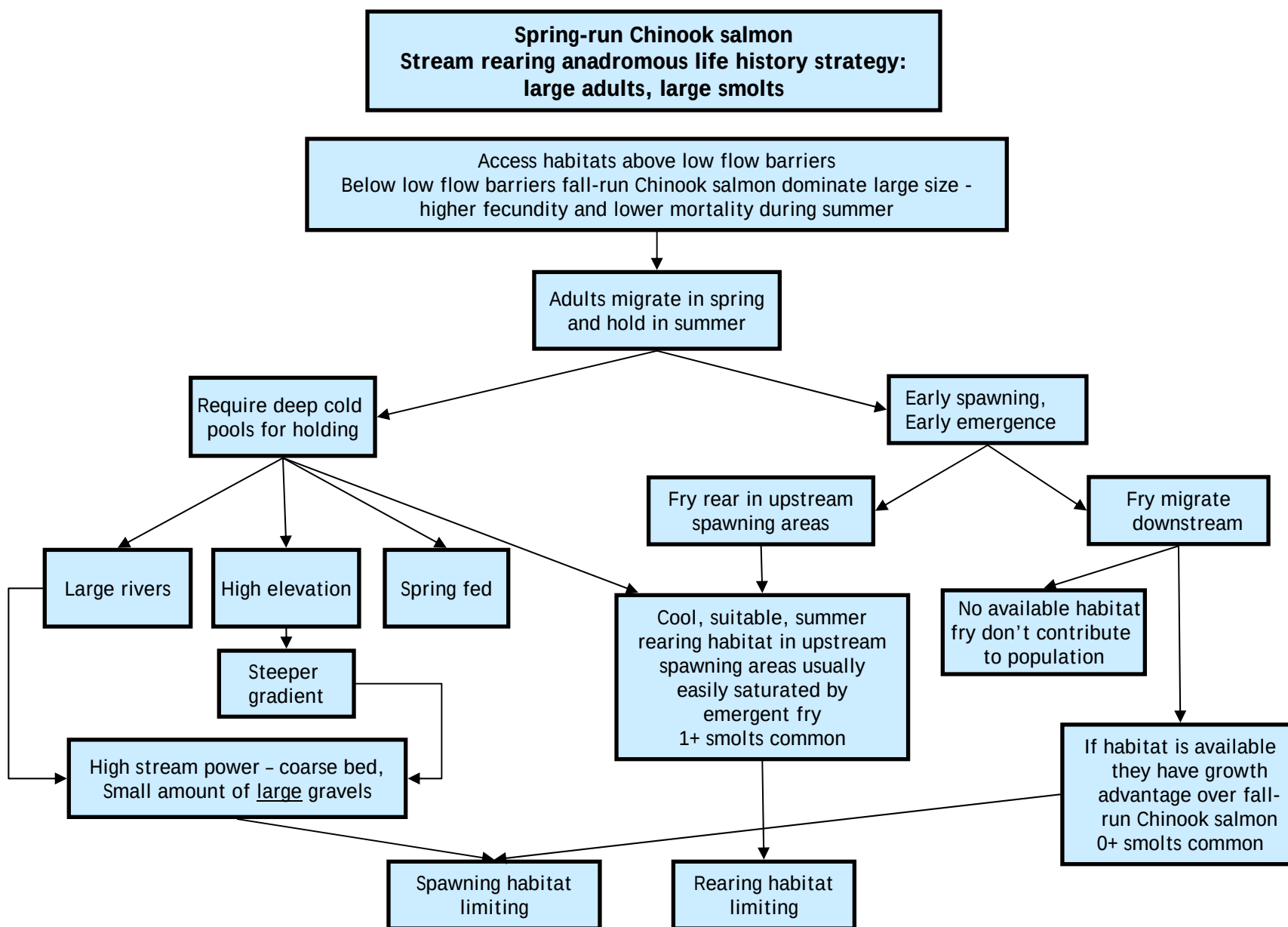
Figure 4.3-2. Spring-run Chinook salmon conceptual model of the Sacramento River.
