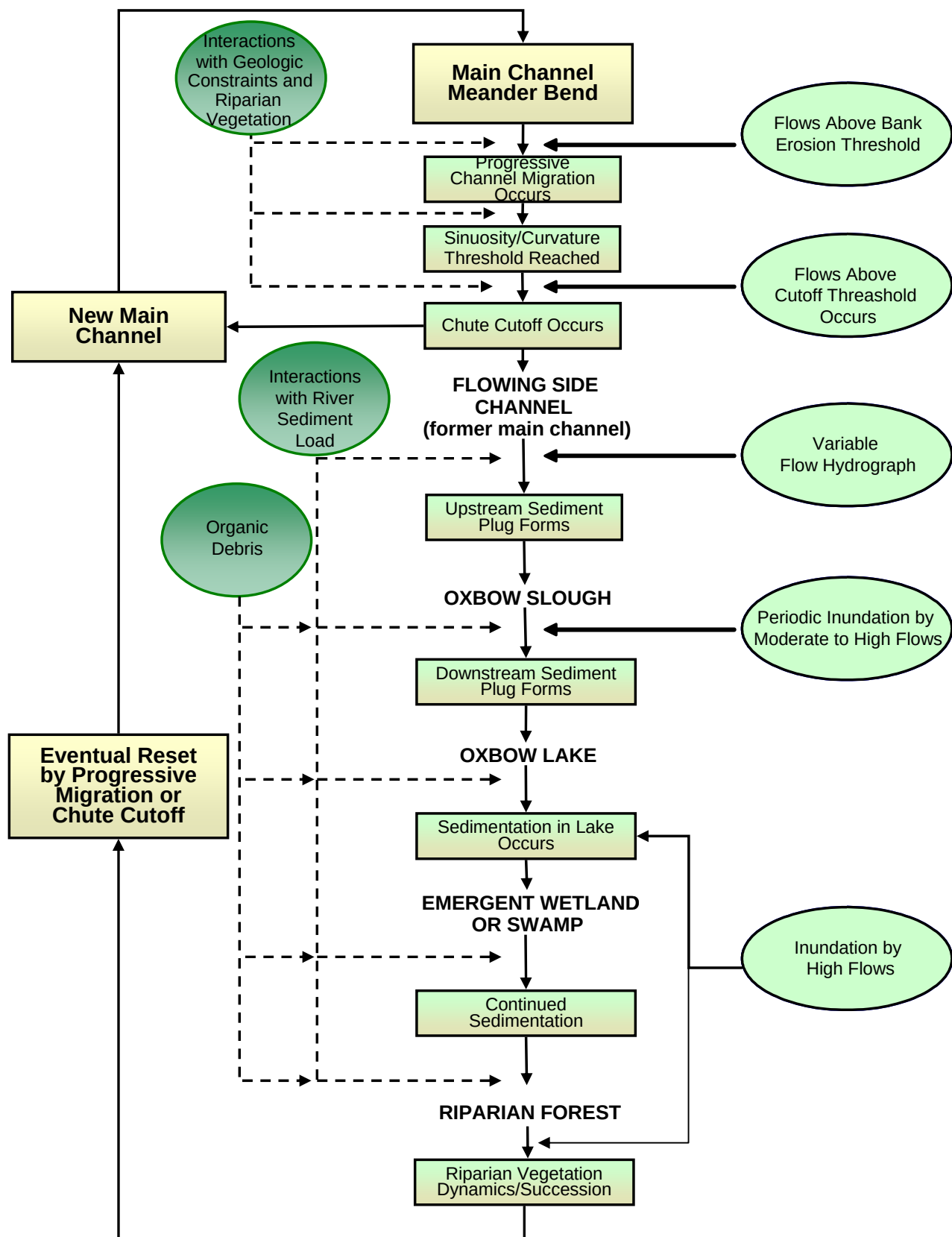
Figure 8-2. Habitats associated with chute cutoffs.
