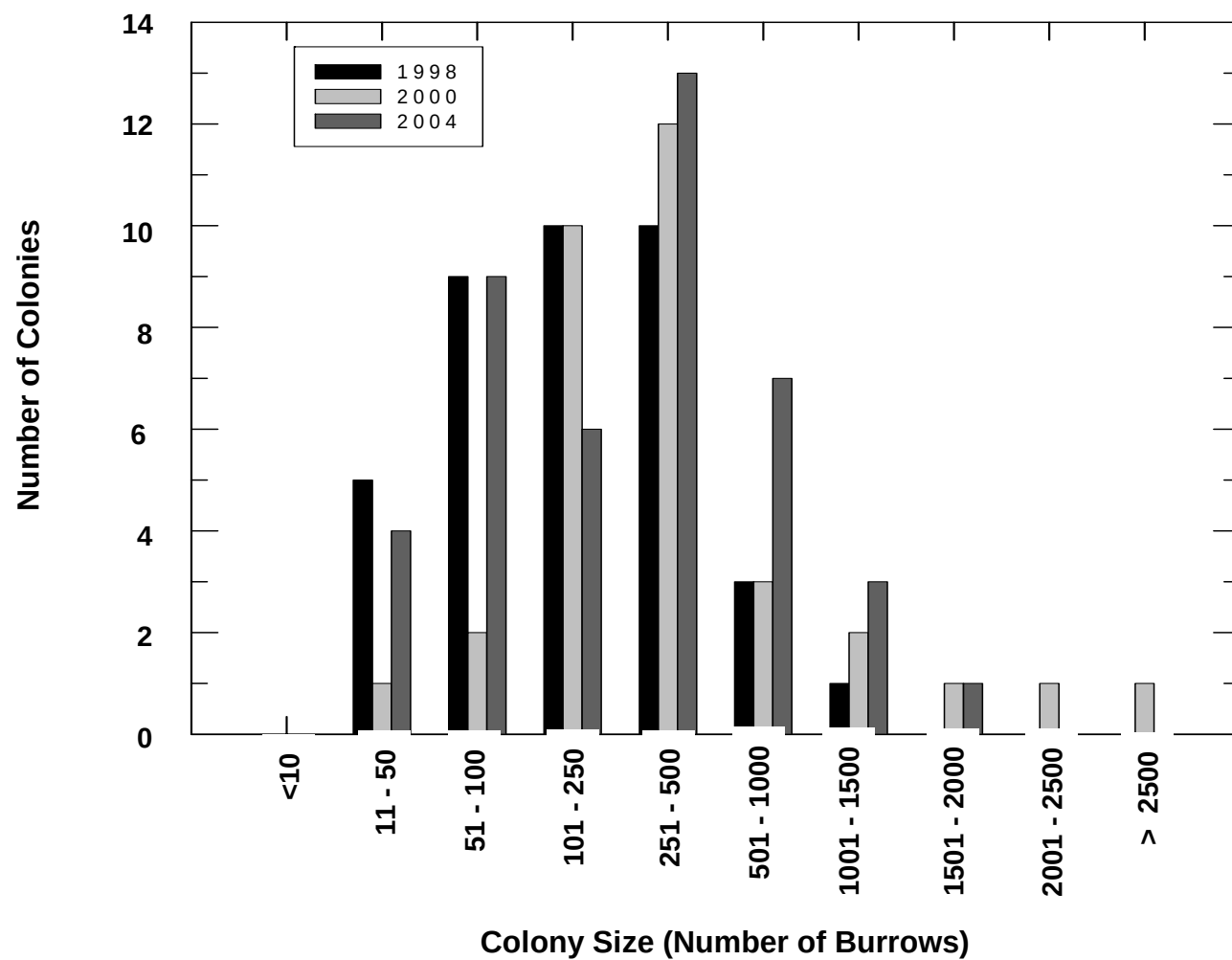
Figure 7-16. Frequency distribution of bank swallow colony sizes (total number of burrows per colony) in the Sacramento River valley for 3 recent survey years. Source: Schlorff 1998, 2001, 2004.
