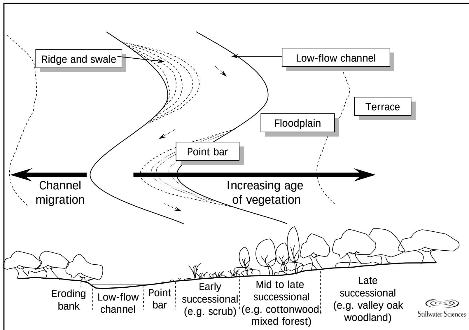
Figure 9-10. Schematic diagram of riparian succession conceptual model for meandering alluvial rivers.
