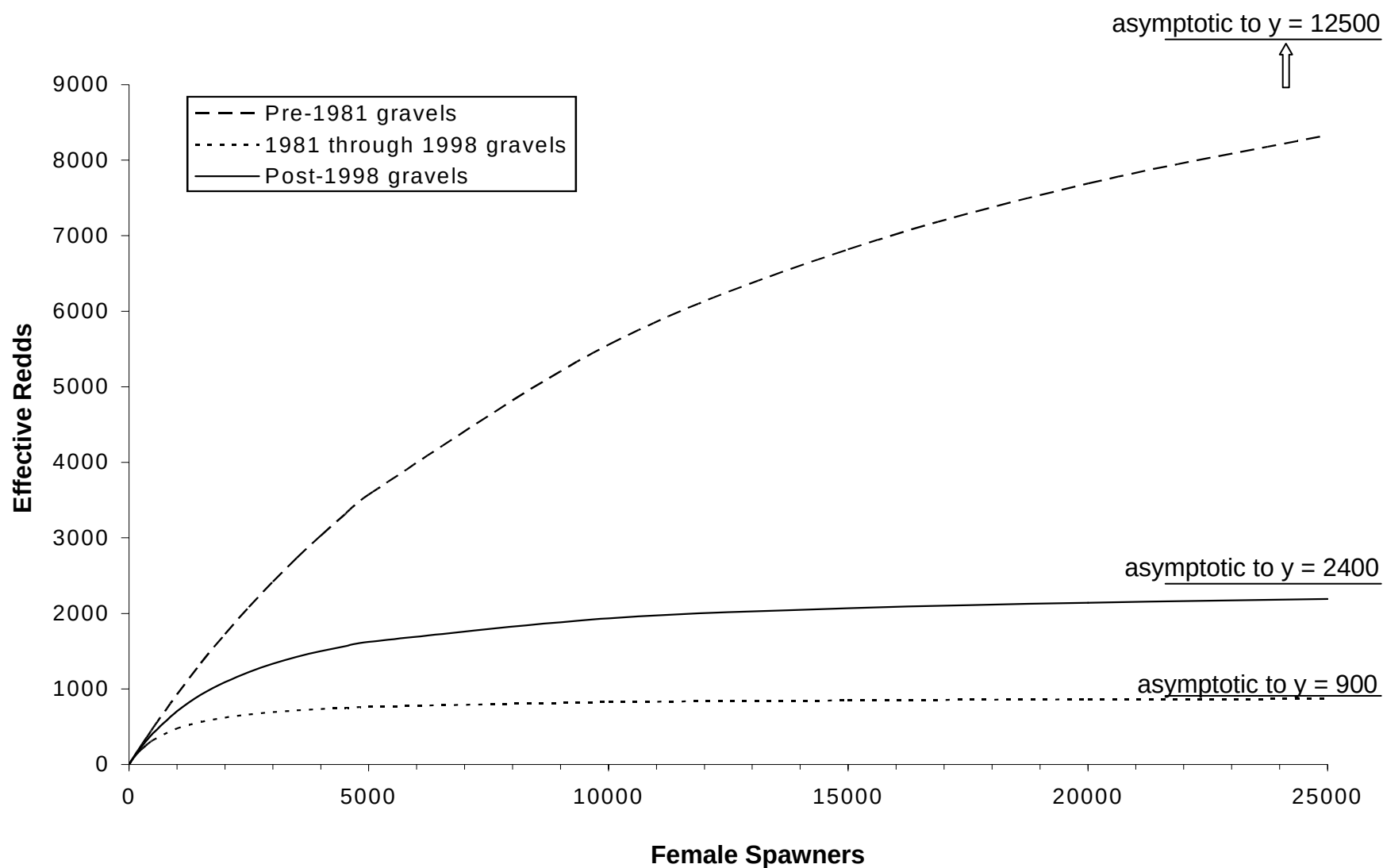
Figure 4.2-23. Number of effective redds, relative to the number of spawners. Effective redds are redds that are built and not superimposed.
