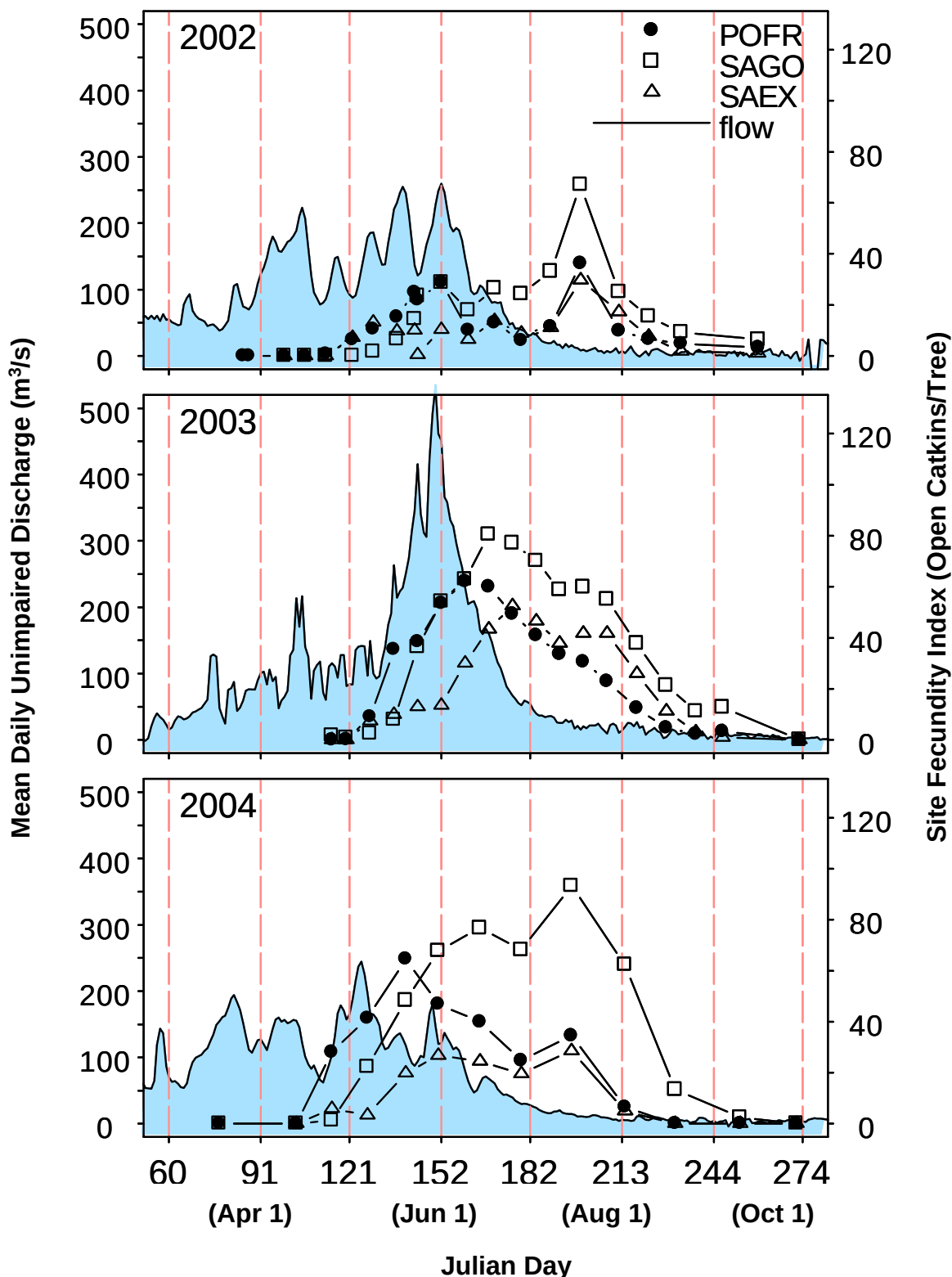
Figure 9-7. Patterns of seed release for Fremont cottonwood ( Populus fremontii = POFR), Goodding's willows ( Salix gooddingii = SAGO), and narrowleaf willow ( S. exigua = SAEX) along the Tuolumne River compared to unimpaired flow for three years. For all species, the annual fecundity index is calculated as mean per-tree open catkin count for all surveys; data from all sites are pooled. The hydrograph is computed unimpaired discharge at La Grange Dam (California Data Exchange Center, gauge TLG). Source: Stella et al. (in press).
