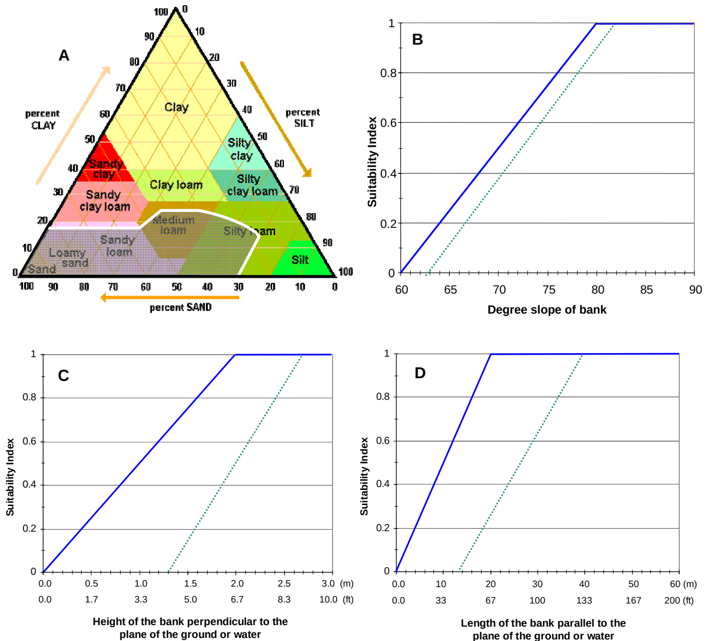
Figure 7-3a, b, c, d. Habitat suitability index (HSI) relationships for four key variables affecting bank swallow breeding habitat, based on the HSI model developed by Garrison (1989). Suitability values can range from unsuitable (0) to fully suitable (1). Solid lines indicate relationship proposed by Garrison (1989). Dashed lines indicate potential adjustments based on new interpretations (this report) of Sacramento River colony data collected by Garrison and others (1987). A. Soil textures suitable for nesting are represented by the shaded region in the lower left-center portion of the soil texture triangle (these soil types have suitability index = 1, all others = 0). B. Relationship between bank slope and suitability (near vertical banks have suitability = 1). C. Relationship of bank height above base flow water surface elevation during the nesting season to habitat suitability (taller banks have greater suitability). D. Habitat suitability increases with length of freshly eroded bank available.
