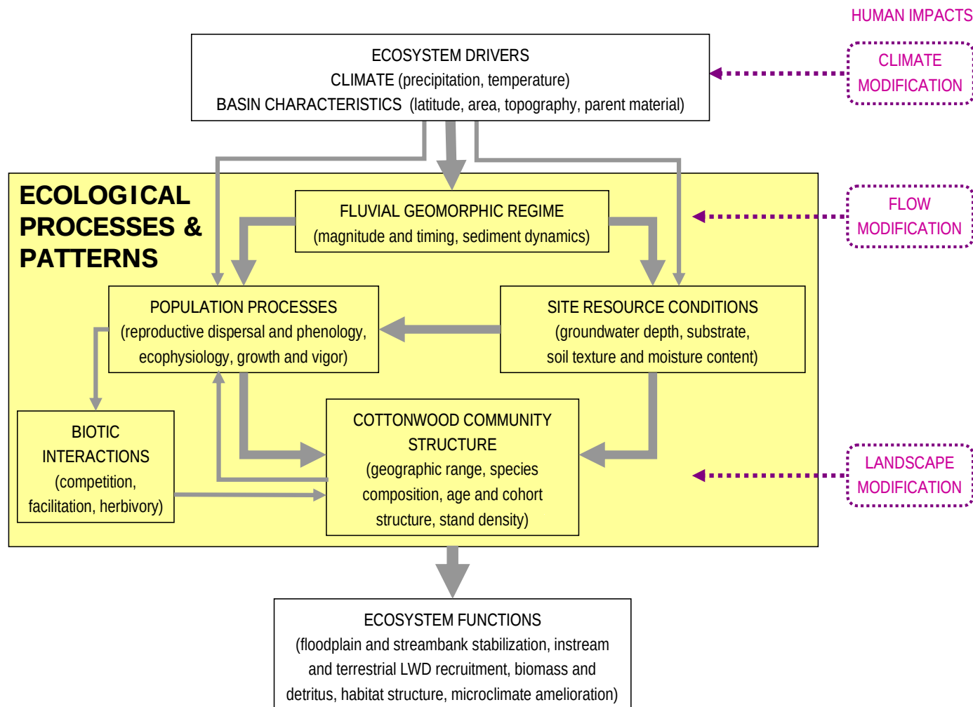
Figure 9-13. Conceptual model of natural and anthropogenic factors affecting the dynamics of cottonwood forest community development, structure, and ecosystem functioning in the middle Sacramento River corridor. Adapted from Battles et al. (2005), based on the framework developed by Strange et al. (1999).
