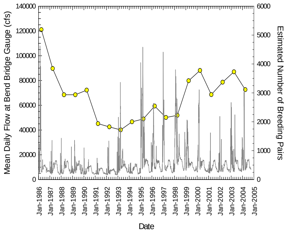
Figure 7-15. Mean daily flow at the Bend Bridge Gauge (gray line, left axis) at RM 258 and total estimated number of bank swallow breeding pairs (closed symbols, right axis) in (A) the Sacramento River as a whole and (B) Hamilton City to Red Bluff Reach (RM 200-243) during 1986-2004. Source: Hight 2000, Schlorff, 1997, 1998, 1999, 2000, 2001, 2002, 2003, 2004.
