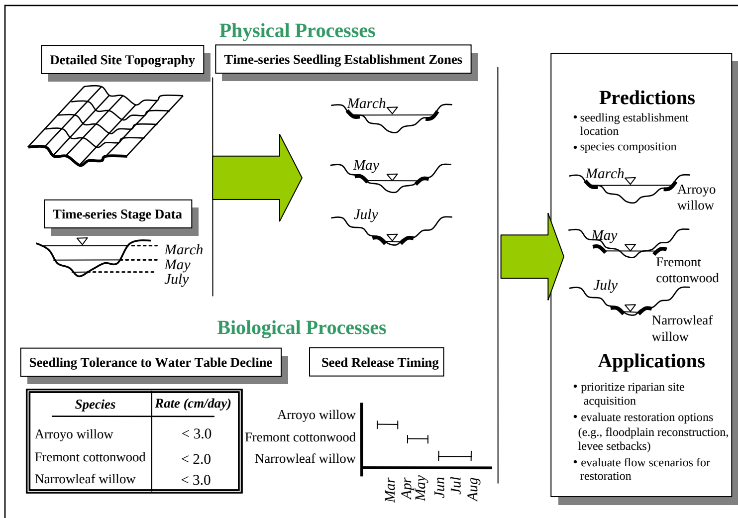
Figure 9-5. Framework for application of the recruitment box model to river corridor management and restoration.
