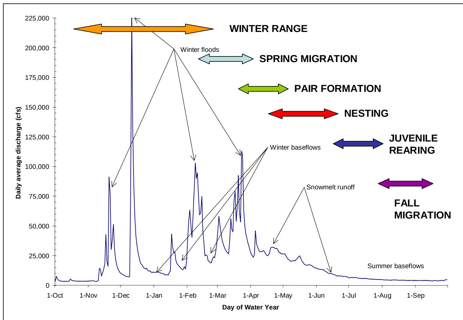
Figure 7-6. Representative annual hydrograph from the pre-Shasta period showing key hydrograph components relative to bank swallow life history stages: overwintering (orange), spring migration (light blue), pair bonding (green), nesting (red), juvenile rearing and local dispersal (dark blue), and fall migration (purple) periods. Hydrograph data are from the Bend Bridge Gage (near Red Bluff) for Water Year 1938 (CALFED 2000).
