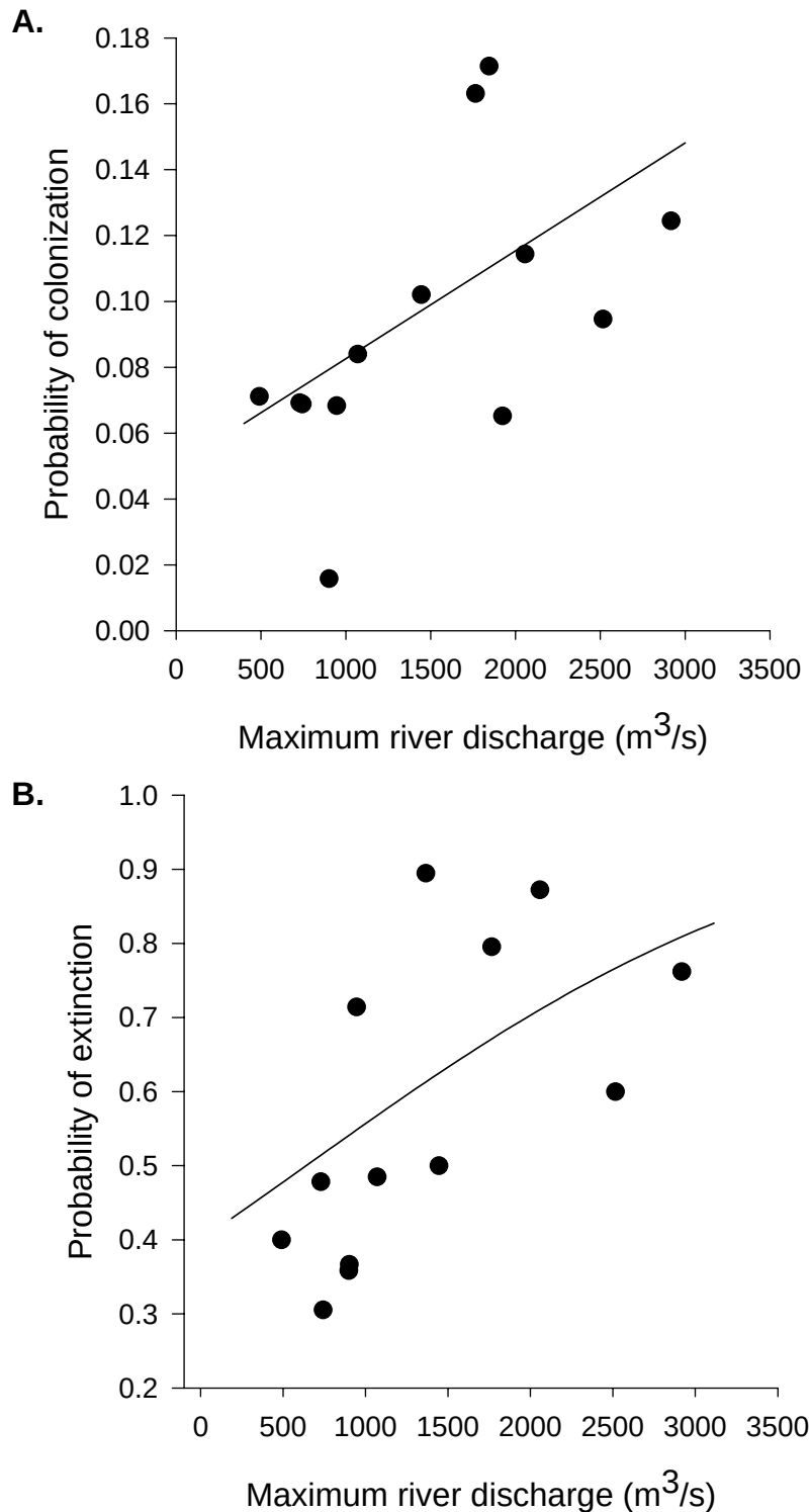
Figure 7-9. Relationship between maximum river discharge and (A) colonization rate and (B) extinction rate (Source: Figure 4 in Moffat et al. 2005). Data are yearly colonization and extinction probabilities from 1986-1992 and 1996-2003, calculated across all sites (i.e., the “temporal” analyses described in Moffat et al. 2005). Note: 1 cfs = 0.02832 \text{m}^3/\text{s} , and 1 \text{m}^3/\text{s} = 35.31 cfs.
