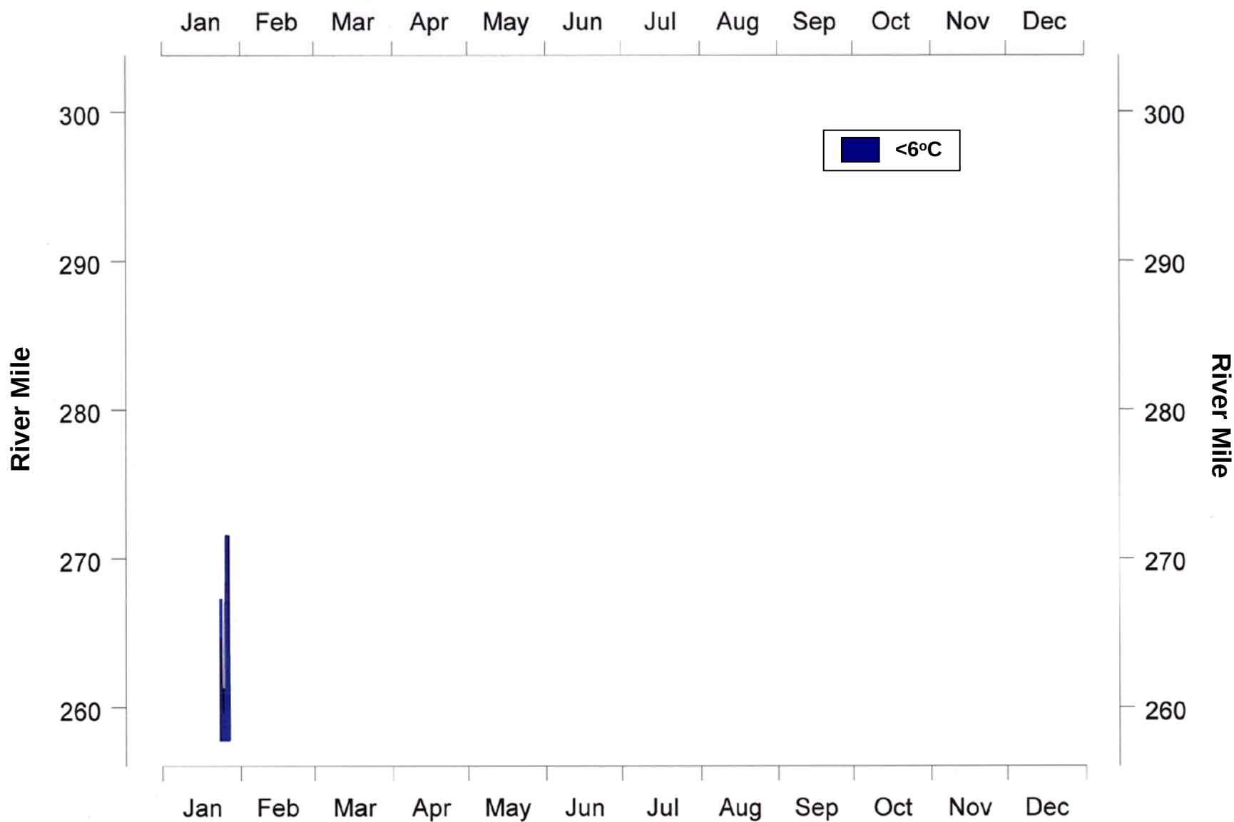
Figure 4.2-5. Example year (1972) where temperatures on the Sacramento River fall below 6°C.
