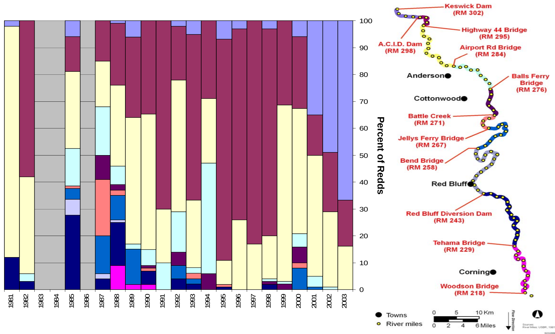
Figure 4.2-1. Redd distribution of winter-run Chinook salmon in the Sacramento River, as determined by DFG aerial redd surveys. Improvement in the fish passage facilities of ACID Dam (RM 298.4) in 2001 facilitated an upstream shift in the distribution of winter-run Chinook salmon spawning in the upper Sacramento River.
