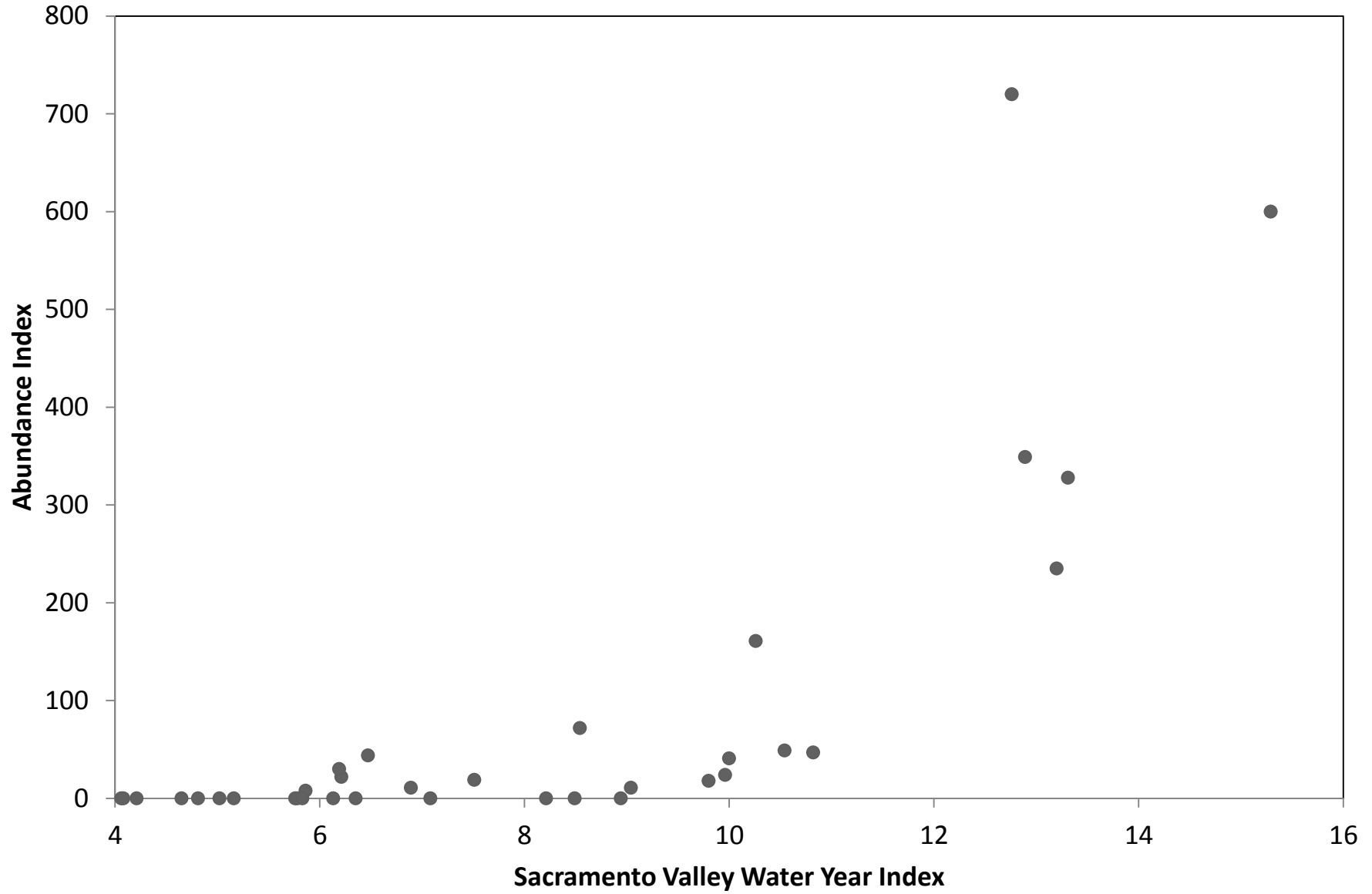
Sacramento Valley Water Year Index vs Annual Age-0 White Sturgeon Abundance Index From Bay Study Otter Trawl, 1980-2014
