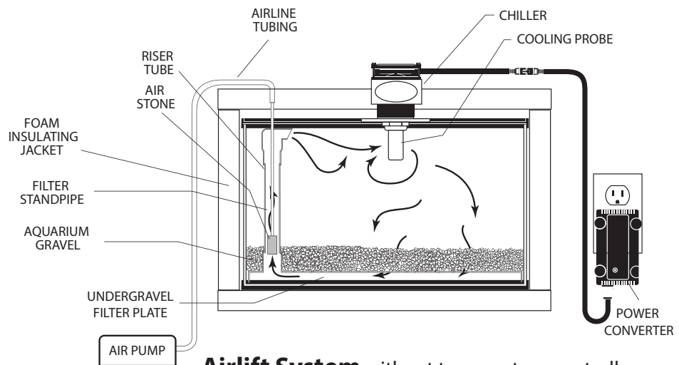
Airlift System without temperature controller
