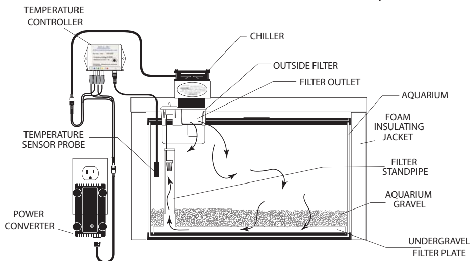
Outside Filter System with temperature controller (the chiller is mounted in the outside filter)
