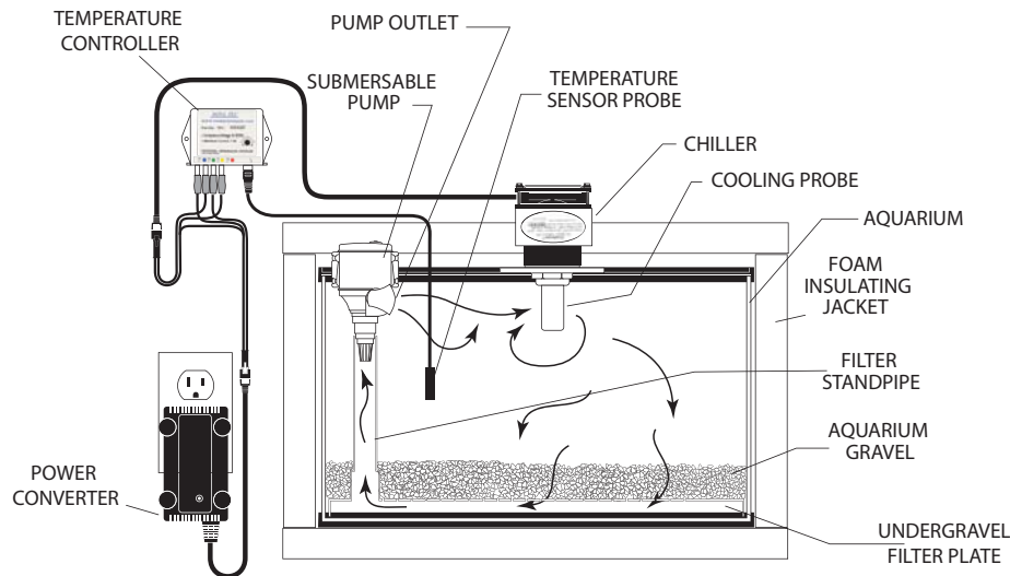
Electric Pump System with temperature controller
