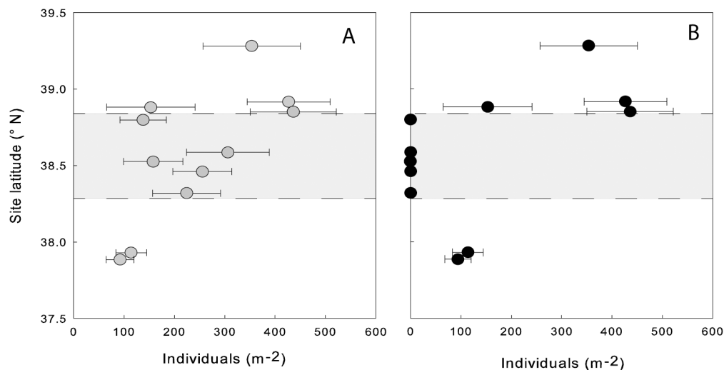
Fig 4. Densities of purple urchins (A) before and (B) after the mass mortality event, by latitude. Bars depict standard deviation across sampled quadrats. Data are from the 11 sites surveyed between September and December 2011 (sites 1–4, 6, 10, 14, 16, 18, 23, 24). The shaded area denotes the impacted region, in which we found zero individuals at all sites surveyed after the event ( n = 5 ).
