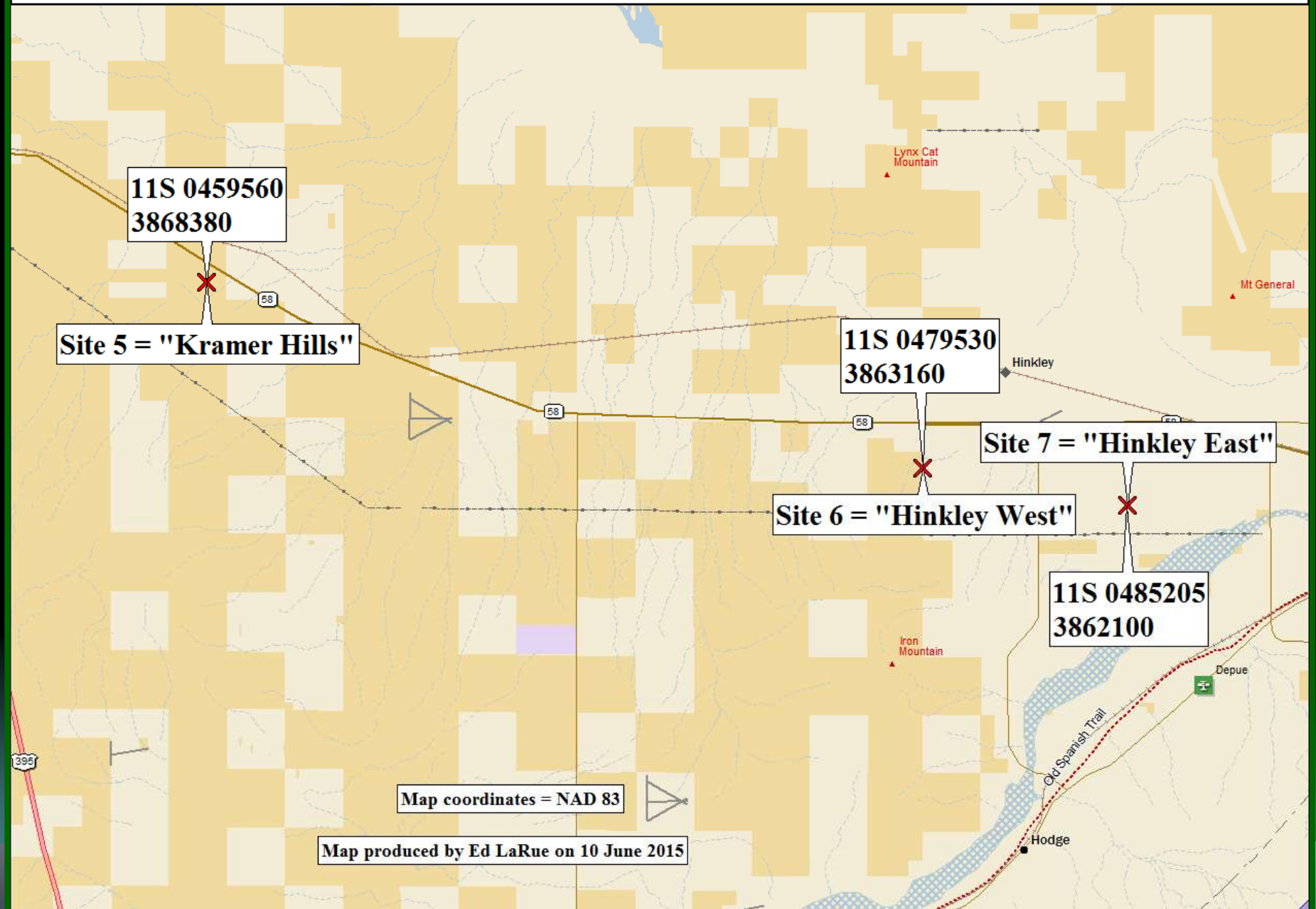
Figure 1c. Three PG&E Sites in 2015
