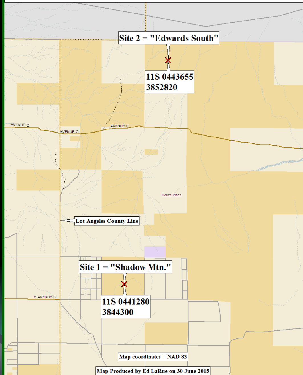
Figure 1a. Two Sites Trapped near L.A. County Line in 2015
