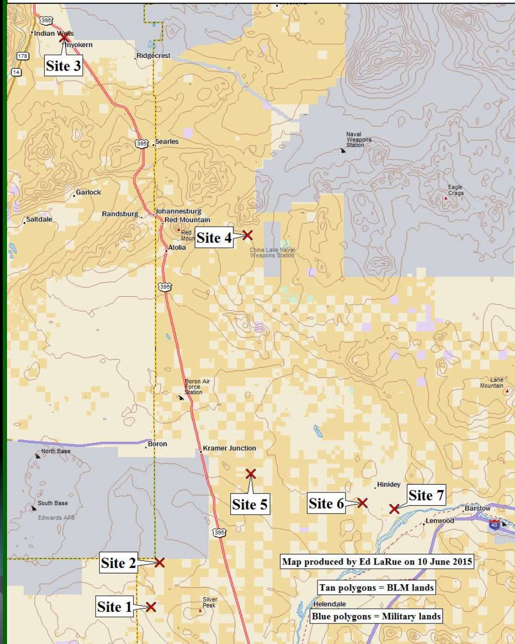
Figure 1. Seven Sites Trapped for Mohave Ground Squirrel in 2015
