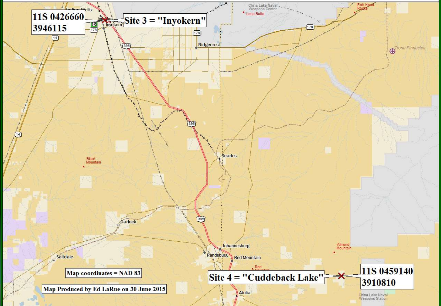
Figure 1b. Two Northwestern Sites Trapped in 2015
