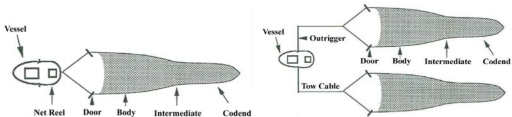
Figure 2-3. Diagrams of (left) a single-rigged vessel pulling one otter trawl, and (right) a double-rigged vessel pulling two otter trawls used on Pink Shrimp vessels (Reproduced from Jones et al. 1996).
