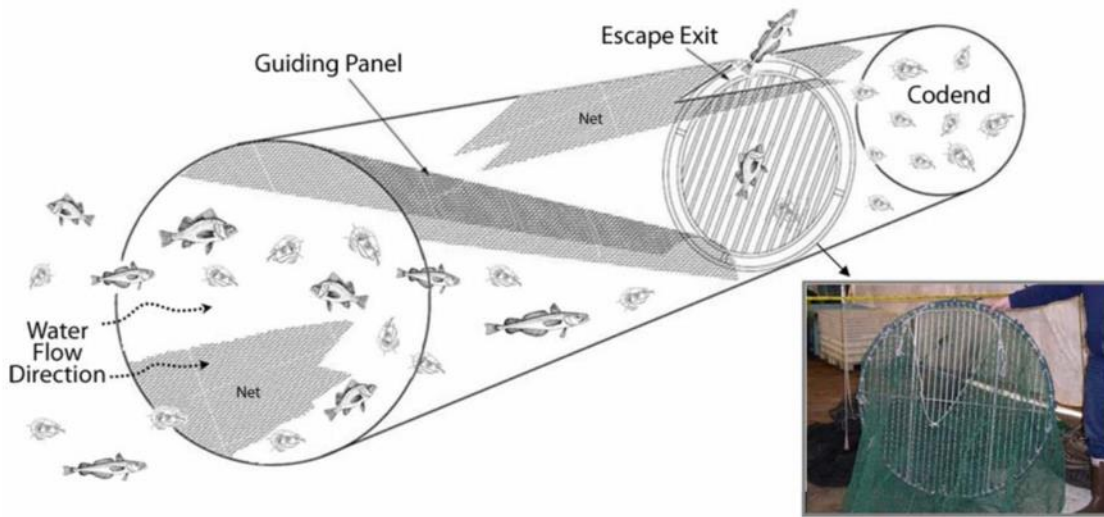
Figure 2-4. Diagram of a rigid-grate Bycatch Reduction Device used in the Pink Shrimp fishery. The diagram depicts shrimp traveling through the BRD, and larger fish being deflected by the BRD and guided through the escape hatch (Photo Credit: Robert Hannah, ODFW).
