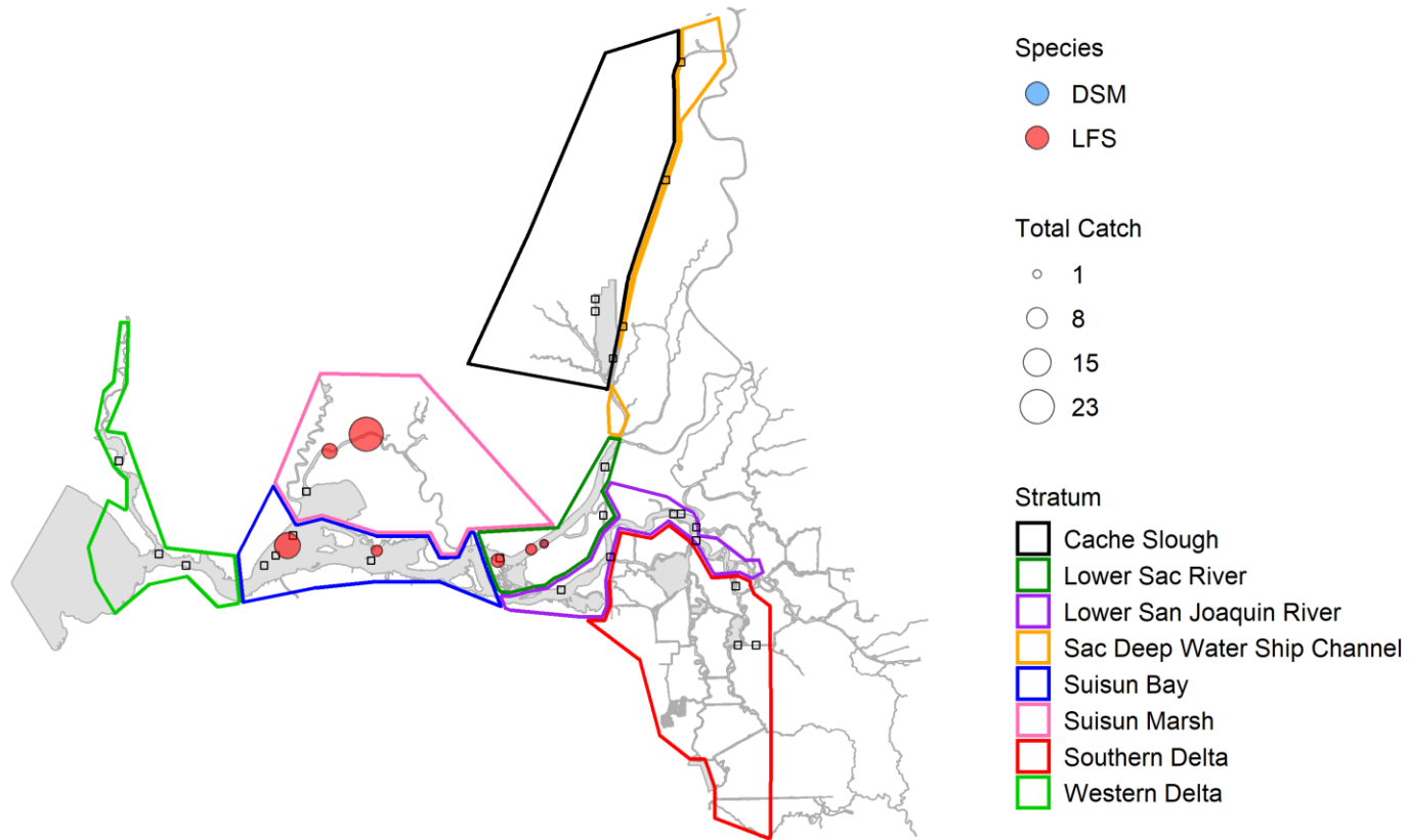
Figure 1. Delta Smelt (DSM) and Longfin Smelt (LFS) catch per station for EDSM 2022 Phase 1 Kodiak trawls, from 1/24/2022–1/28/2022. Sites with no DSM or LFS catch are indicated with squares.
