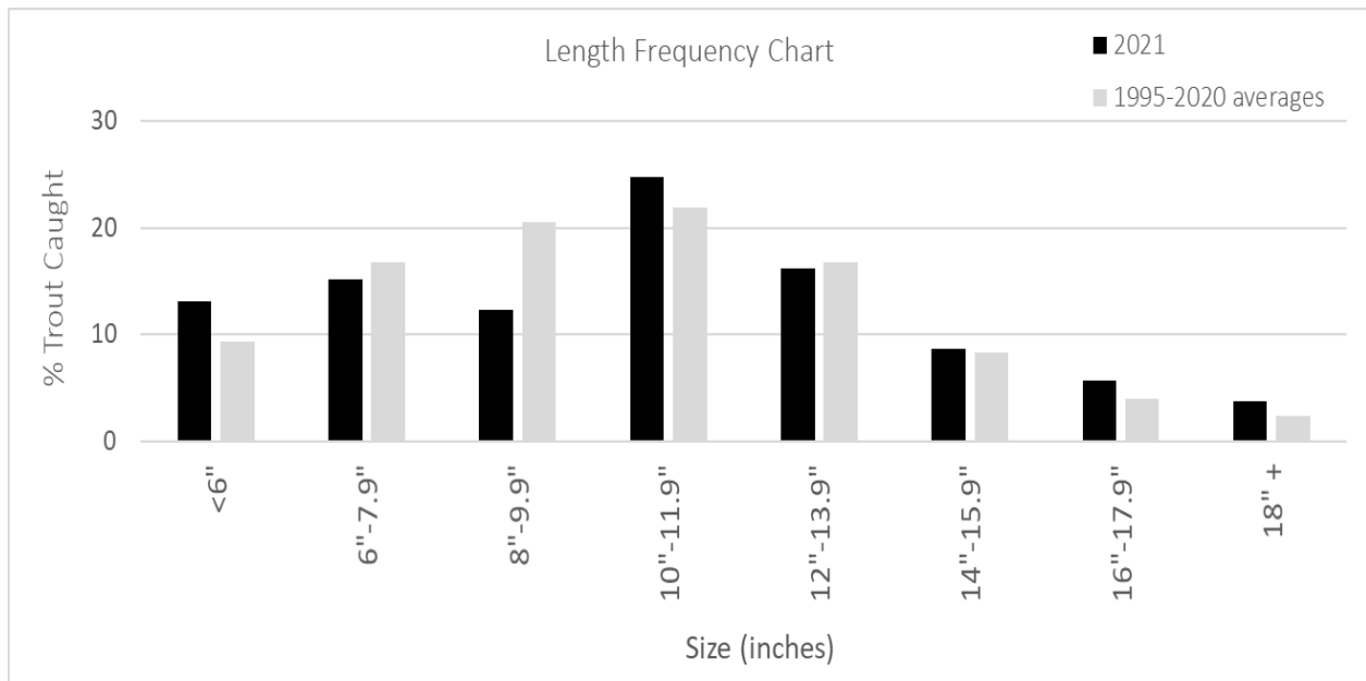
Figure 1. Chart showing distribution of size classes captured from 1995-2021.
