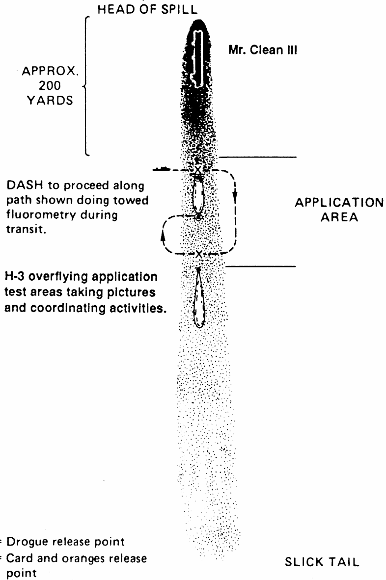
Figure 3. Idealized representation of vessel movements for the Dash and Mr. Clean III (response vessels) after dispersant application to the surfacing PAC Baroness oil assuming a wind direction parallel with the current-controlled slick drift (see Figure 2) (from Payne et al. 1991c).
