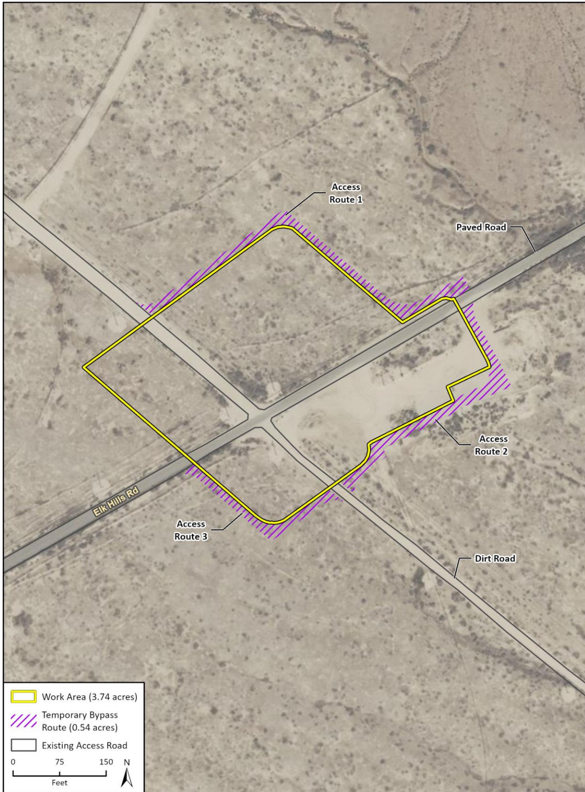
Figure 2 Work Area and Access Routes
