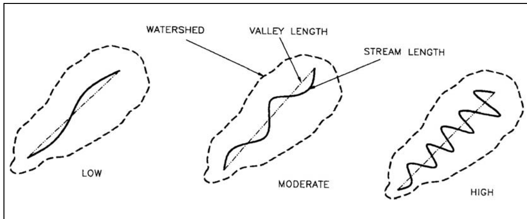
Figure III-3. Sinuosity.
