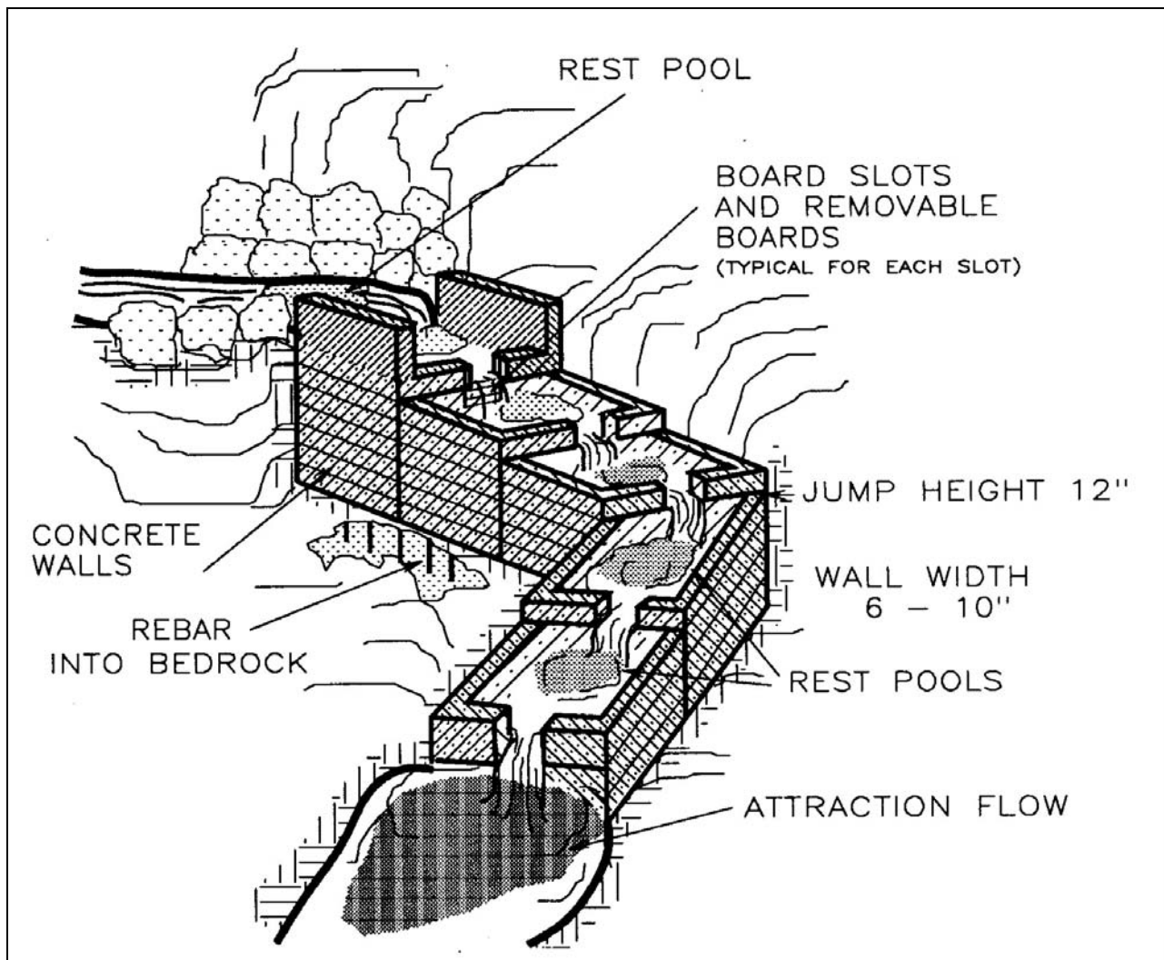
Figure VII-39. Step-and-pool fishway.
