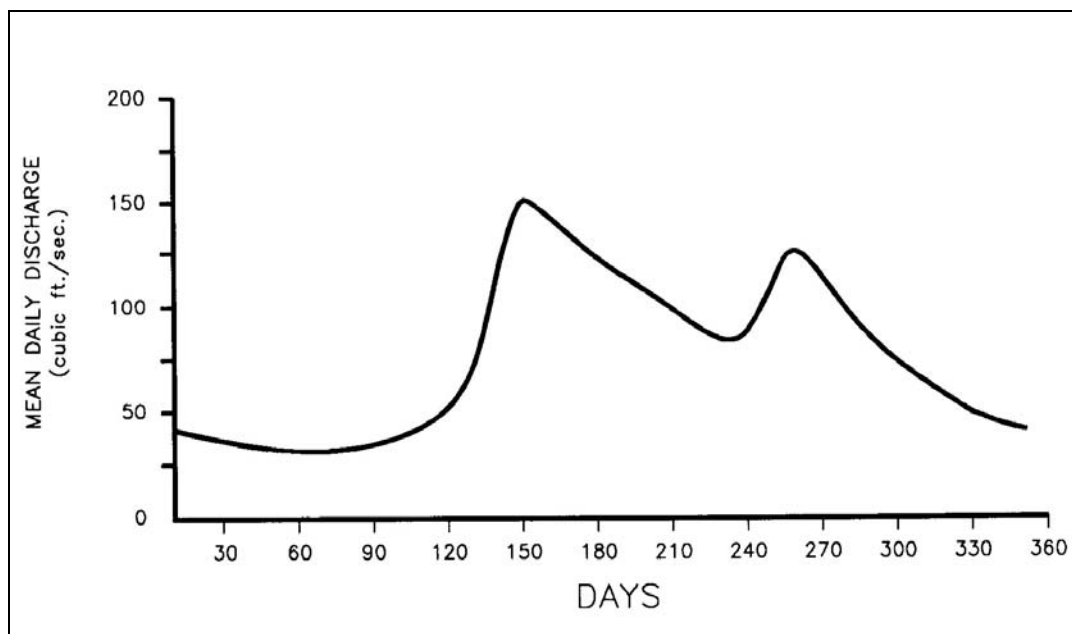
Figure II-4. Hydrograph.
