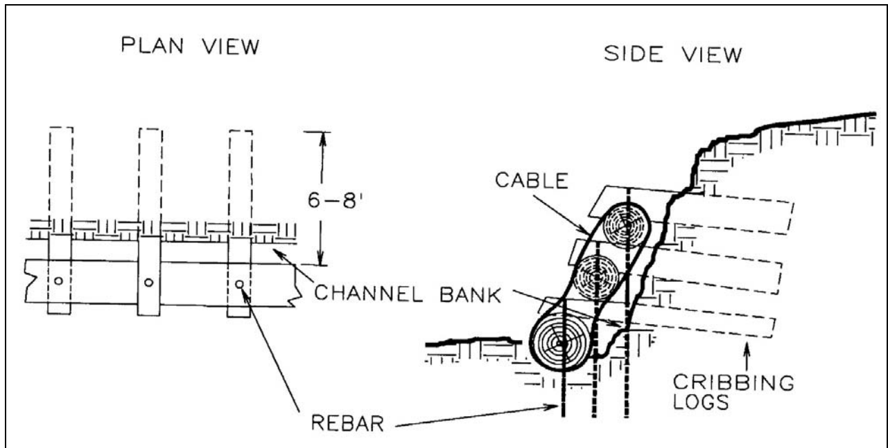
Figure VII-50. Log cribbing.
