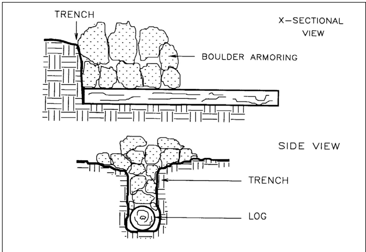
Figure VII-15. Trenching.
