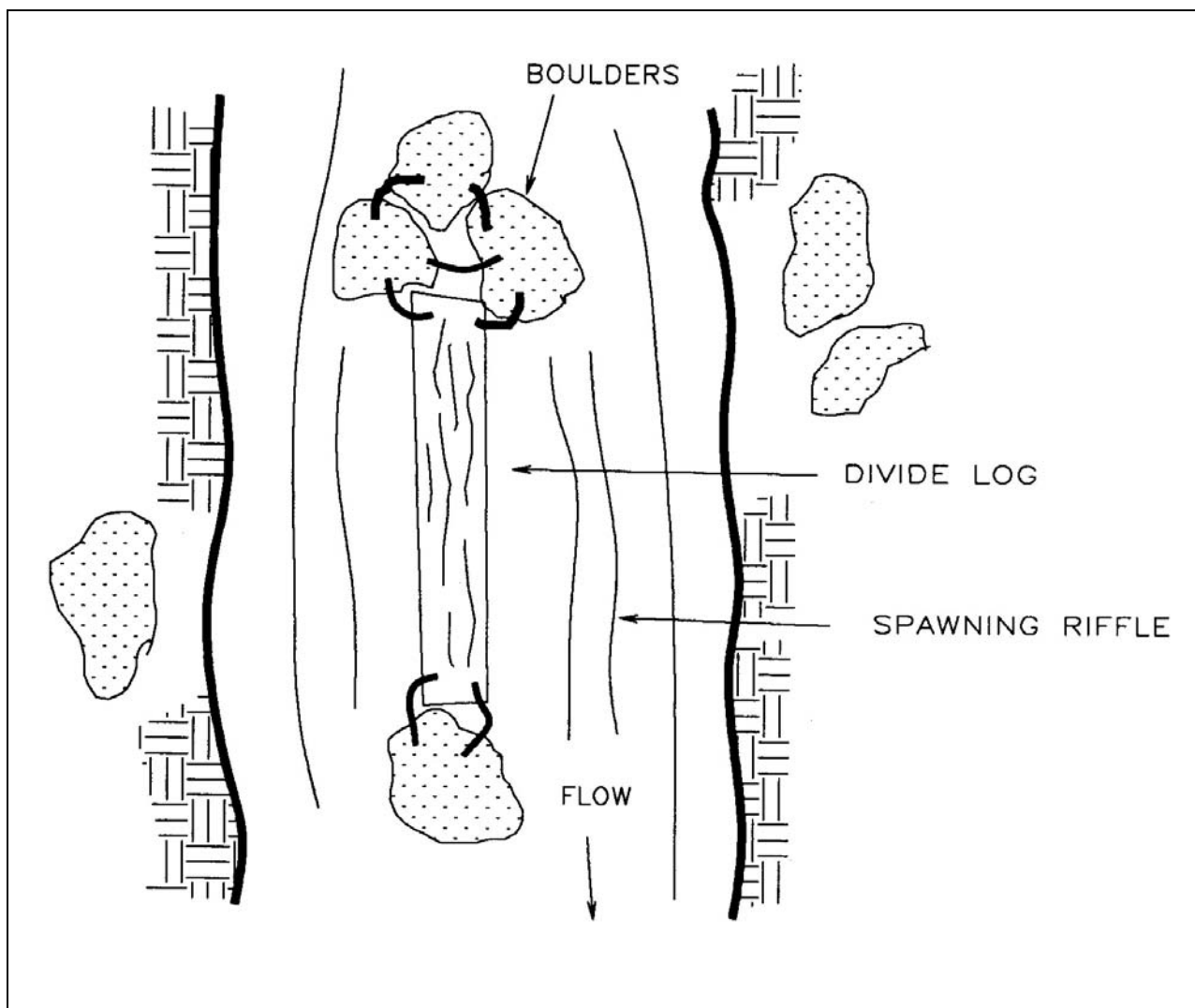
Figure VII-17. Divide log.
