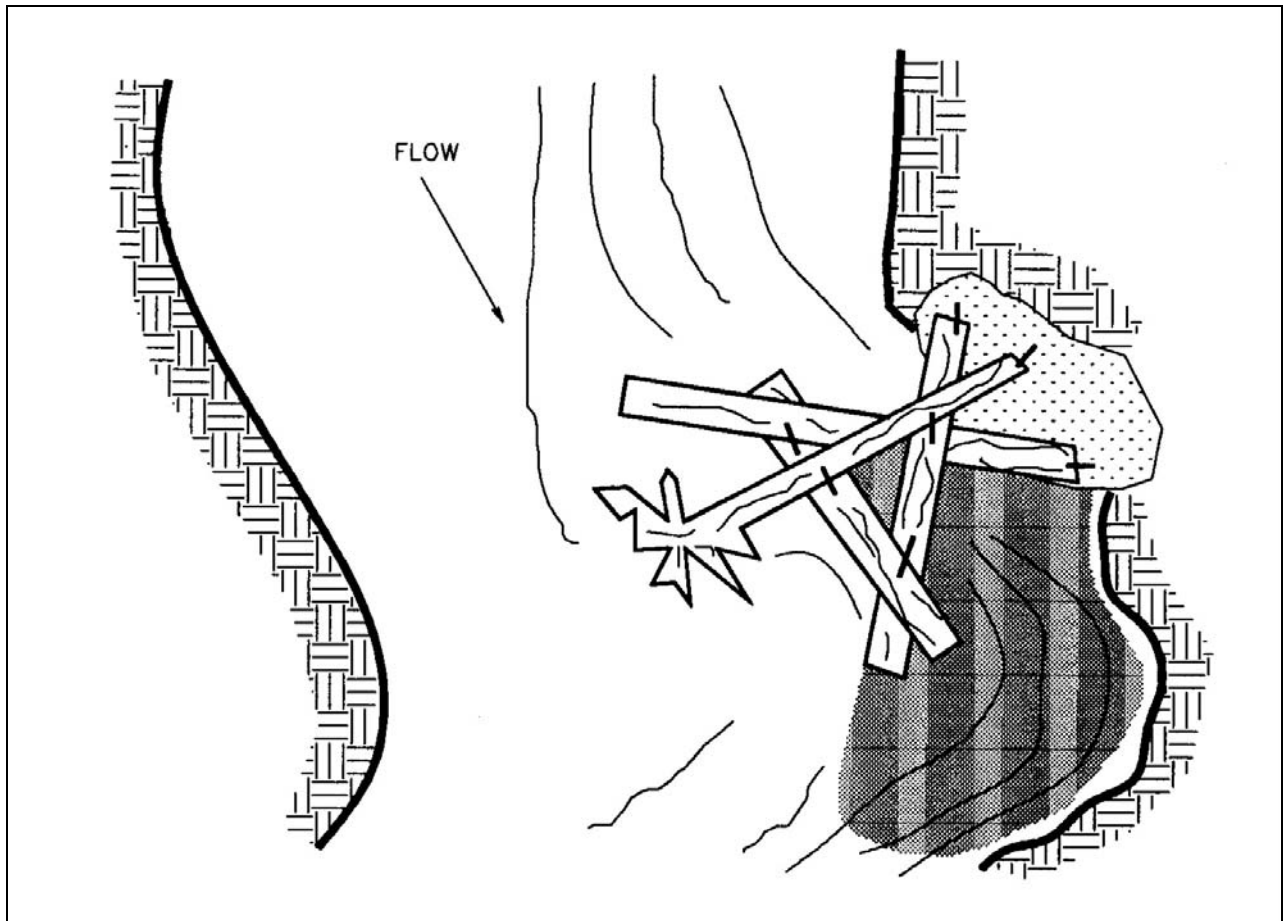
Figure VII-19. Spider logs.
