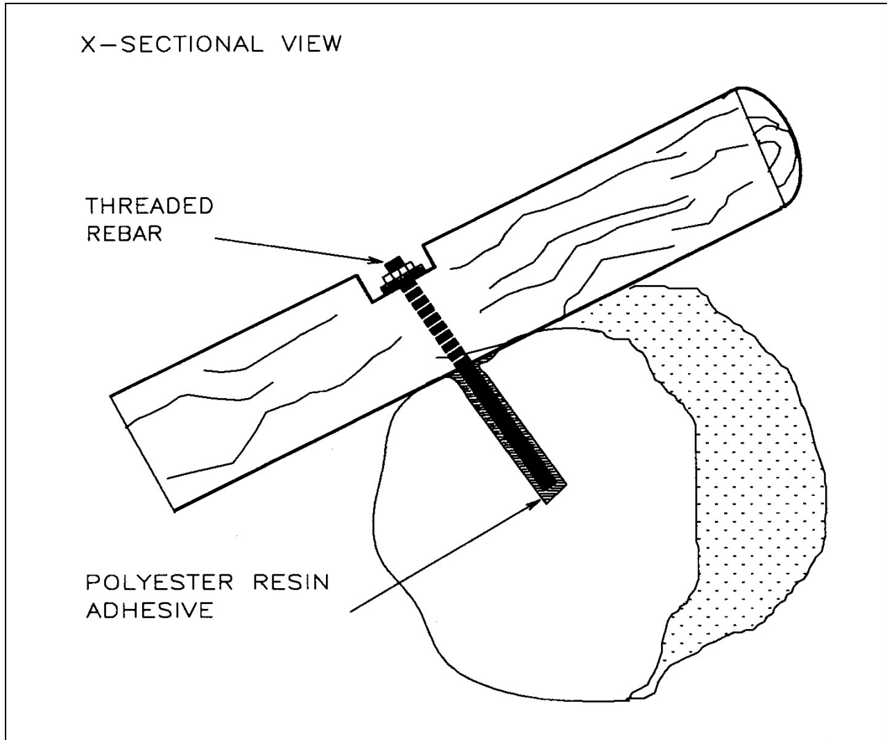
Figure VII-12. Threaded rebar anchoring log to boulder, using polyester resin adhesive.
