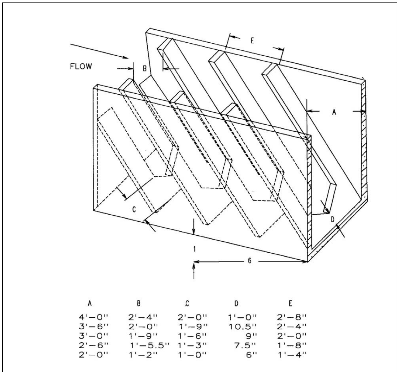
Figure VII-40. Denil fishway.
