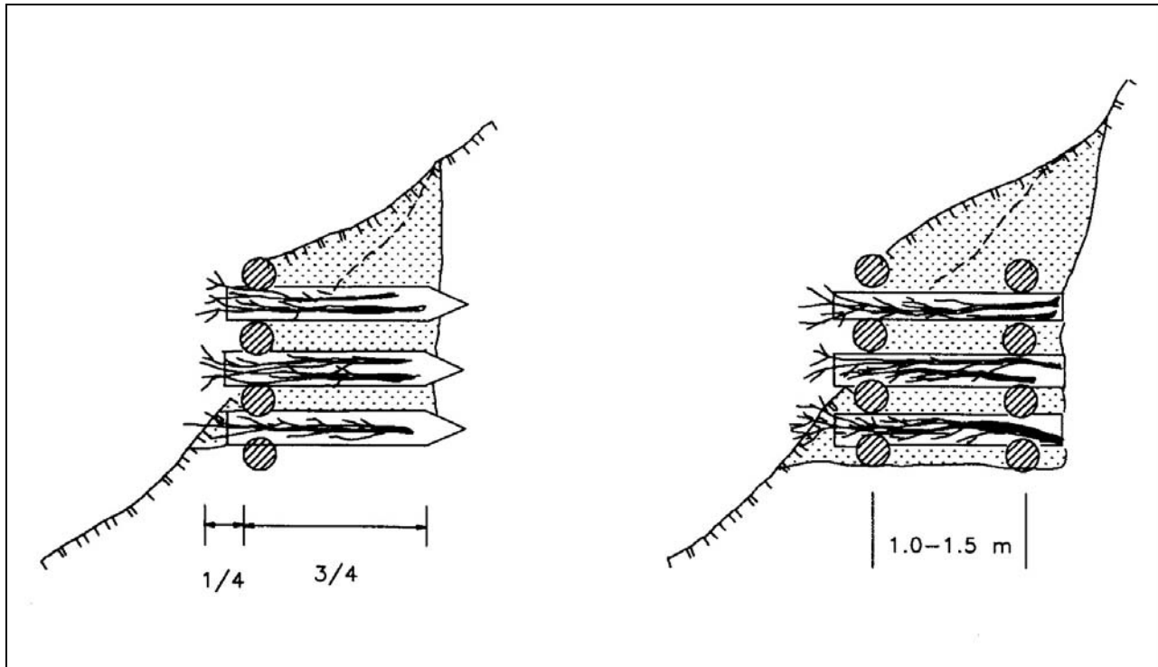
Figure VII-51. Live Vegetated Crib Wall (Schiechl and Stern, 1996)
