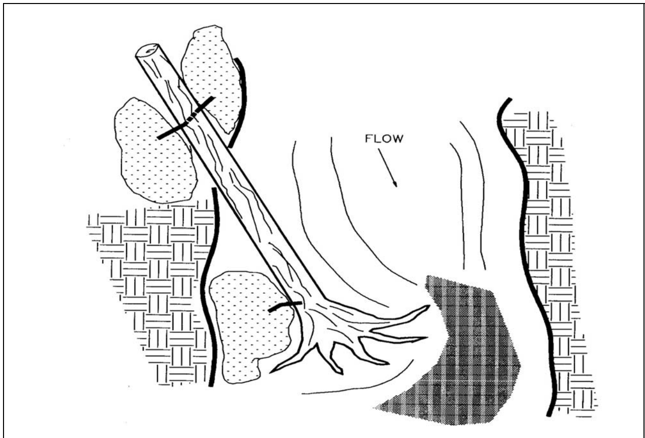
Figure VII-18. Digger log.
