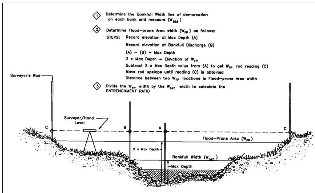
Figure III-7. Entrenchment determination.
