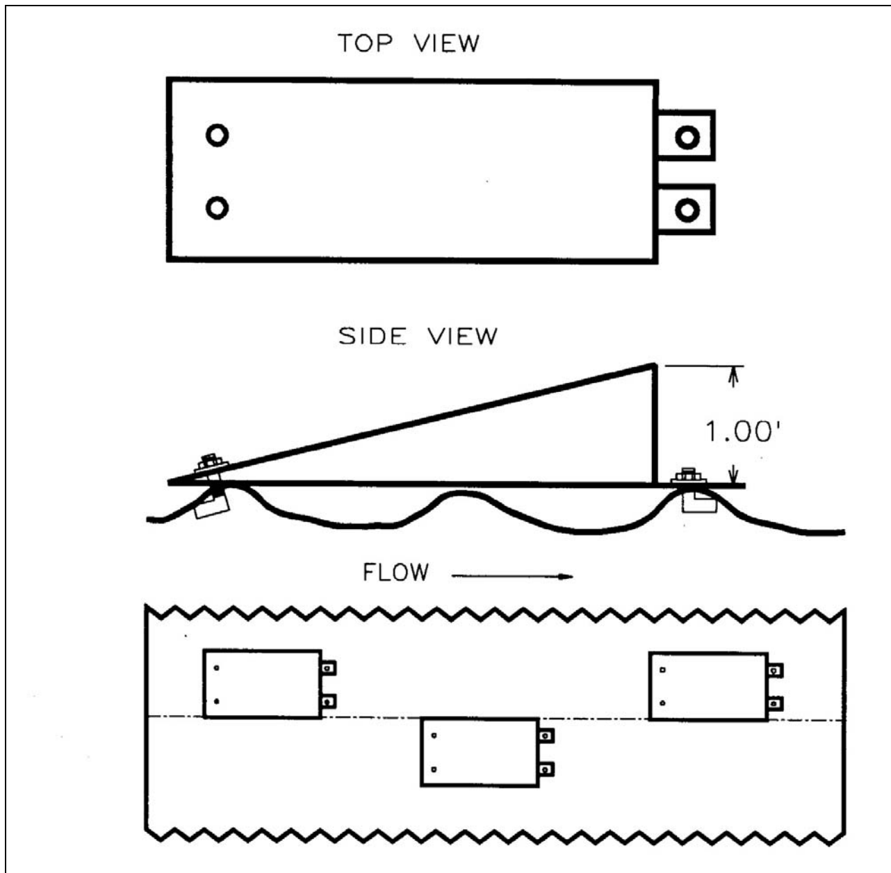
Figure VII-47. Corrugated metal pipe steel ramp baffles.
