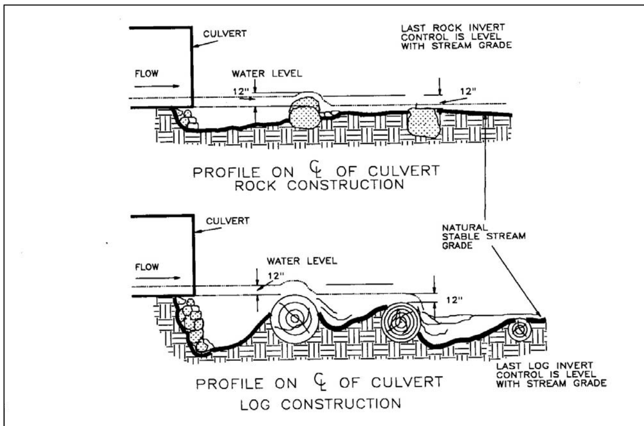
Figure VII-42. Back-flooding weirs.
