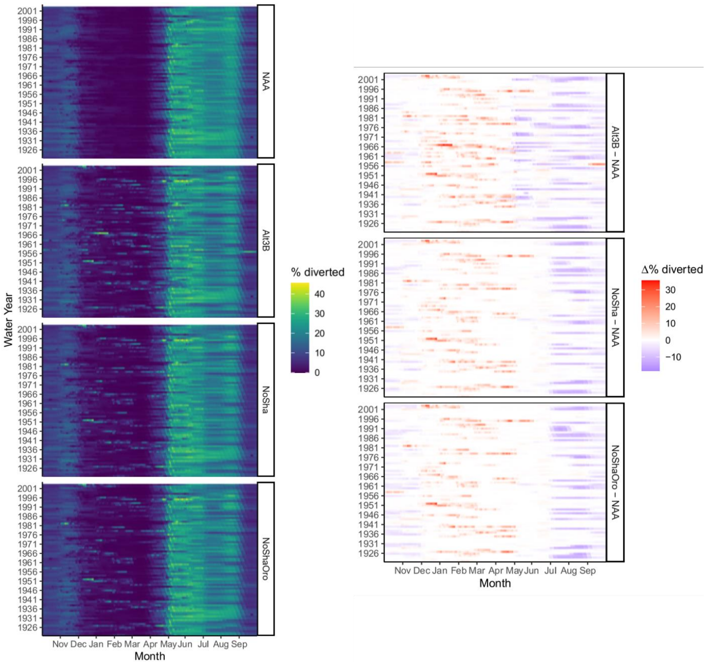
Figure 4-30. (left) Upper Sacramento River Daily Operations Model (USRDOM) simulated daily percentage of Sacramento River flow diverted by the Hamilton City Pump Station under (top to bottom) the No Action Alternative (NAA), Alt3B, NoSha, and NoShaOro during water years 1922 – 2003. Color brightness indicates percent diverted. The differences in percent diverted between Alt3B and NAA, NoSha and NAA, and NoShaOro operational scenarios and NAA are shown on the right from top to bottom, respectively. Red shades indicate positive differences (Project > NAA), while blue shades indicate negative differences (Project < NAA). USRDOM data provided by Sites Authority (2023).
