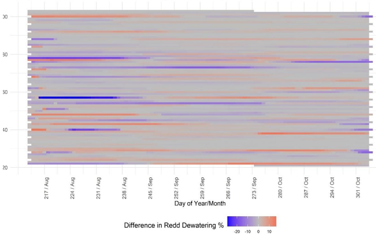
Figure 4-71. Heatmap showing the percent (%) change in daily potential for redd dewatering for spring-run Chinook Salmon (i.e., redds built during the months of August-October) for the Alt3B operational scenario compared to the NAA for Water Years 1922-2003.
