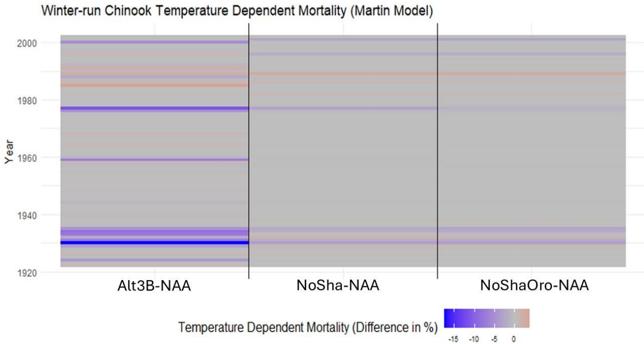
Figure 4-68. A heatmap showing the difference in winter-run Chinook Salmon redd temperature dependent mortality for water years 1922-2003 using HEC5Q Sacramento River Temperatures and Martin model parameters. Each operational scenario (i.e. Alt3B, NoSha, NoShaoOro) is shown as a difference to the No Action Alternative (NAA).
