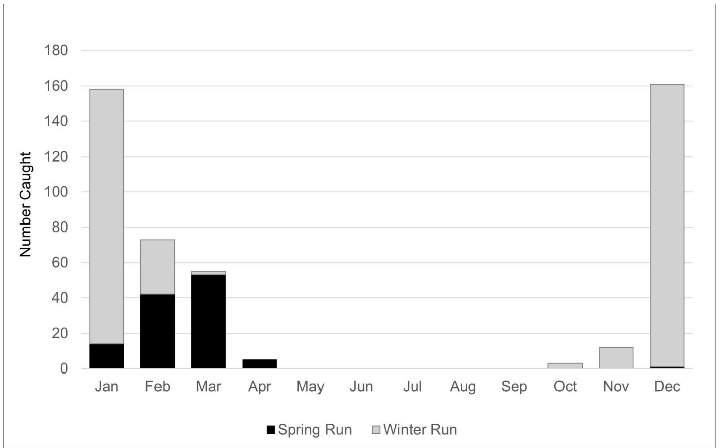
Figure 3-3. Juvenile spring-run and winter-run Chinook Salmon catch by month in the USFWS Delta Juvenile Fish Monitoring Program beach seine sampling at Knights Landing Boat Ramp, 2005–2017.
