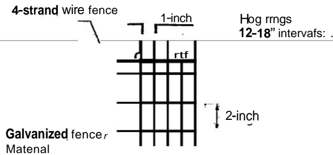
DETAIL B
