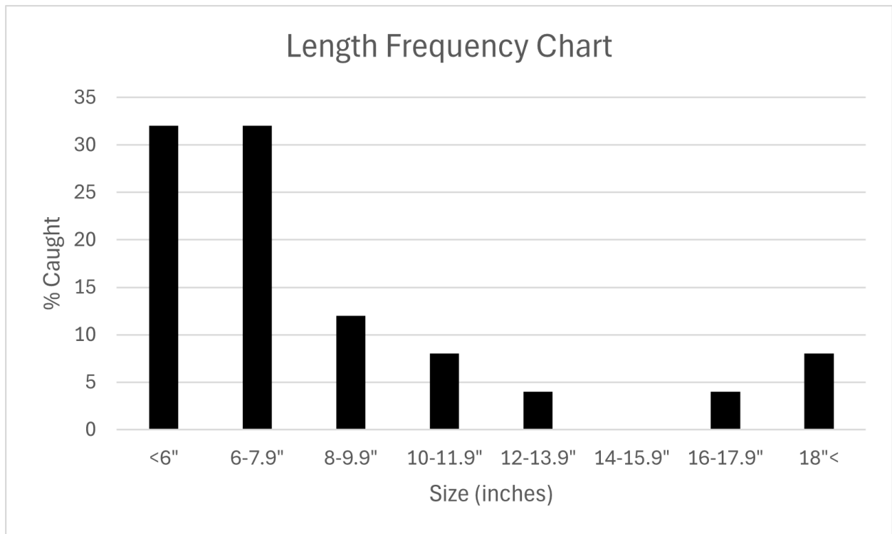
Figure 1. Histogram showing distribution of size classes captured from 2023.
