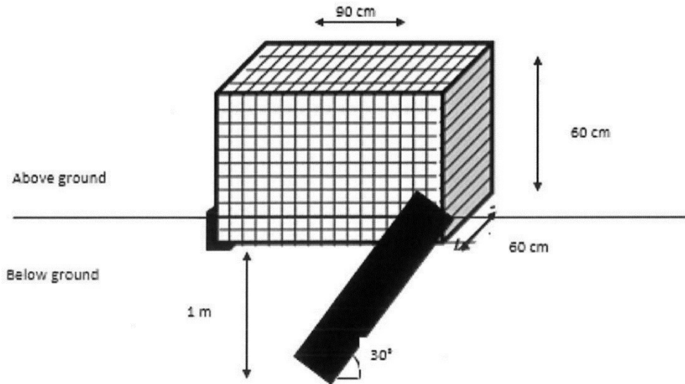
Figure 2. SBKR retention cage (Condition of Approval 7.9.1).
