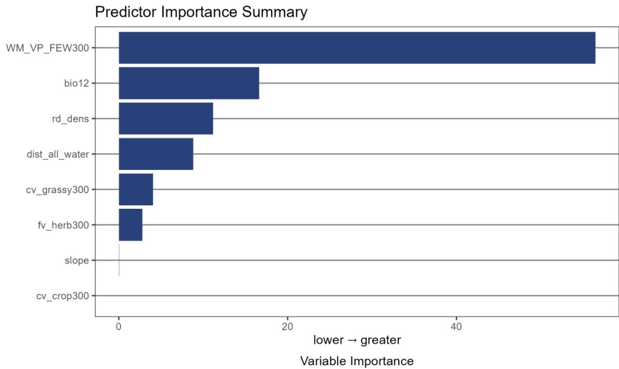
Figure 1. Estimates of the relative percent of contributions (variable importance %) of covariate inputs to the top Maxent model. Covariates are defined in Table 4.
