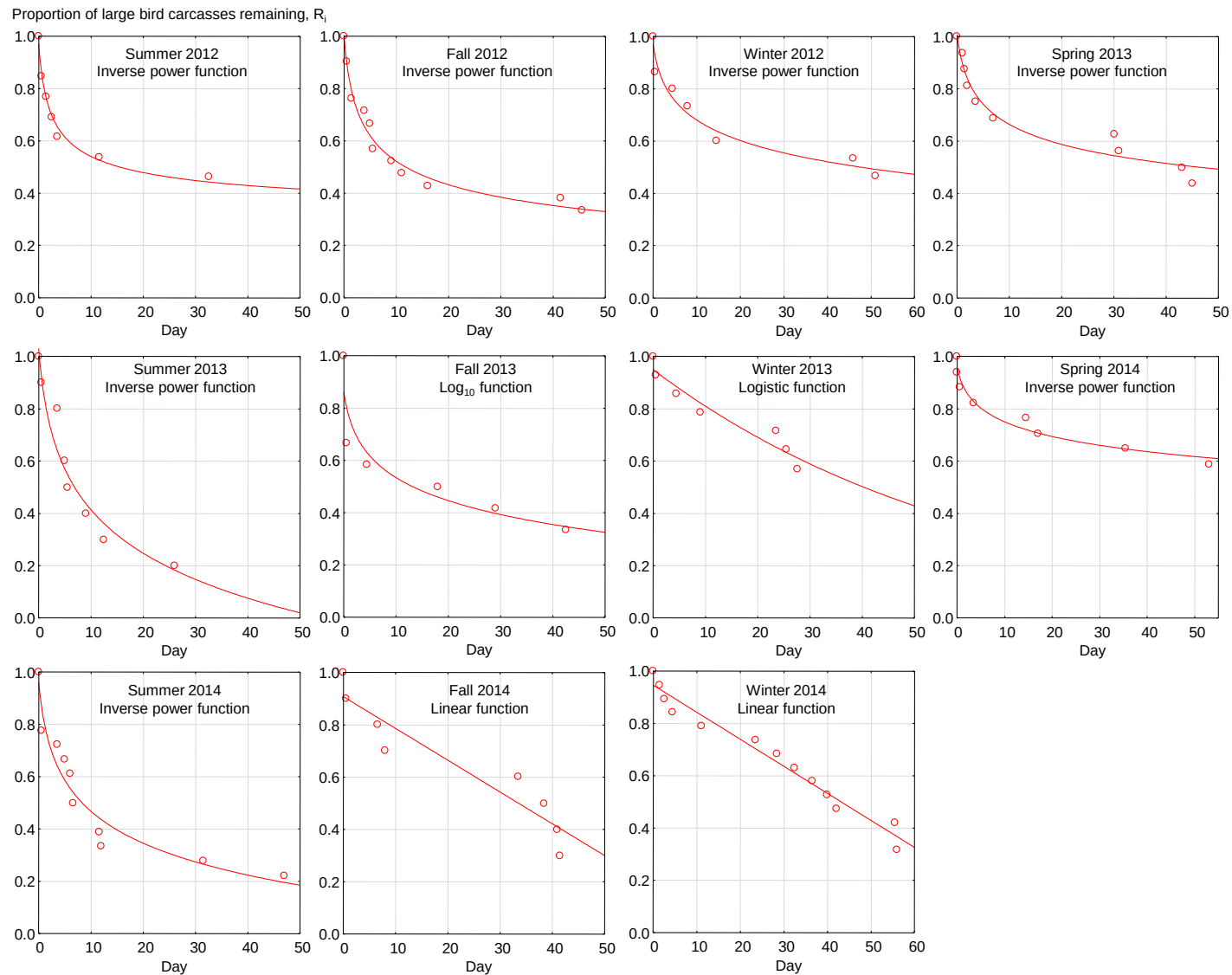
Figure 19. Seasonal carcass persistence patterns for large ( \geq 280g ) birds placed in trials over 3 years in the Vasco Winds Energy Project. Although trials lasted ca. 60 days, only 50 days of trial time are graphed to show patterns of data around the search intervals of 7 and 28 days.
