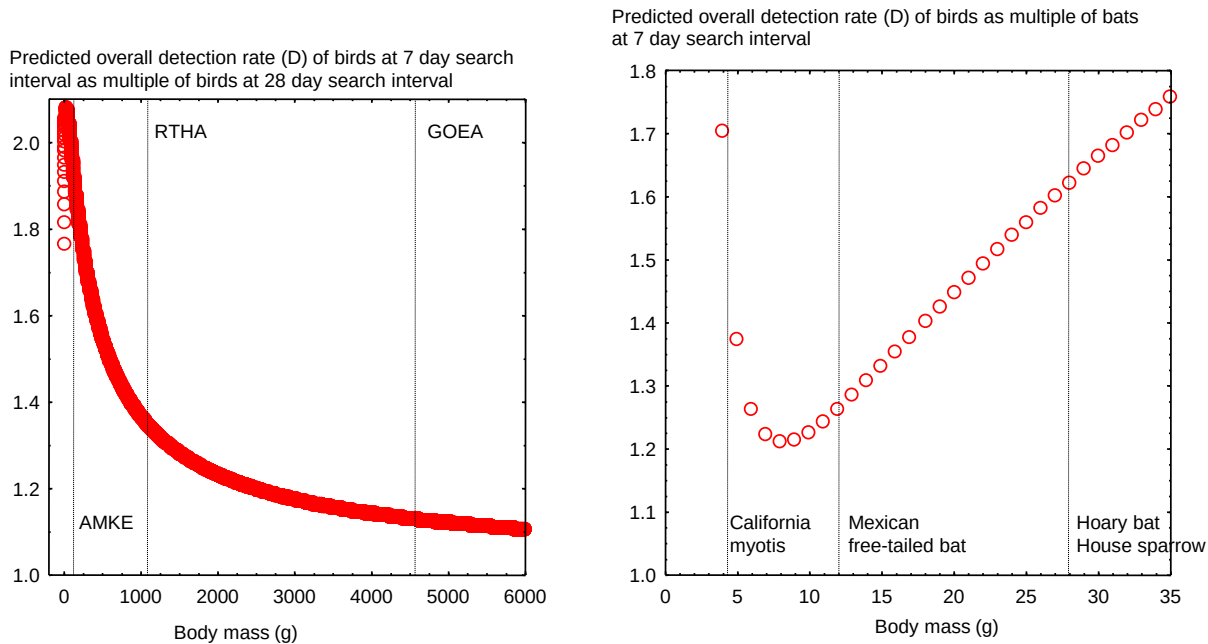
Figure 27. After projecting the logistic models of overall detection rates to bird and bat species of North America, and except for the smallest body masses, the ratio of predicted overall detection rates at turbines searched every 7 days to every 28 days declined with increasing body mass of bird species (left graph), and the ratio of predicted overall detection rates of birds to bats increased with increasing body mass (right graph). Vertical lines correspond with body masses typical of American kestrel (AMKE), red-tailed hawk (RTHA), golden eagle (GOEA), California myotis, Mexican free-tailed bat, and hoary bat and house sparrow.
