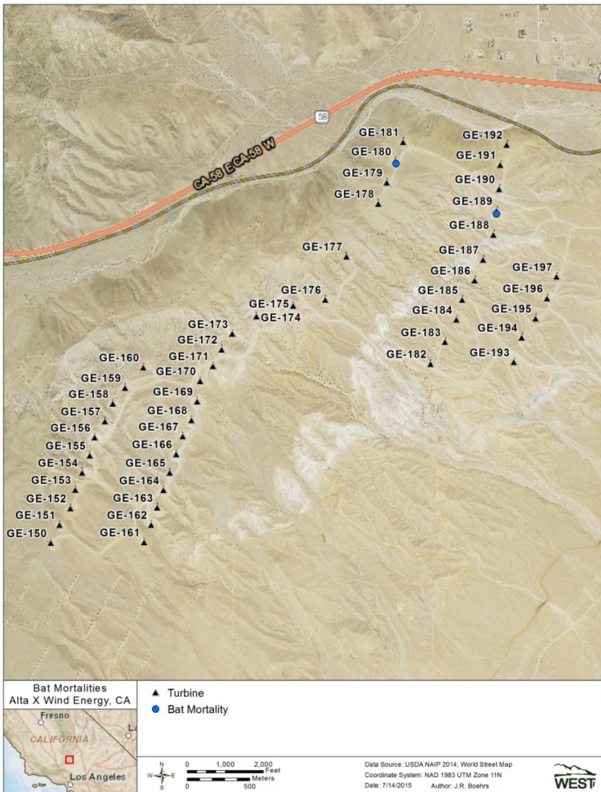
Figure 3b. Location of all bat mortalities found at the Alta X Wind Energy Project.
