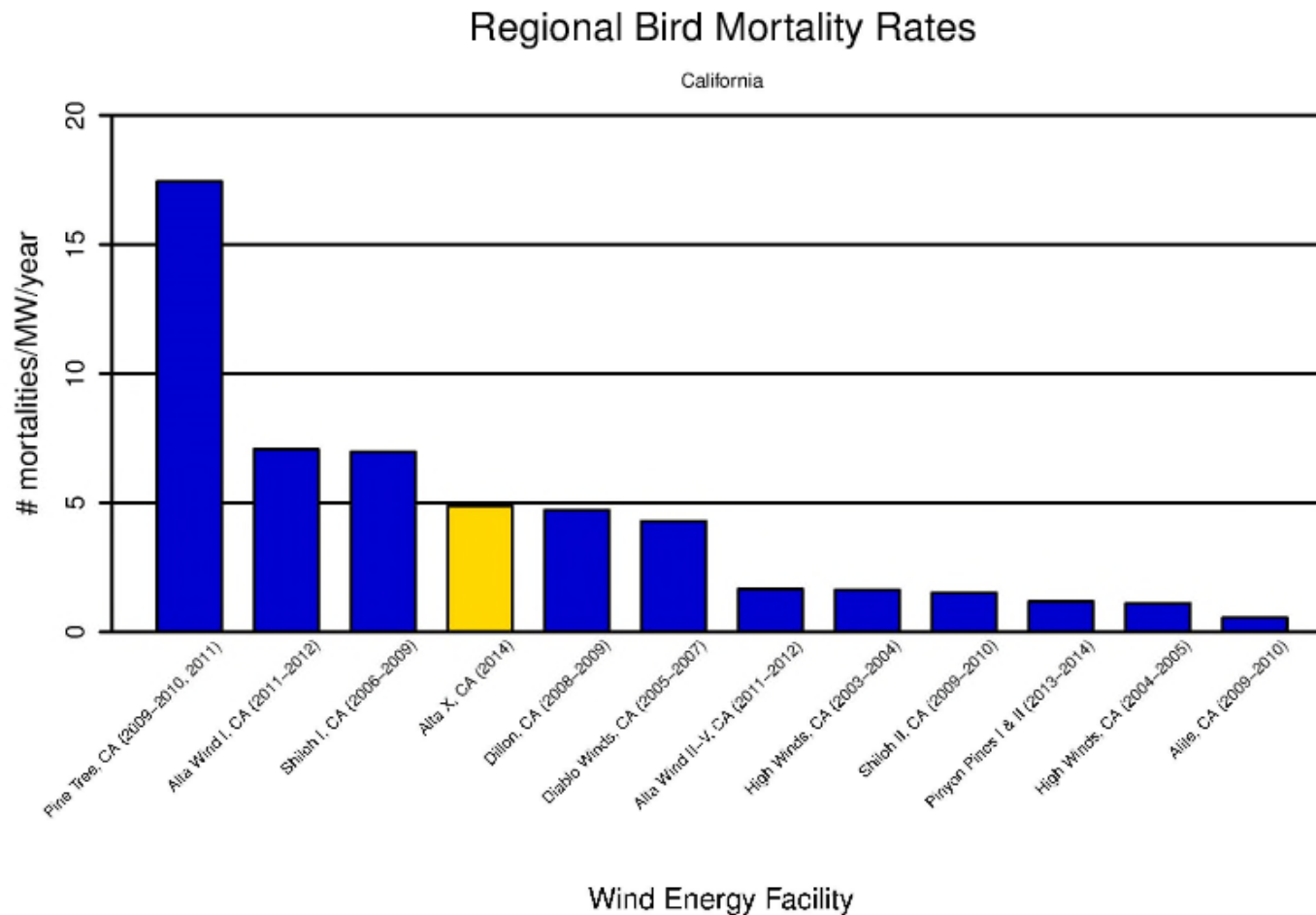
Figure 8. Mortality rates for all birds (number of birds per MW per year) at the Alta X Wind Energy Project compared with publicly-available studies at wind energy facilities in California.
