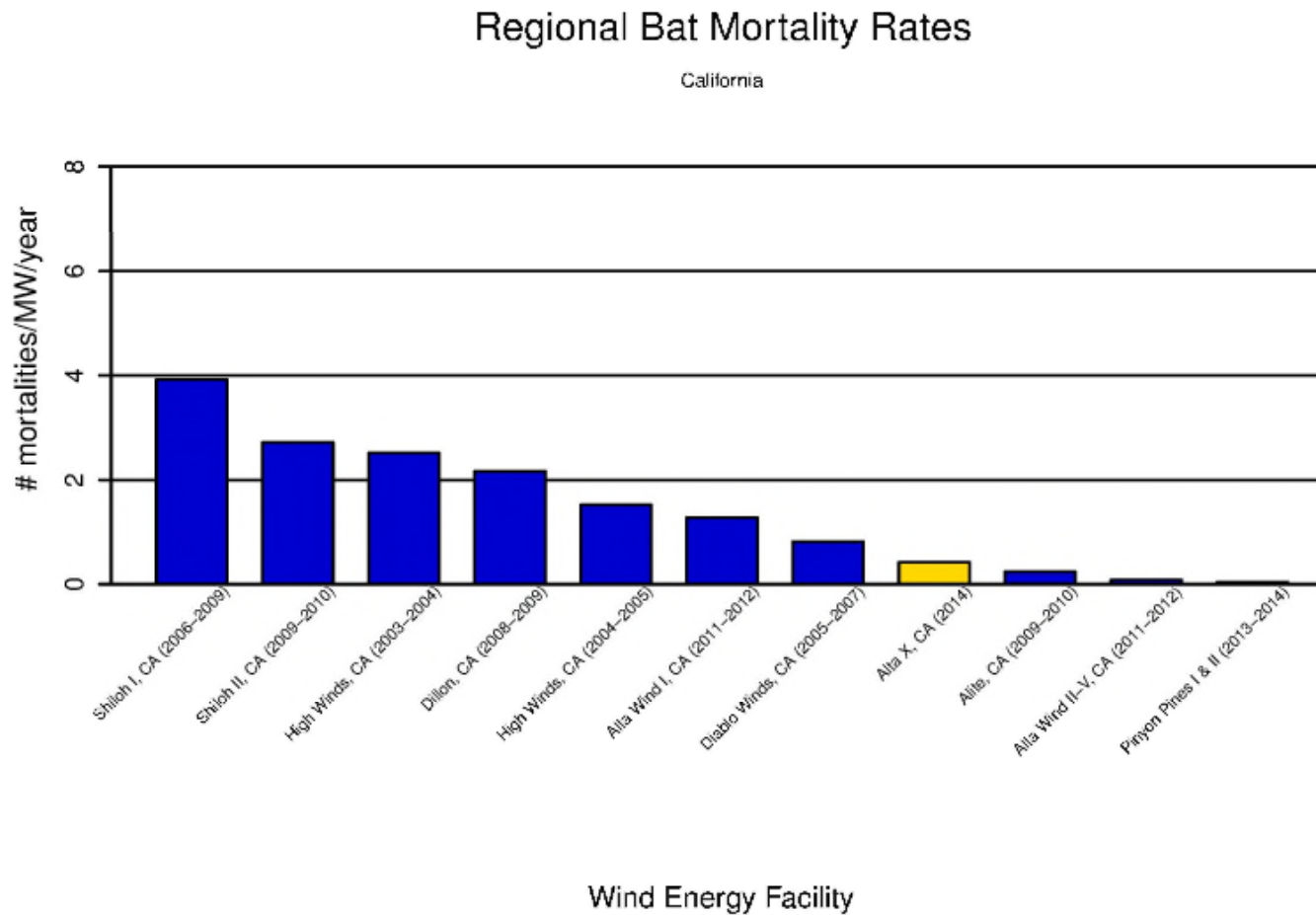
Figure 10. Mortality rates for bats (number of bats per MW per year) at the Alta X Wind Energy Project compared with studies at publicly-available wind energy facilities in California.
