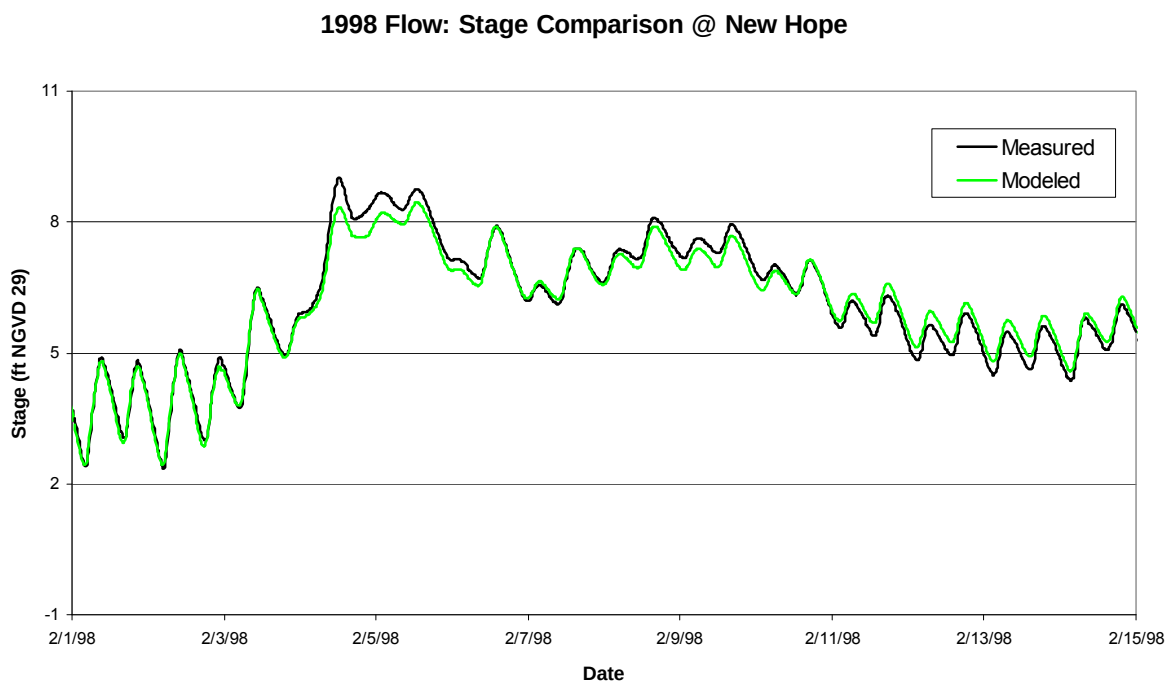
Figure E-8. Model Results Compared to Measured Data at Benson's Ferry (top panel) and New Hope (bottom panel) for the Year 1998 Flow
