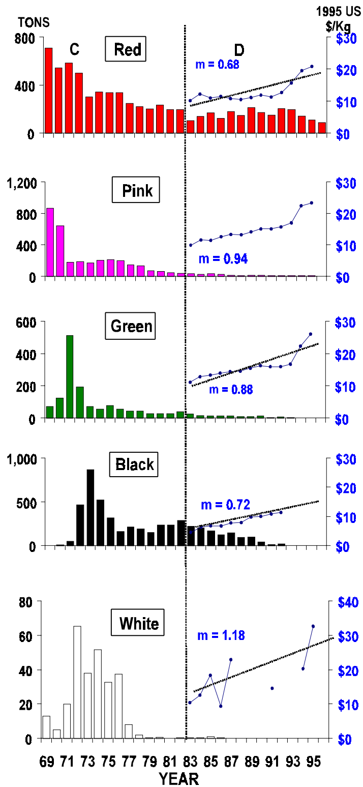
Figure 3-2. Landings for red, pink, green, black, and white abalones (bars): the ex-vessel average value (solid line), with fitted regression lines (dotted line) ( m = \text{slope} , t \times \text{year}^{-1} ).
