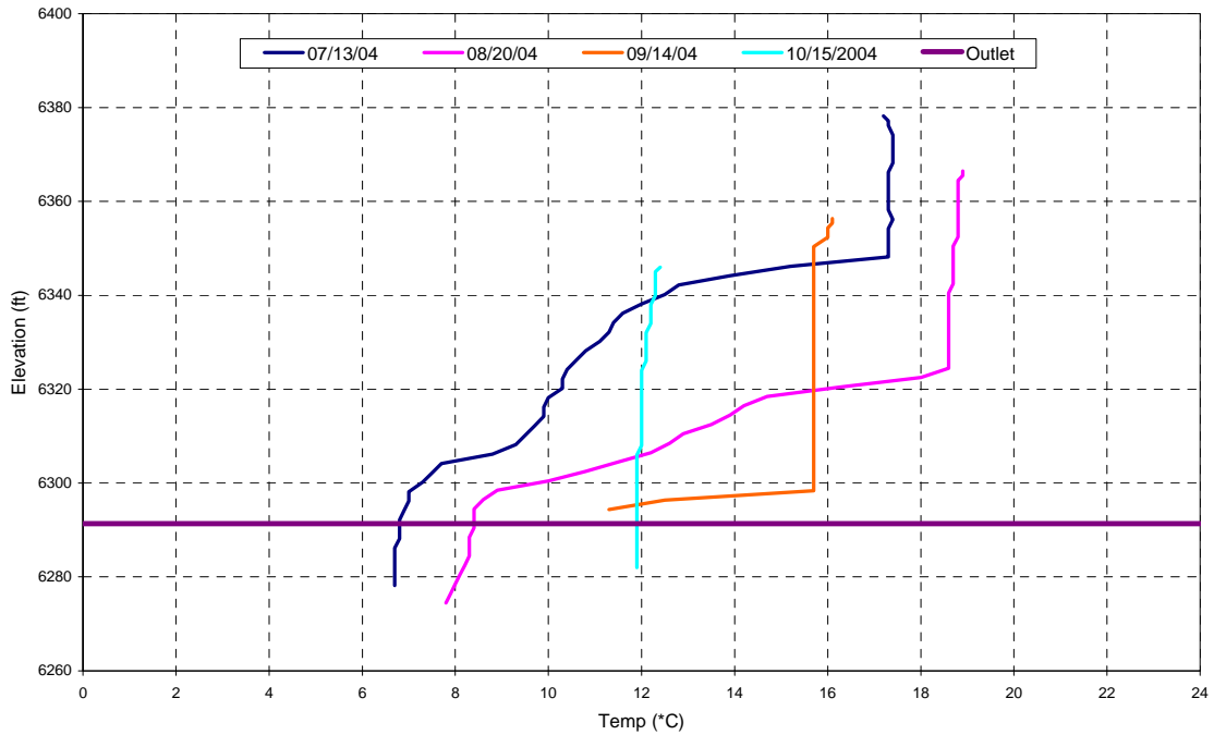
FIGURE 9 Water Temperature Profiles in Fordyce Lake During 2004
