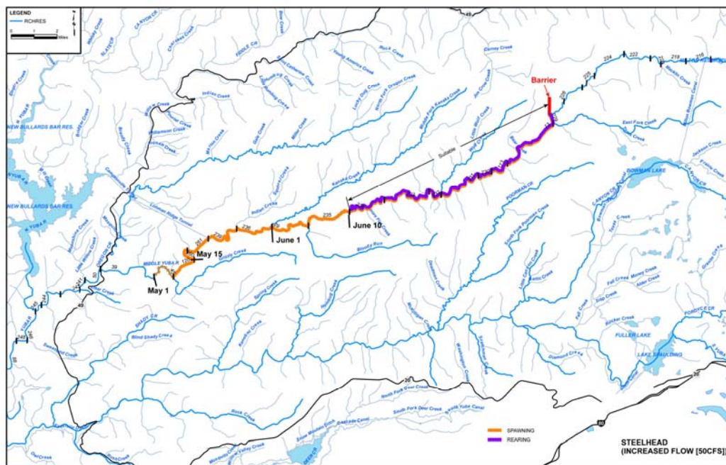
FIGURE 4-8 River Reaches With Suitable Water Temperatures for Steelhead in the Middle Yuba River Predicted with Increased Flows (50 cfs)
