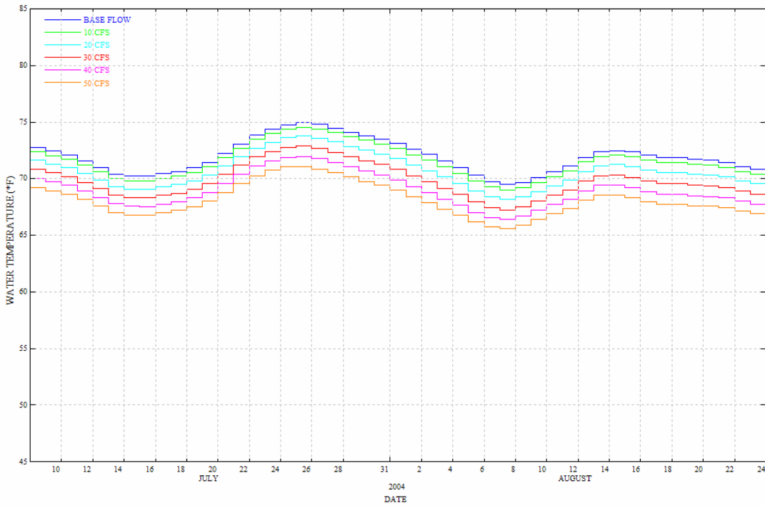
FIGURE 17 Comparison of 7-day Average Simulated Temperatures below Kanaka Creek for Base (4 cfs), 10, 20, 30, 40, and 50 cfs Flow Levels
