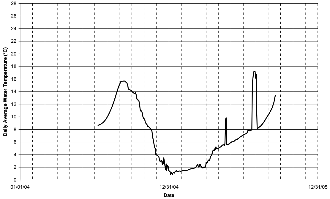
FIGURE 11 Daily Average Water Temperatures in the Bowman-Spaulding Canal Below Bowman Lake Short-duration temperature spikes likely due to operational changes (dewatering)
