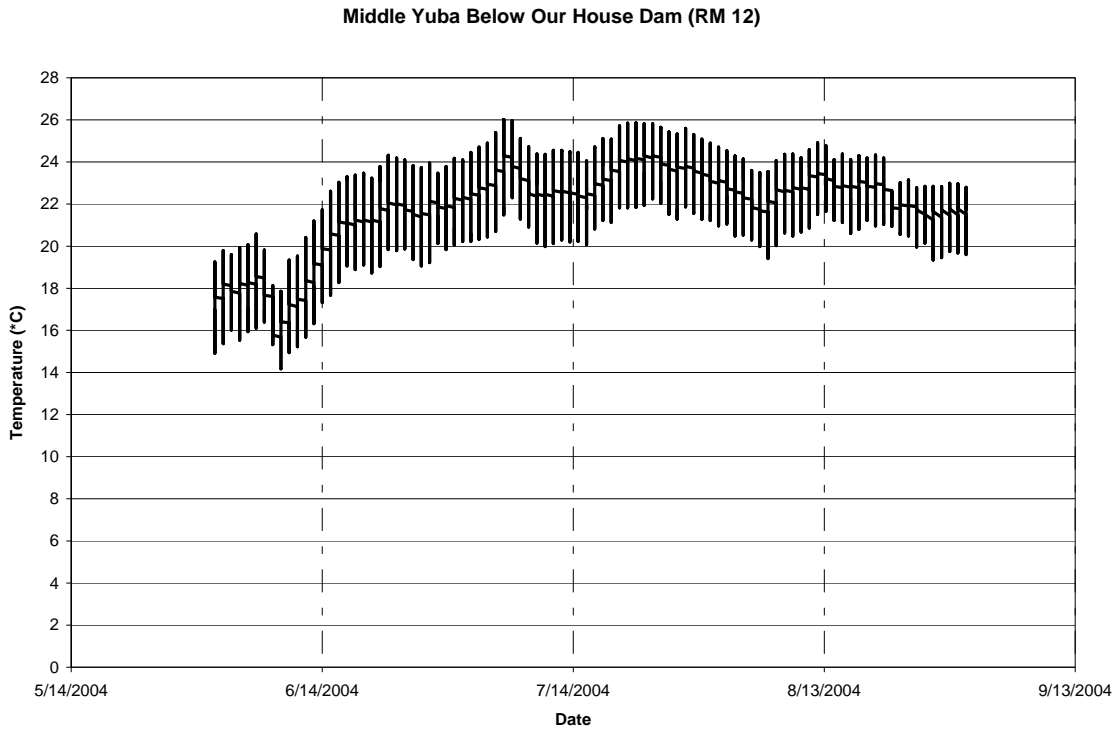
FIGURE 2B Summer Water Temperatures in the Middle Yuba River below Our House Dam (15-minute interval)
