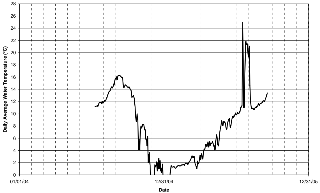
FIGURE 13 Daily Average Water Temperatures in the Bowman-Spaulling Canal Below Fuller Lake Short-duration temperature spikes likely due to operational changes (dewatering)
