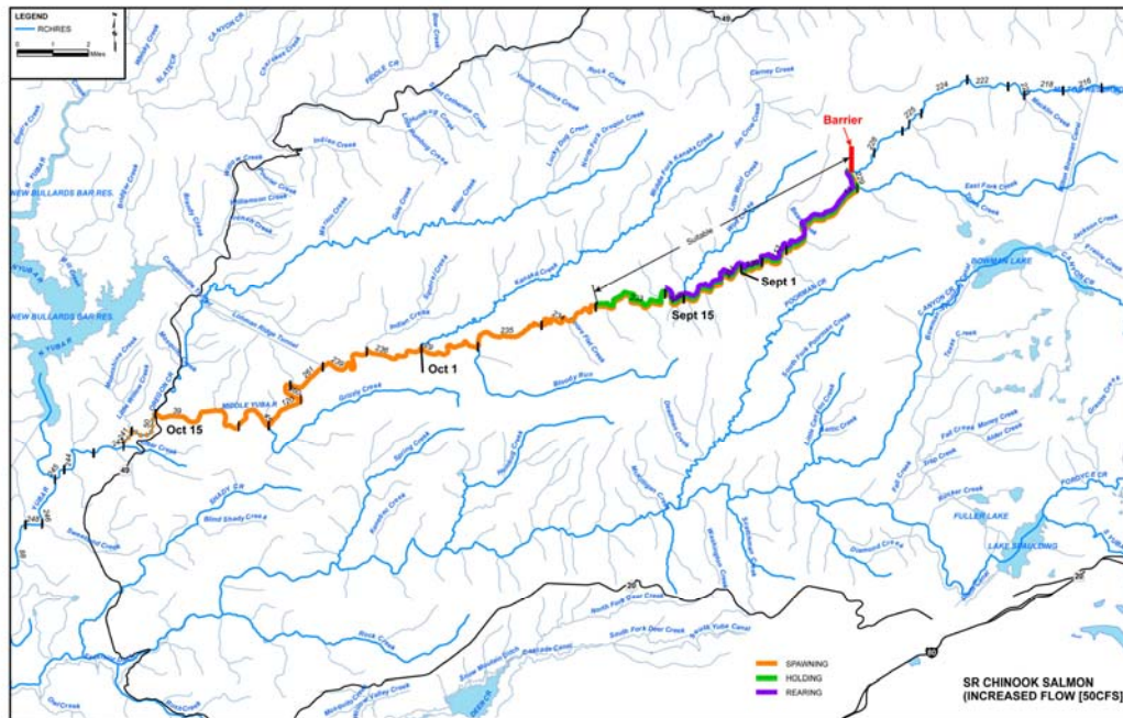
FIGURE 4-6 River Reaches with Suitable Water Temperatures for Spring-run Chinook Salmon in the Middle Yuba River Predicted with Increased Flows (50 cfs)
