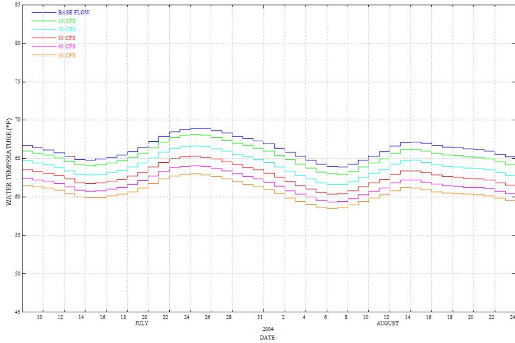
FIGURE 16 Comparison of 7-day Average Simulated Temperatures above Wolf Creek for Base (4 cfs), 10, 20, 30, 40, and 50 cfs Flow Levels
