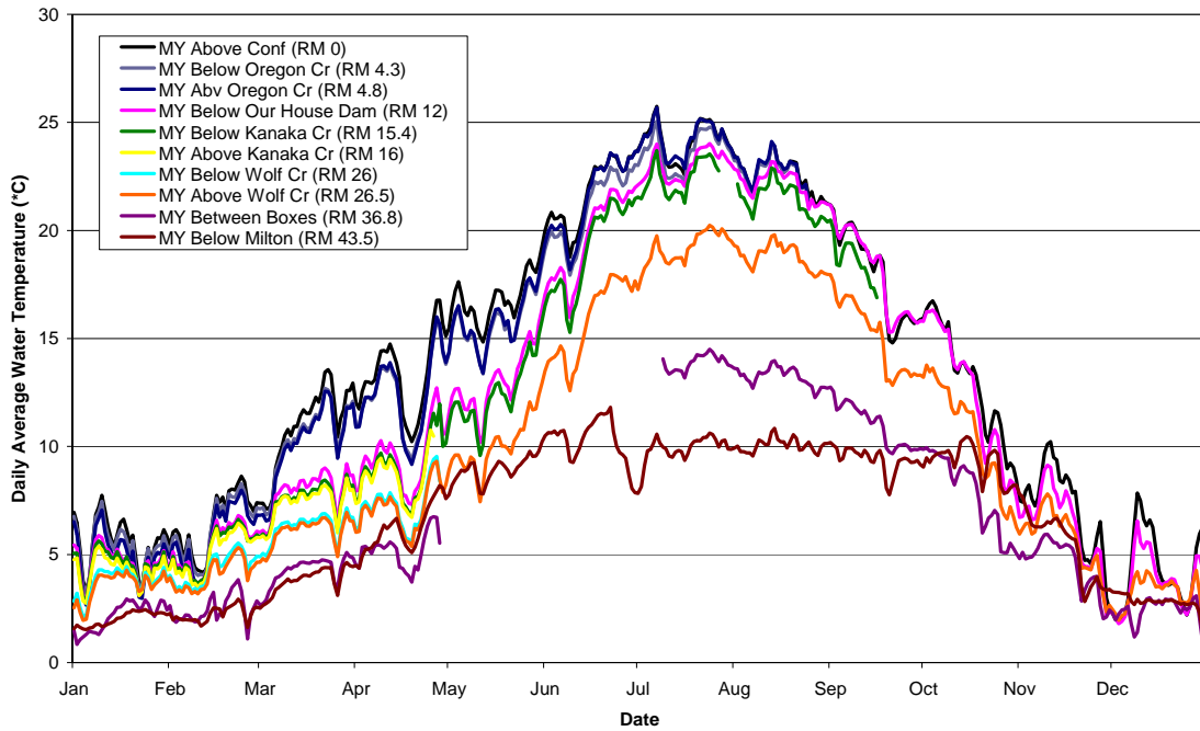
FIGURE 4B Water Temperatures in the Middle Yuba River (daily average) During 2004
