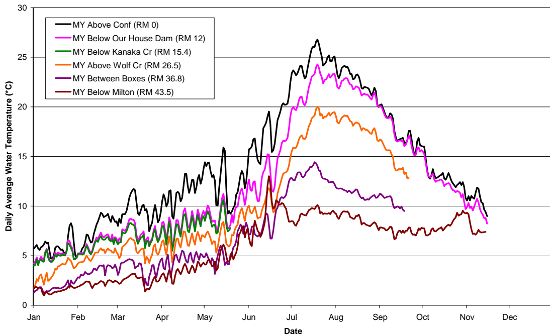
FIGURE 4C Water Temperatures in the Middle Yuba River (daily average) During 2005
