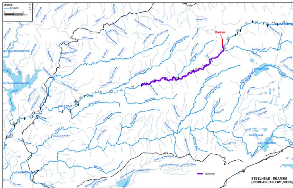
FIGURE 4-5 River Reaches with Suitable Water Temperatures for Steelhead Summer Rearing (in purple) in the Middle Yuba River Predicted With Increased Flows (50 cfs)
