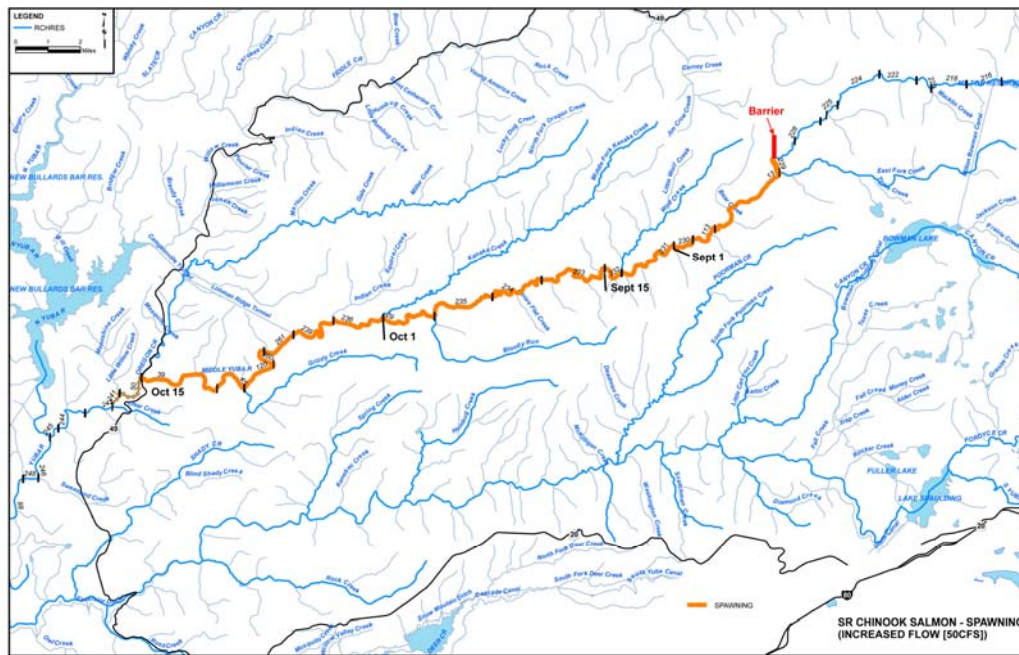
FIGURE 4-2 River Reaches With Suitable Water Temperatures for Spring-run Chinook Salmon Spawning and Incubation (in orange) in the Middle Yuba River Predicted With Increased Flows (50 cfs)
