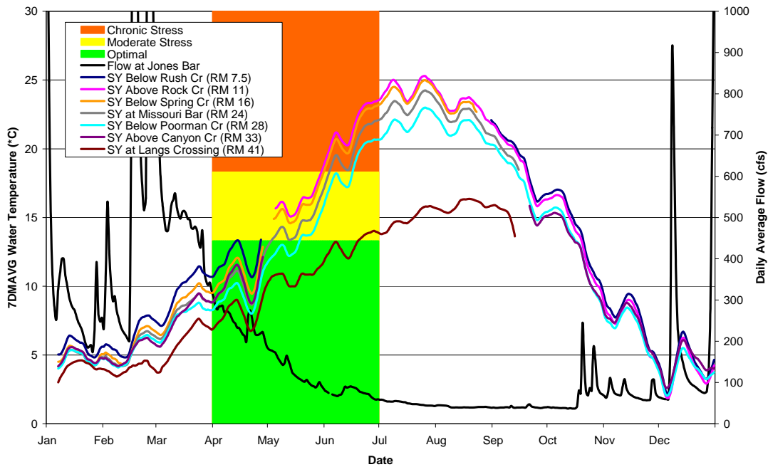
FIGURE 3-2 Average Water Temperatures and Flow During the Adult Spring-run Chinook Salmon Migration Period in the South Yuba River Under Current Operations (2004)
