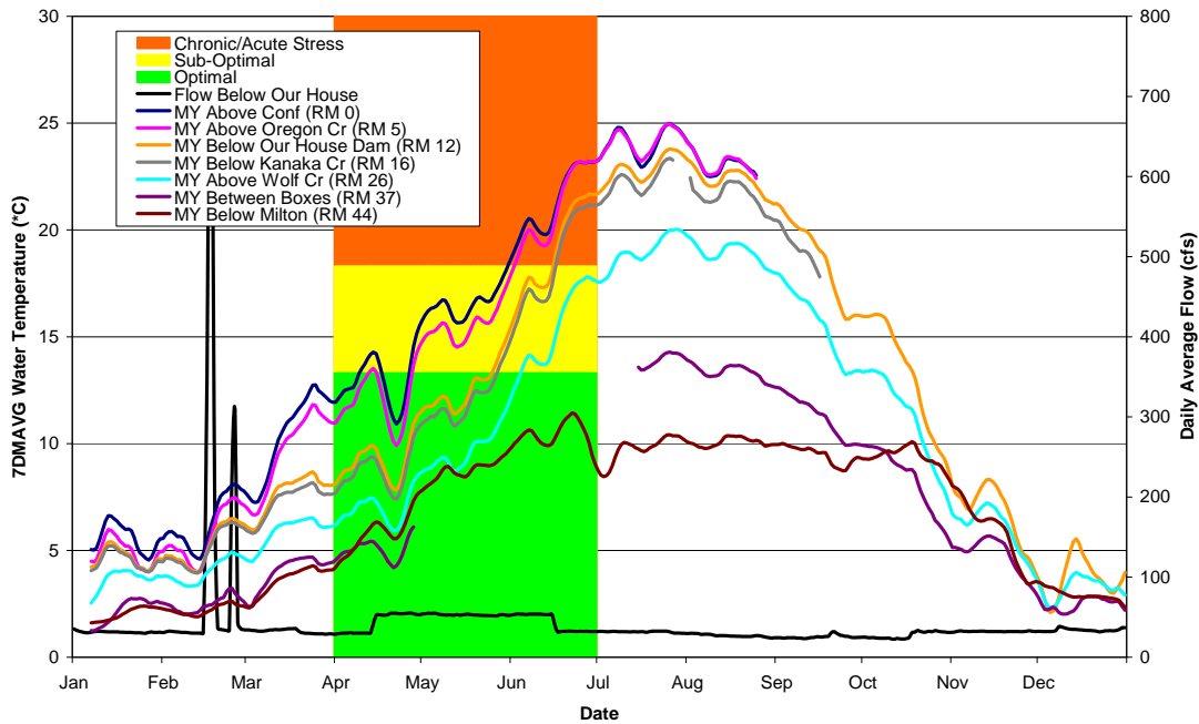
FIGURE 3-1 Average Water Temperatures and Flow During the Adult Spring-run Chinook Salmon Migration Period in the Middle Yuba River Under Current Operations (2004)
