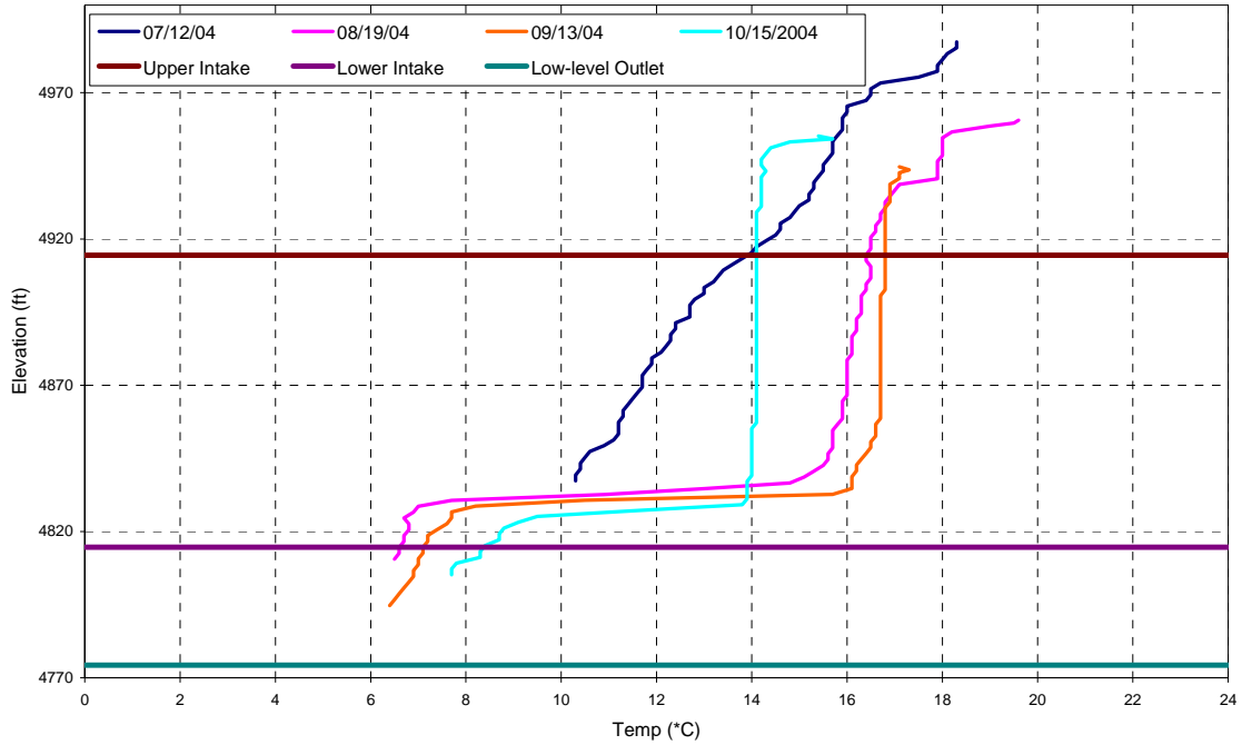
FIGURE 8 Water Temperature Profiles in Lake Spaulding During 2004
