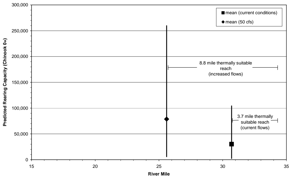
FIGURE 3-17 Predicted Summer Rearing Capacity of Spring-run Chinook Salmon Fry (age 0+) in Thermally Suitable Reaches of the Middle Yuba River Under Current (2004) and Increased Flows Vertical lines indicate predicted minimum and maximum.
