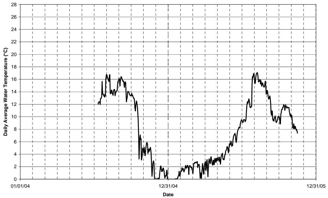
FIGURE 14 Daily Average Water Temperatures in Fordyce Creek Above Lake Spaulding
