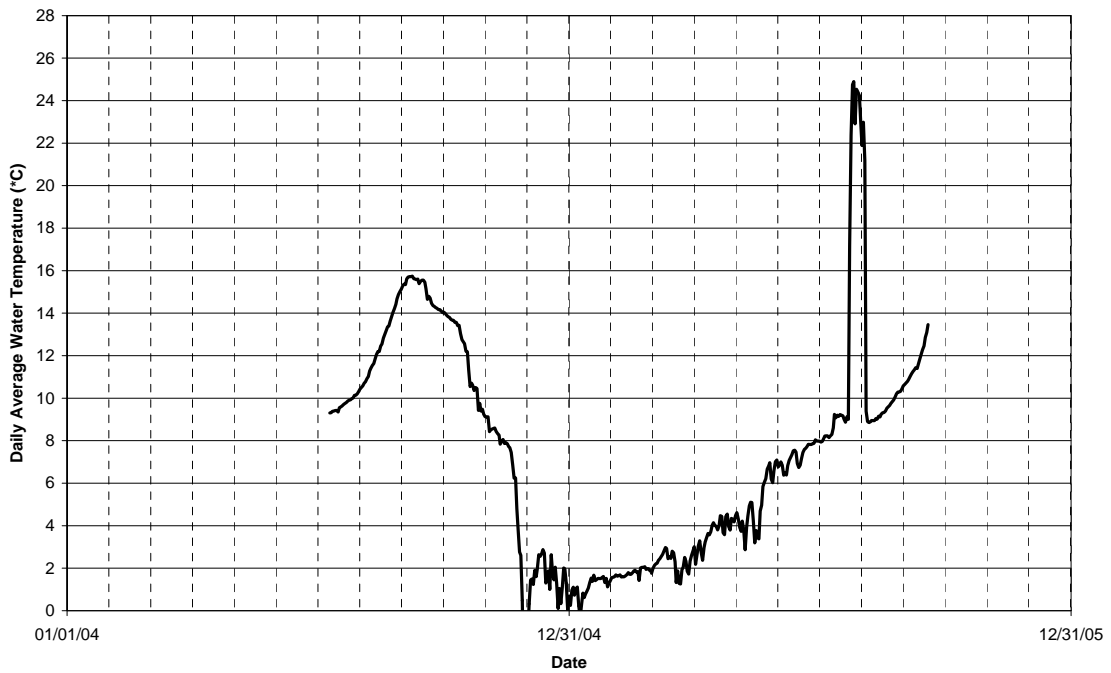
FIGURE 12 Daily Average Water Temperatures in the Bowman-Spaulding Canal Below Rucker Lake Short-duration temperature spikes likely due to operational changes (dewatering)
