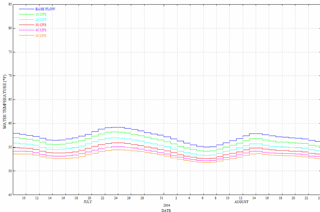
FIGURE 15 Comparison of 7-day Average Simulated Temperatures between Box Canyons 1 and 2 for Base (4 cfs), 10, 20, 30, 40, and 50 cfs Flow Levels
