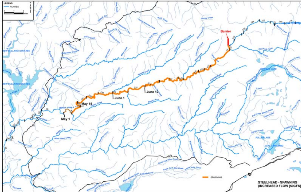
FIGURE 4-4 River Reaches with Suitable Water Temperatures for Steelhead Spawning and Incubation in the Middle Yuba River Predicted With Increased Flows (50 cfs).
