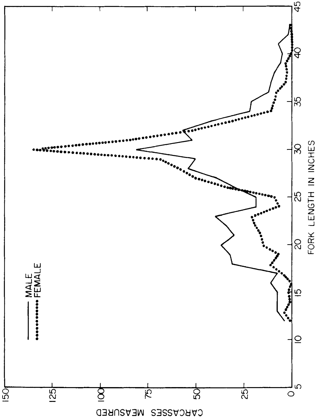
Figure 2. Length frequencies of king salmon measured during the 1970 spawning season in the Trinity River.
