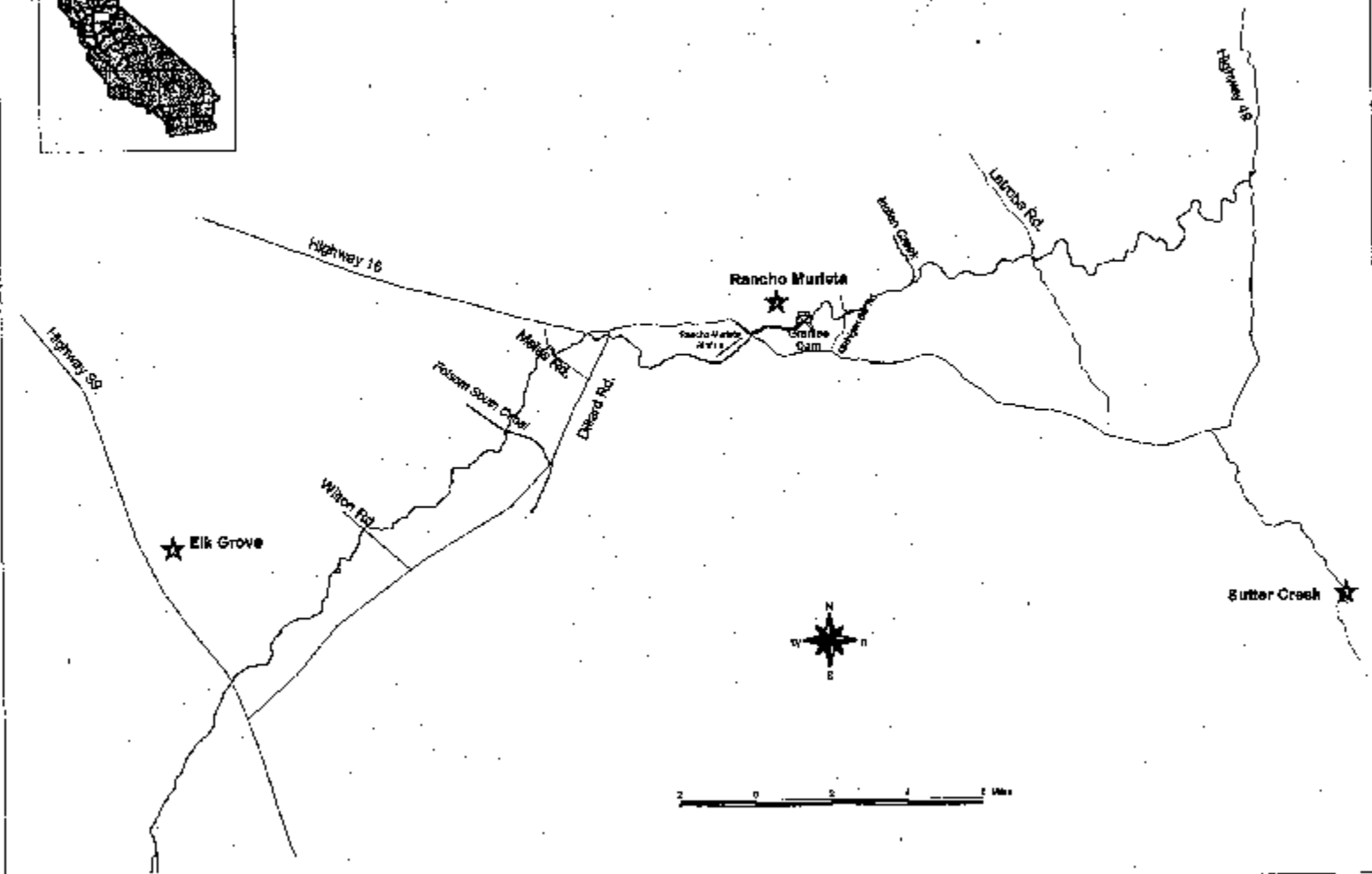
Figure 1. Location of Cosumnes River study landmarks.
