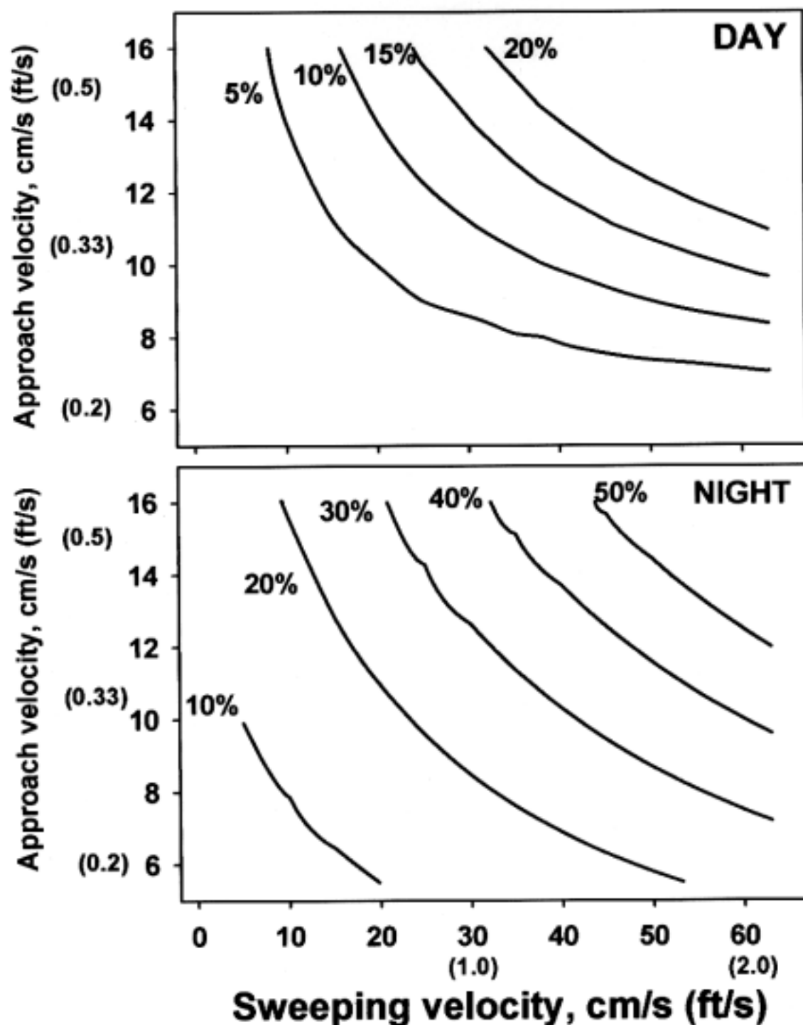
Figure 2. Effects of approach and sweeping velocity on 48-h post-experiment mortality of delta smelt (12°C, 4-6 cm SL). Each isopleth depicts selected levels of mortality, expressed as % of exposed fish, at the various combinations of approach and sweeping velocity. Plots were derived from general linear statistical models describing the effects of approach and sweeping velocities on 48-h mortality (see text). Slight irregularities in the lines do not represent real differences from the "smooth" relationships shown.
