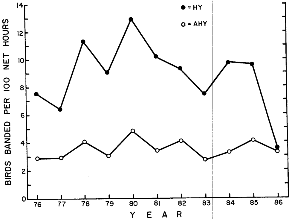
FIGURE 1. Number of birds of all species combined banded per 100 net hr during the period 10 May to 17 August for each of 11 years.
