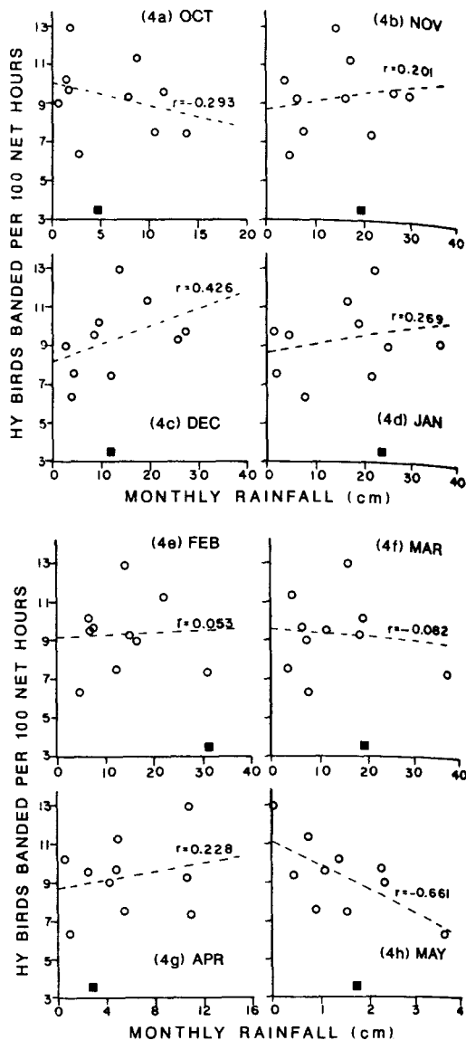
FIGURE 4. Number of HY birds banded per 100 net hr (during the period 10 May to 17 August) as a function of monthly rainfall totals for the 10 years 1976 to 1985 (○) and for 1986 (■). Also shown are the linear regression lines and correlation coefficients for the 10 years 1976 to 1985. (4a) October. (4b) November. (4c) December. (4d) January. (4e) February. (4f) March. (4g) April. (4h) May.
