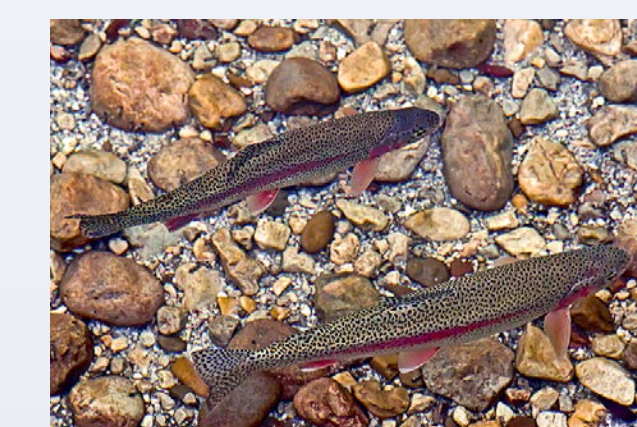
Rainbow trout, introduced genetic material
