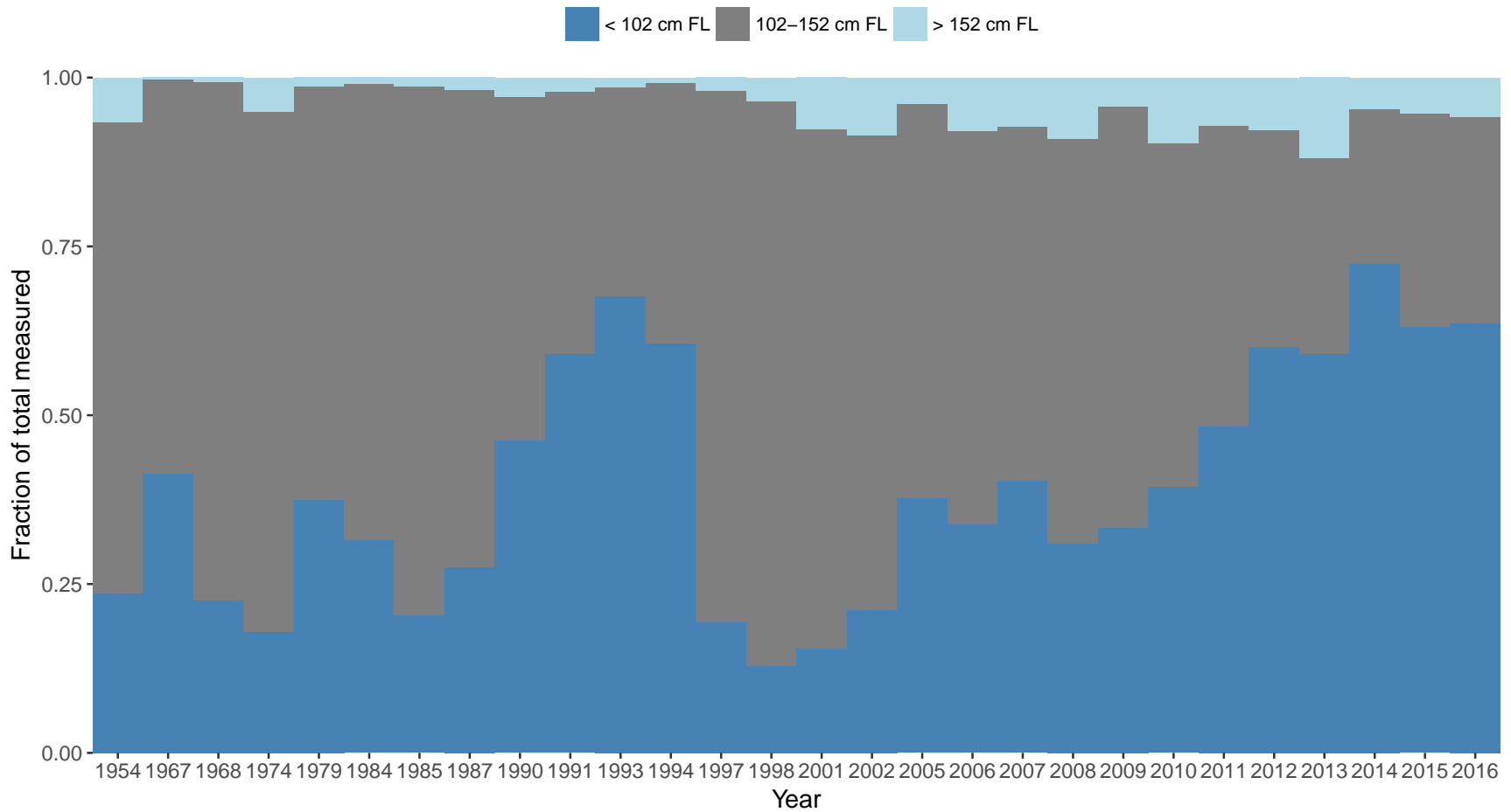
Fraction by Length Category of White Sturgeon Catch from CDFW Sturgeon Population Study Trammel Nets in Suisun Bay and San Pablo Bay (Aug–Oct), 1954–2016; current slot 102–152 cm FL
