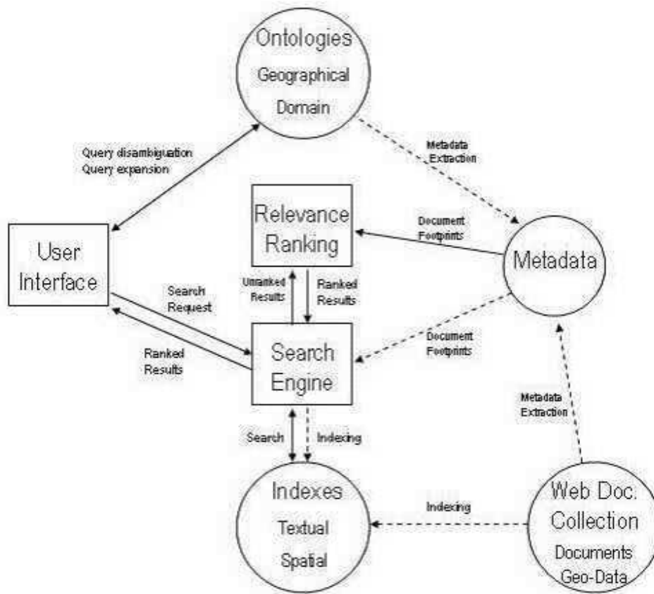
Fig. 1. SPIRIT search engine architecture.
