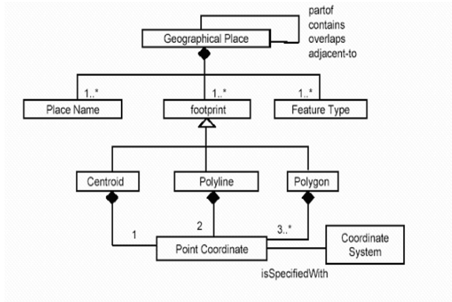
Fig. 2. Conceptual design of the geo-ontology.
