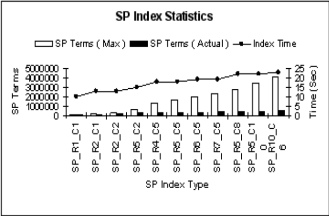
Fig. 4. SP index statistics.
