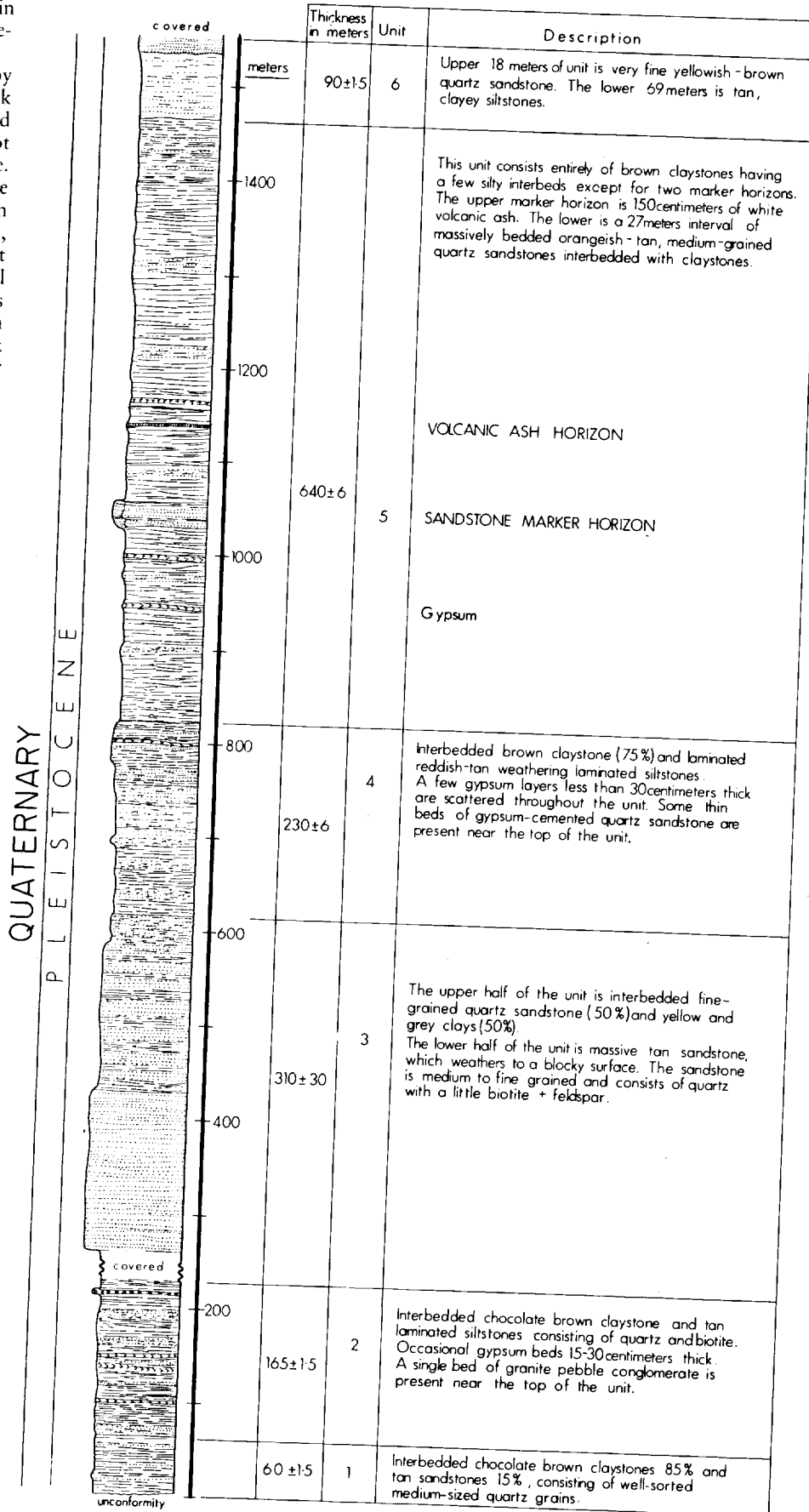
Figure 4. Columnar section of Borrego Formation east of Salton Sea, California.
