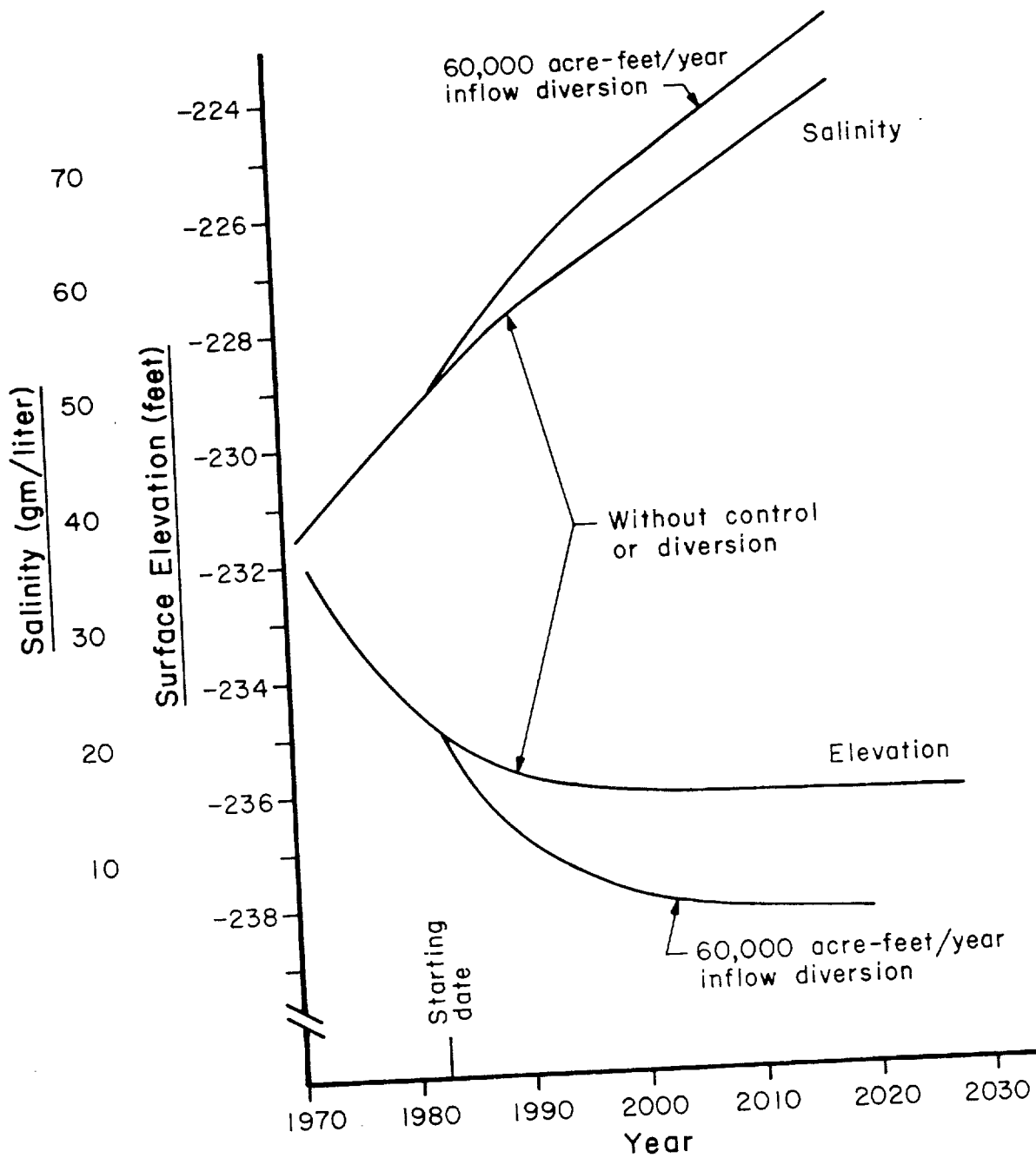
Figure 1 Behavior of Salton Sea With and Without Diversion of Inflow (60,000 acre-ft/yr for cooling 1000mw geothermal power plants—no return of blow-down to sea)
