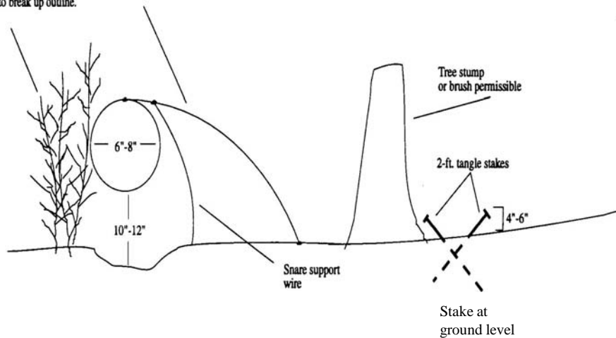
Fig. 8. Kill snare with washer lock.
