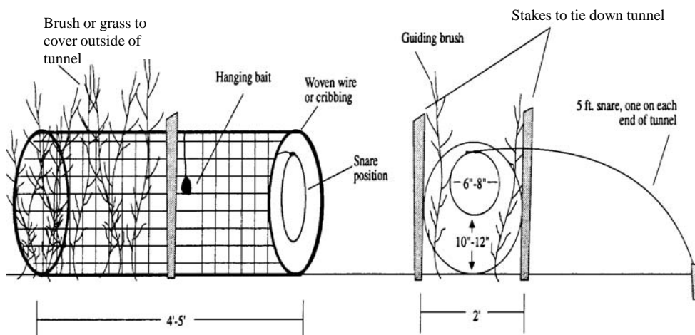
Fig. 6. Cubby set with snare.
