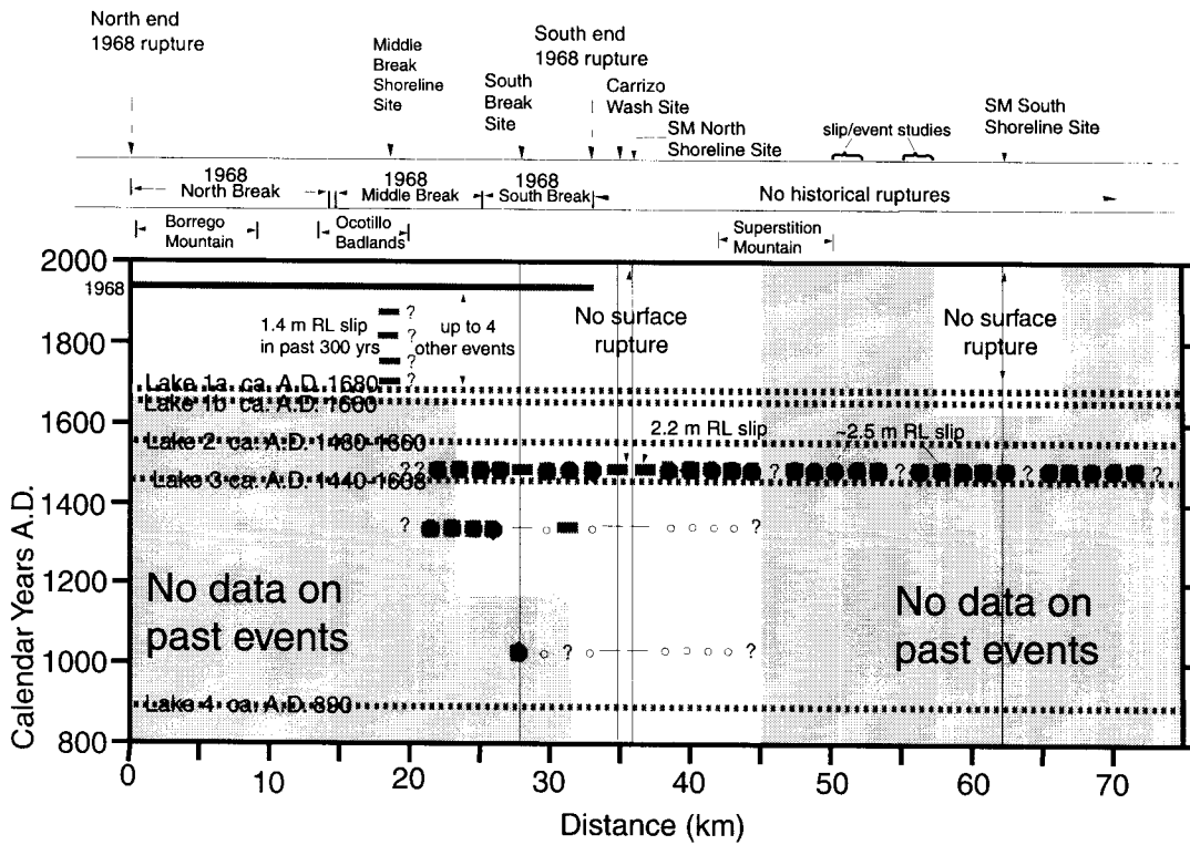
Figure 1. Correlation diagram of ongoing paleoseismic sites along the southern San Jacinto project. The record of earthquakes at each site are being extended as new dates come in, and new trenches are excavated.
