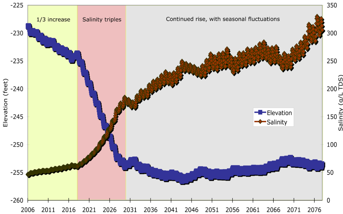
Figure 8. Future salinity trends at the Salton Sea.
