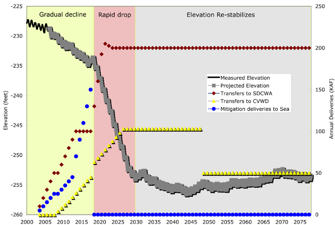
Figure 4. Surface elevation, Jan. 2000 - Dec. 2077. 19
