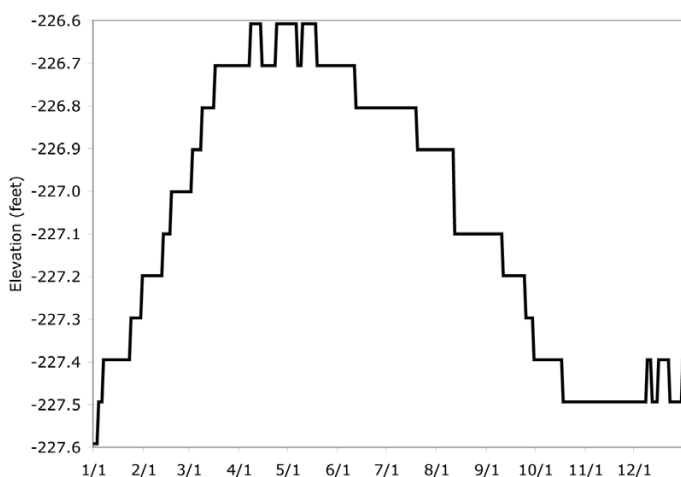
Figure 3. Daily Salton Sea elevation, 1995. Source: USGS
