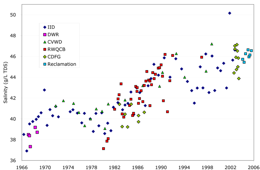
Figure 7. Reported Salton Sea salinities 1966-2006, by agency. 24
