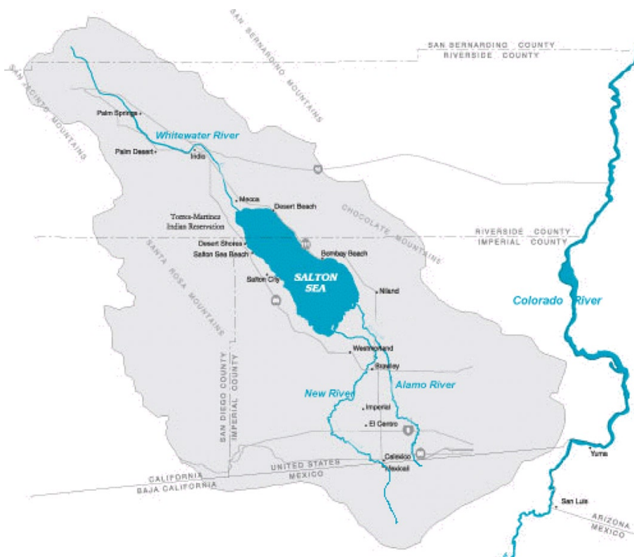
Figure 1. The Salton Sea watershed. 8
