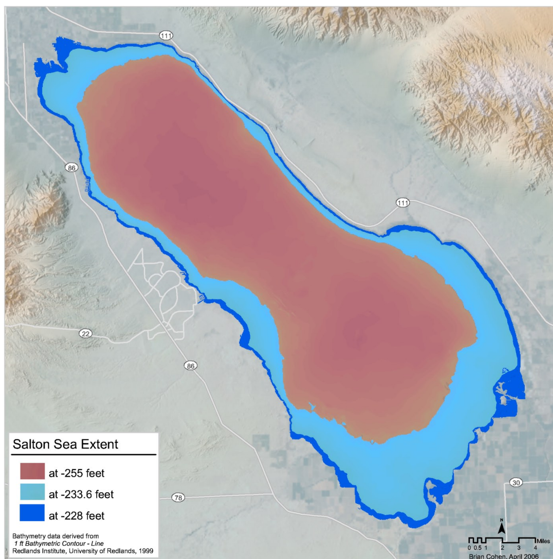
Figure 5. Exposed lakebed at -233.6' and at -255'.
