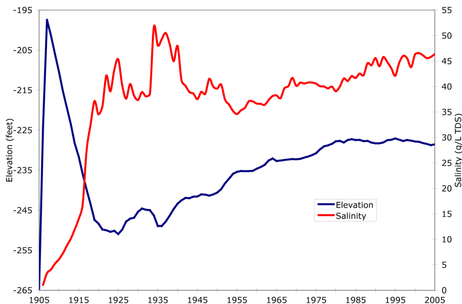
Figure 2. Historic elevation and salinity of the Salton Sea. 9
