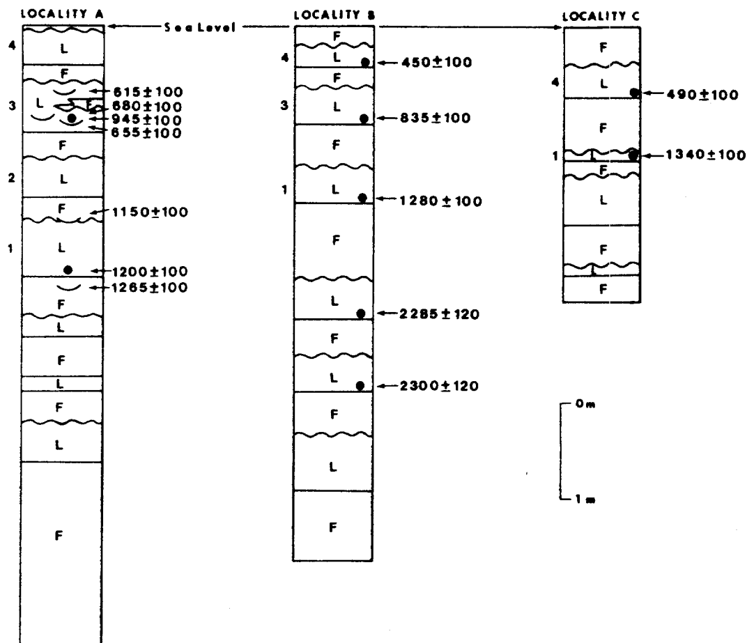
FIG. 4. Stratigraphic sections at radiocarbon localities A, B, and C. Dates give in \delta^{13}\text{C} -corrected radiocarbon yr B.P. (Table 1). Explanation: (F) fluvial deposits; (L) lacustrine deposits; (1) deposits of lacustral interval 1; (2) deposits of lacustral interval 2; (3) deposits of lacustral interval 3; (4) deposits of lacustral interval 4; solid dots represent position of shell dates; dish-shapes represent position of hearth-charcoal dates; straight-line contacts are conformable; wavy-line contacts are unconformable.
