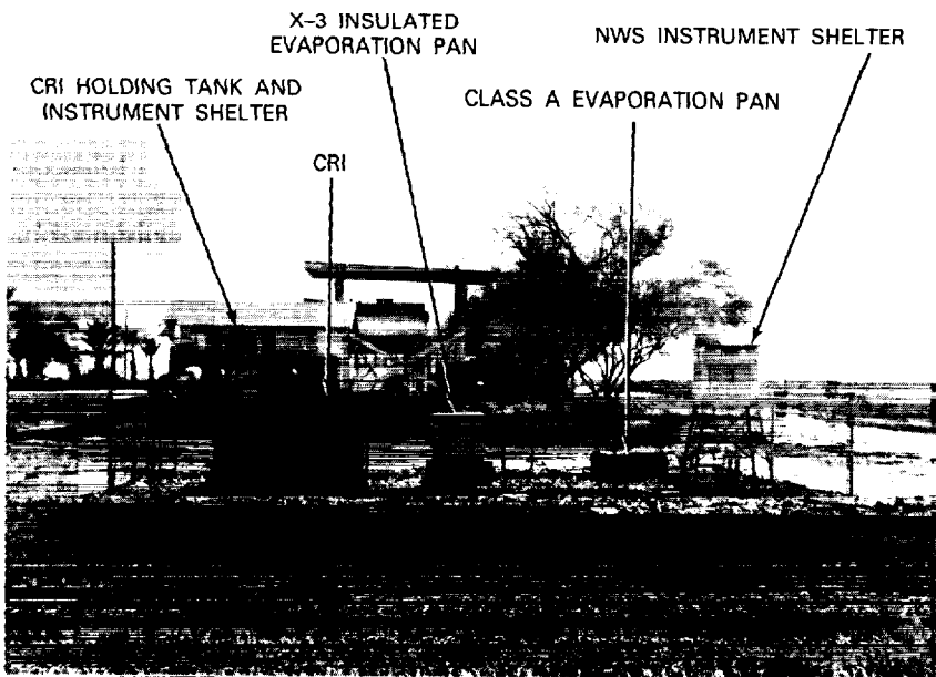
FIGURE 2.—South Station enclosure with Cummings Radiation Integrator and National Weather Service instruments.
