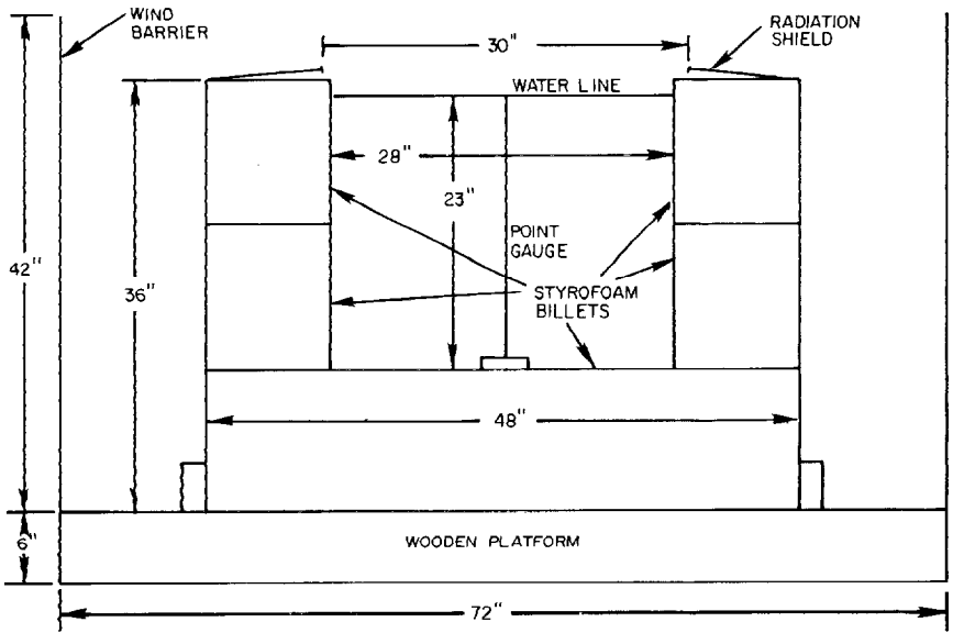
FIGURE 3.—Cross section of Cummings Radiation Integrator.
