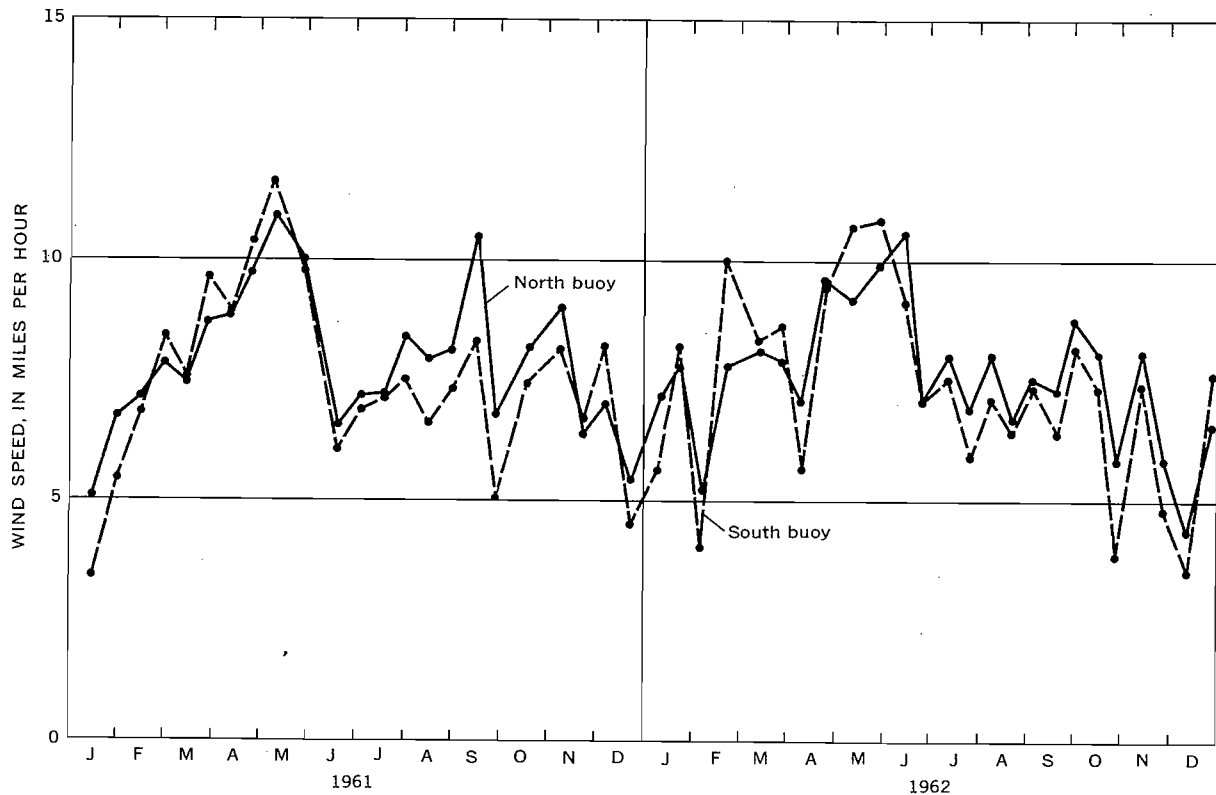
FIGURE 56.—Average wind speeds for energy-budget periods as measured at two buoys in Salton Sea, 1961-62.
