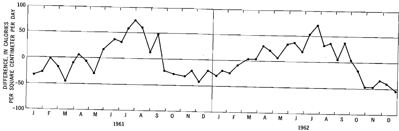
FIGURE 66.—Seasonal differences between measured and computed long-wave atmospheric radiation.
