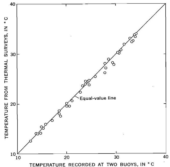
FIGURE 51.—Relation between water-surface temperatures of Salton Sea as recorded at two buoys and as measured during thermal surveys.
