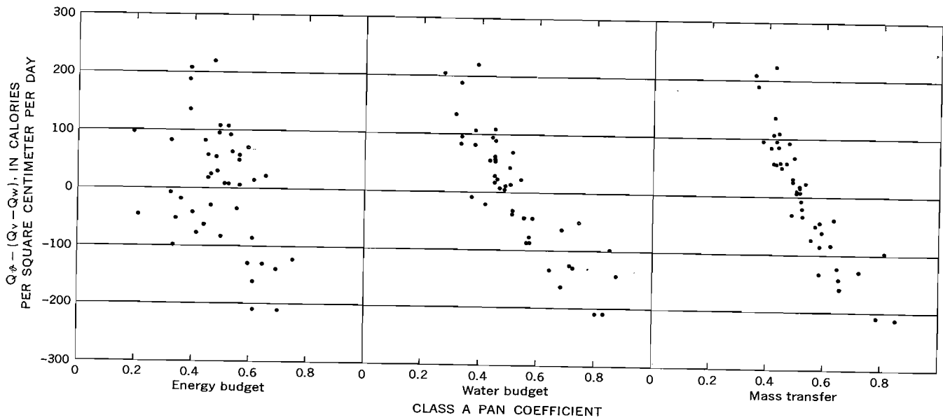
FIGURE 68.—Correlation between changes in energy storage in Salton Sea and coefficients for a class A pan at Sandy Beach.
