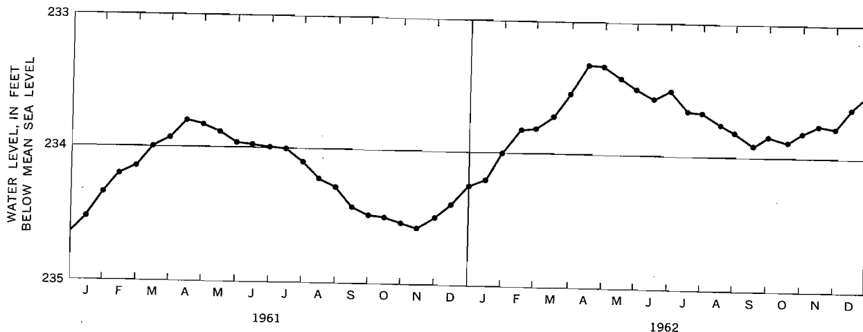
FIGURE 58.—Water level of Salton Sea at midmonth and at end of month, 1961-62.
