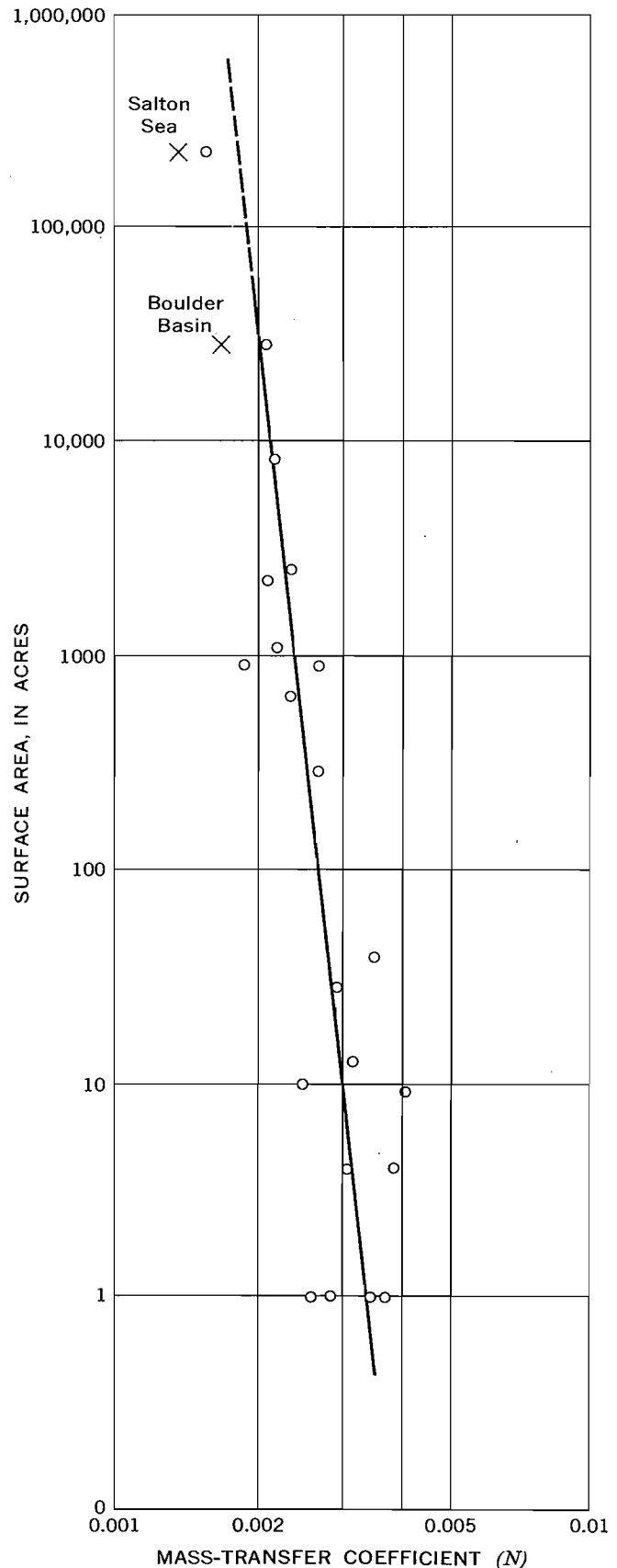
FIGURE 69.—Relation between mass-transfer coefficient, N , and surface area of water body. Values indicated for Boulder Basin and Salton Sea by circles are based on vapor pressures of air measured locally at the respective water bodies; values indicated by crosses for the same water bodies are based on vapor pressures of air at Las Vegas, Nev., and Yuma, Ariz., respectively. (Adapted from Harbeck, 1962 fig. 31.)
