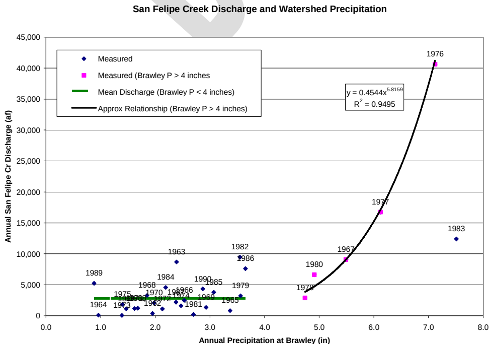
Figure 4 Relationship Between San Felipe Creek Discharge and Precipitation at Brawley
