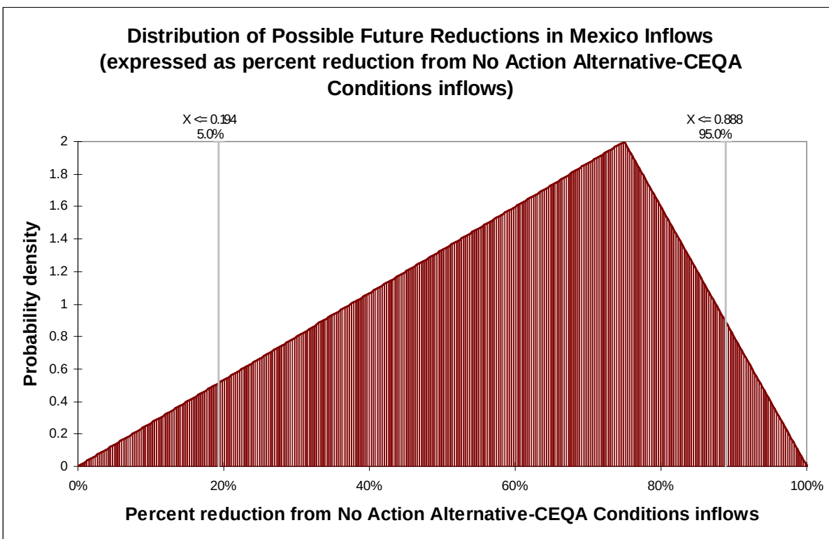
Figure 15 Probability Distribution to Describe Range of Uncertainty in Future Mexico Flows
