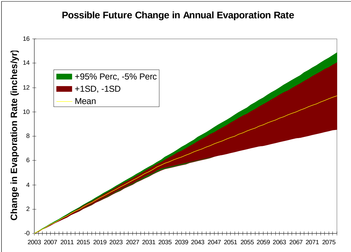
Figure 25 Possible Future Change in Annual Evaporation Rate
