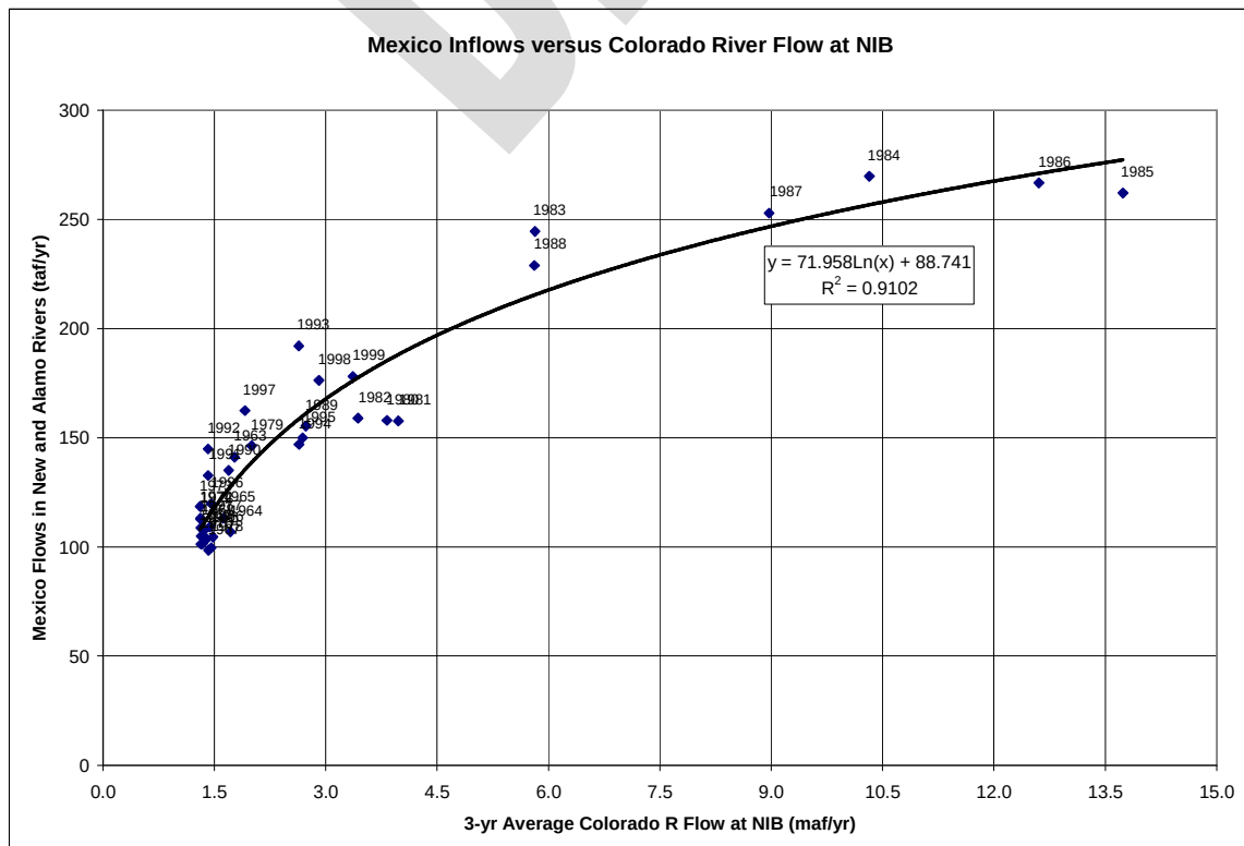
Draft Figure 10 Relationship Between Colorado River Flow at the Northerly International Boundary and Flows into Imperial Valley from Mexico January 2006
