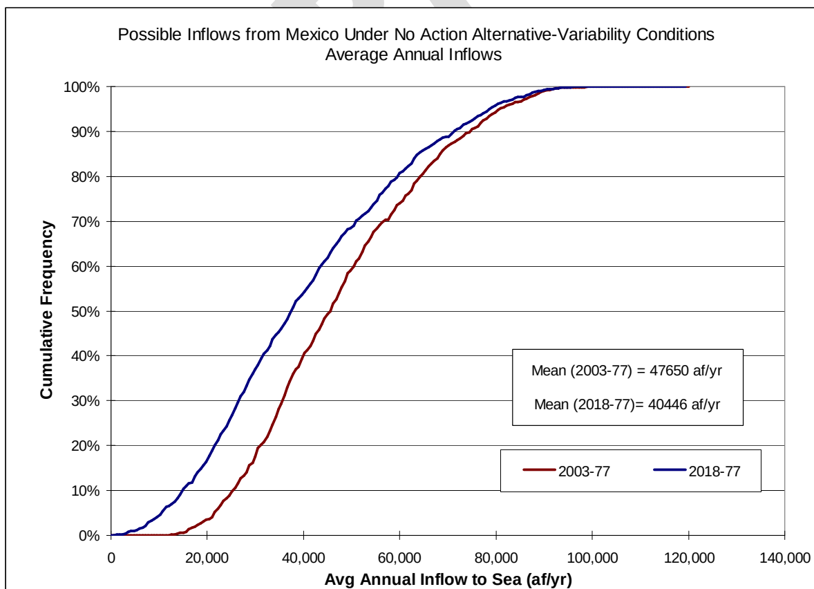
Figure 16 Possible Inflows from Mexico for No Action Alternative-Variability Conditions
