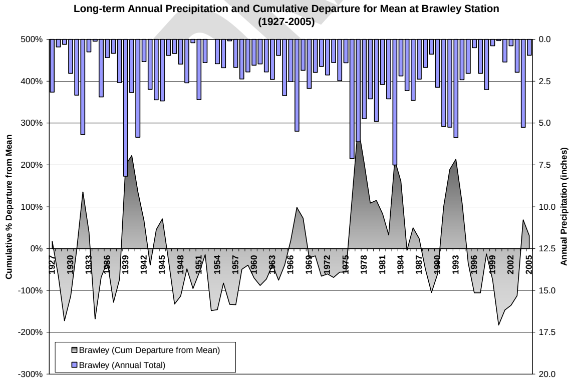
Figure 3 Annual Precipitation and Percent Cumulative Departure from the Mean at Brawley
