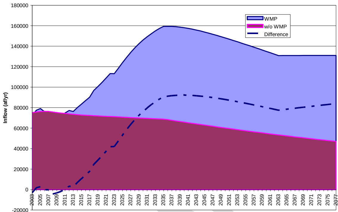
Figure 21 Estimated Future Salton Sea Inflows from the Coachella Valley with and without WMP
