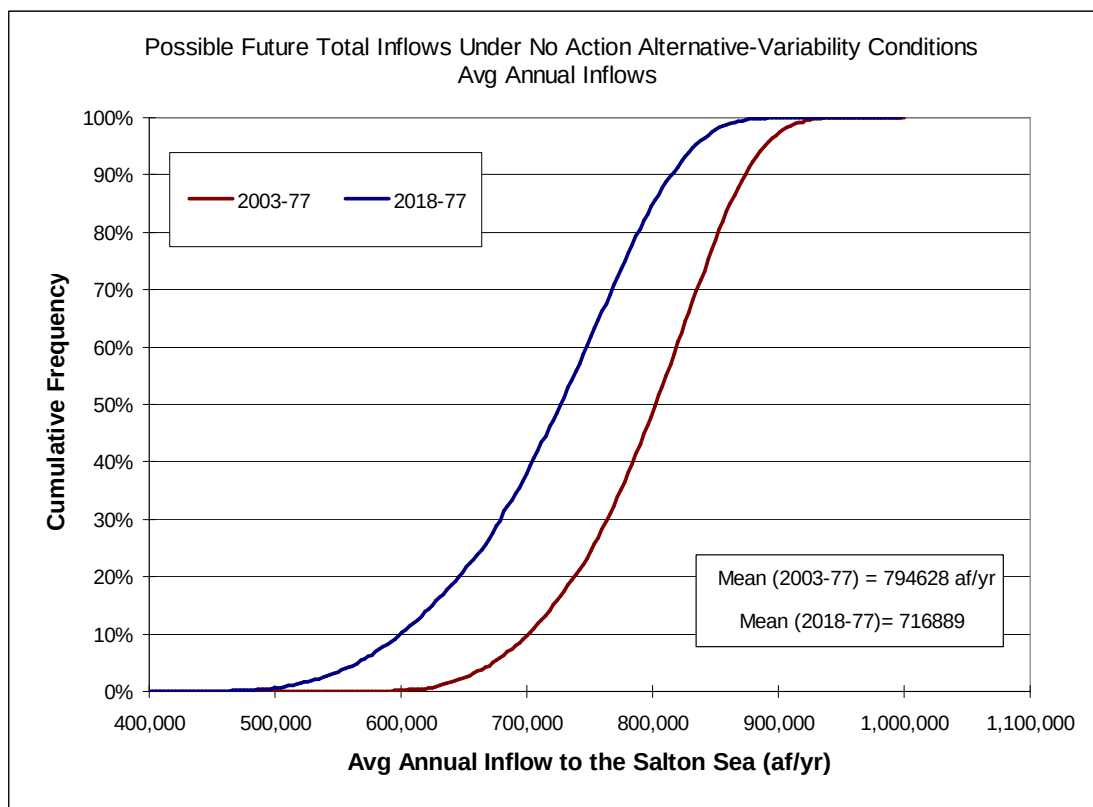
Figure 26 Possible Total Salton Sea Inflows for No Action Alternative-Variability Conditions
