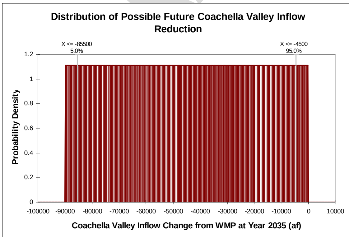
Figure 22 Probability Distribution to Describe Range of Uncertainty in Future Coachella Valley Flows
