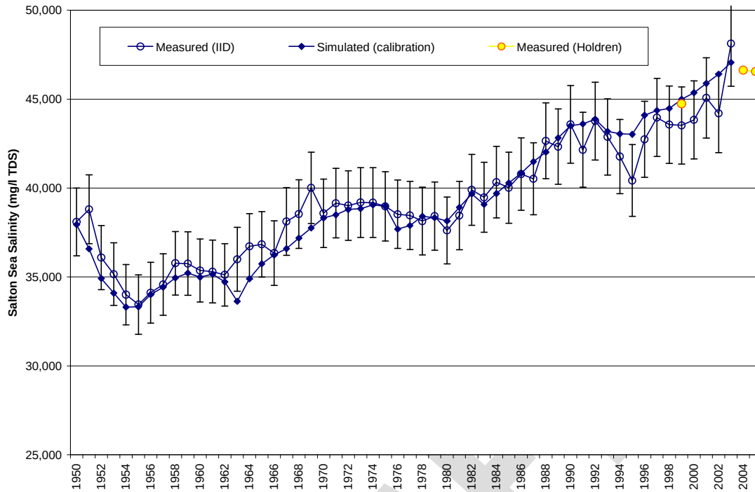
Figure 8 Measured and Simulated Salton Sea Salinity. Error Bars Represent +/- 2000 mg/L
