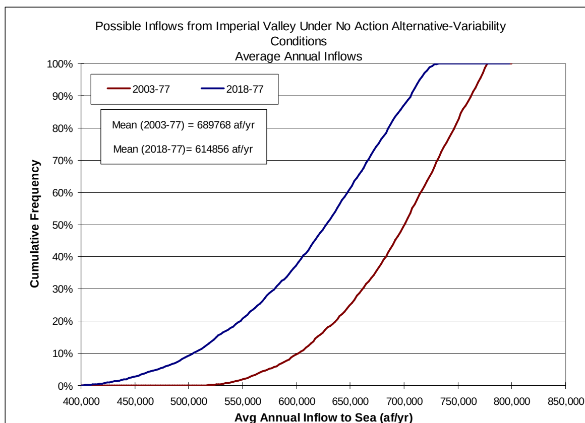
Figure 20 Possible Inflows from the Imperial Valley for No Action Alternative-Variability Conditions
