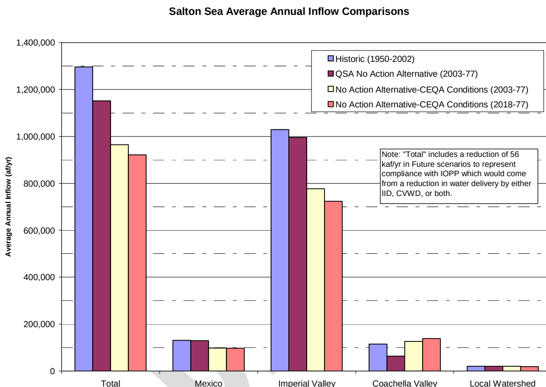
Figure 12 Comparison of Average Annual Inflows to the Salton Sea Under Historic, QSA No Action Alternative, and No Action Alternative-CEQA Conditions
