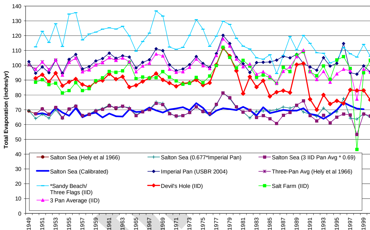
Figure 6 Estimated Annual Evaporation Rates Determined from Water Budget and Pan Evaporation Measurements
