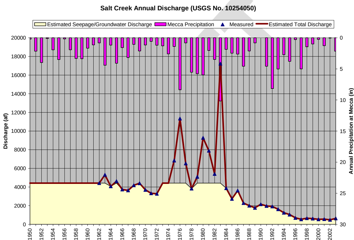
Figure 5 Historical Salt Creek Discharge and Estimated Baseflow from Seepage/Groundwater
