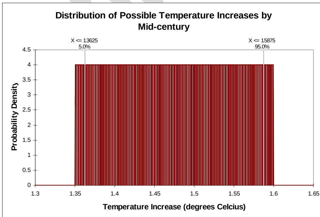
Figure 24 Probability Distribution to Describe Range of Uncertainty in Future Climate Change
