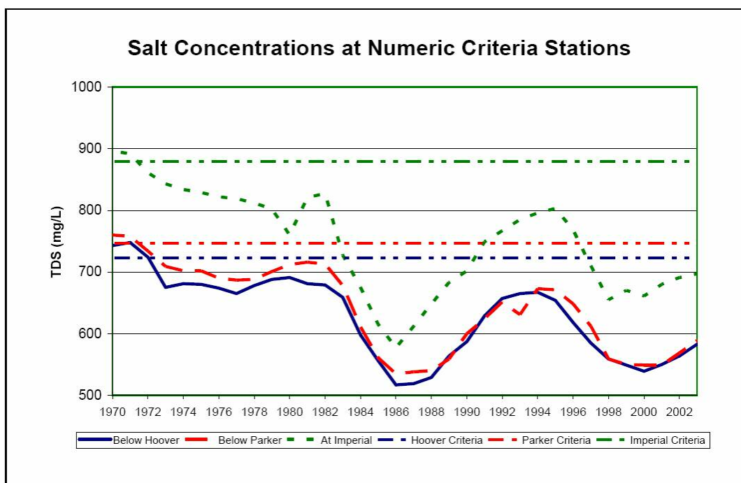
Figure 17 Salt Concentrations at Numeric Criteria Stations (Source: CRBSCF 2005)
