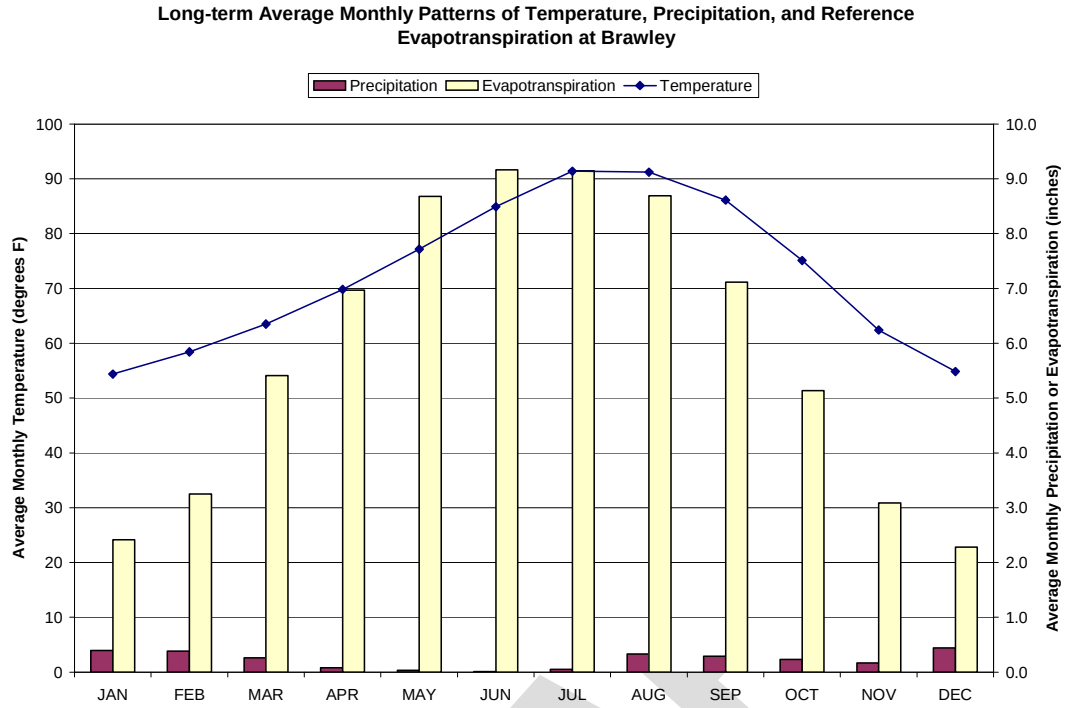
Figure 2 Long-term Average Monthly Temperature, Precipitation, and Reference Evapotranspiration at Brawley
