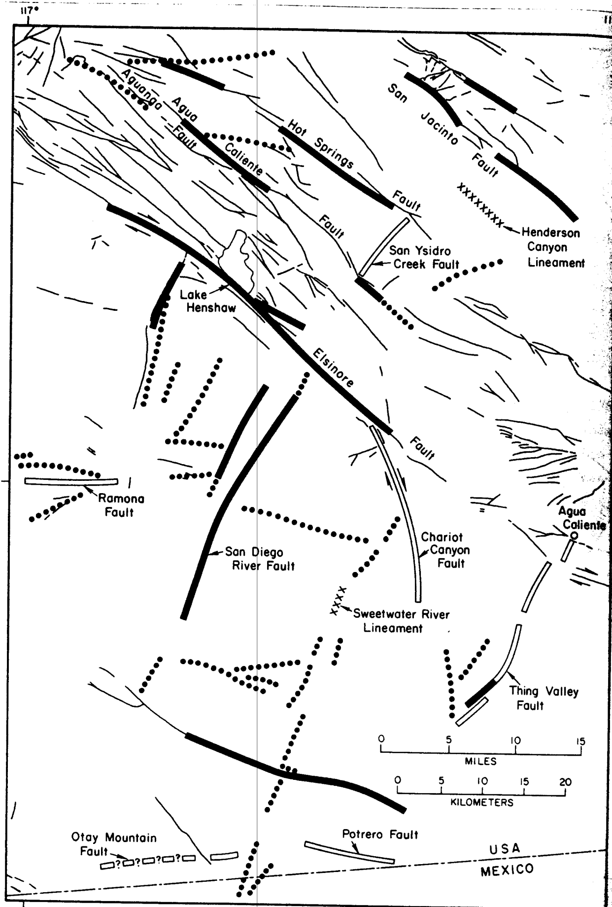
Fig. 2 - Faults and lineaments visible on Skylab and ERTS imagery of southwestern California. Solid lines: faults shown on Strand (1962), Rogers (1965), and Jennings (1973); Heavy lines: on satellite images; Light lines: faults do not appear. Open lines: previously unmapped faults. Dotted lines: Lineaments of unknown character. XXXX: Lineament not due to faulting.
