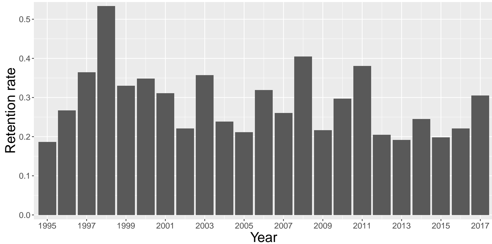
Annual Sturgeon Retention Rate (as \frac{\sum kept}{\sum kept+released} ) by CPFVs fishing in the SF Bay and Delta, 1995-2017
