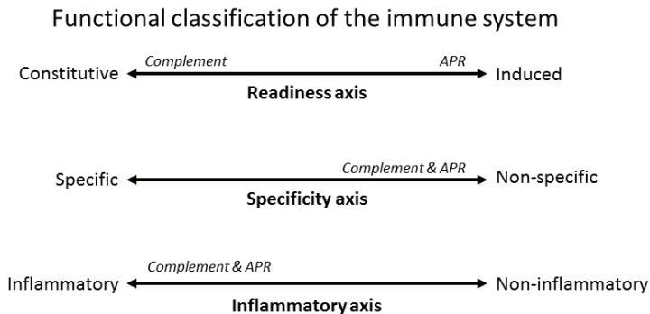
FIGURE 3. —Three functional axes are often used to describe immune responses in ecoimmunology studies: readiness, specificity, and inflammatory. Traditionally, immune responses are partitioned into innate and adaptive responses. No combination of functional axes describes all responses classified as innate or adaptive under the traditional classification; rather, each innate or adaptive response can be described as a combination of these three functional axes. This figure depicts the placement of two innate immune responses, the acute phase response (APR) and complement activity (complement), on the three functional axes.
