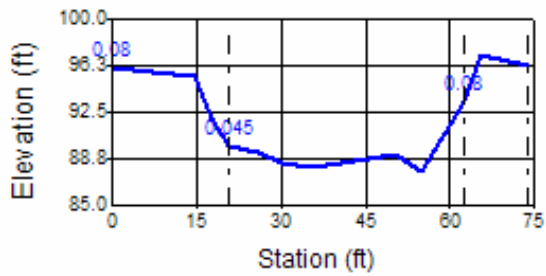
Channel Cross Section
