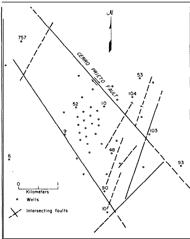
Figure 4: Location of known faults in the vicinity of the Cerro Prieto field, showing the intersecting faults and the location of wells and the very production well No. 103.
