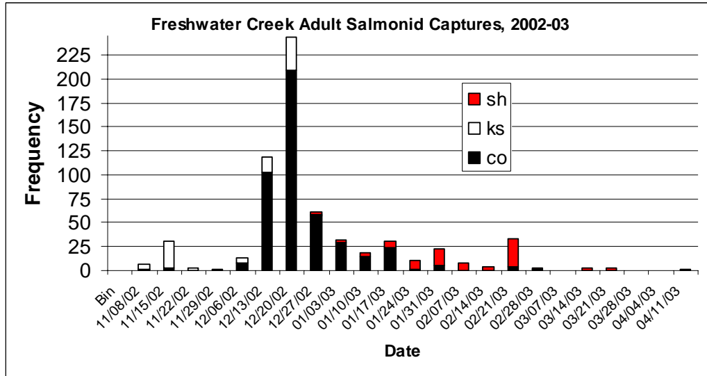
Figure 4. Temporal distribution of all salmonids captured at the Freshwater weir, 2002-2003.
