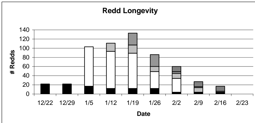
Figure 11. Attrition in visibility of observed redds in Freshwater Creek, 2002-2003. Colored bars depict total new redds observed by date of first observation and during subsequent surveys.
